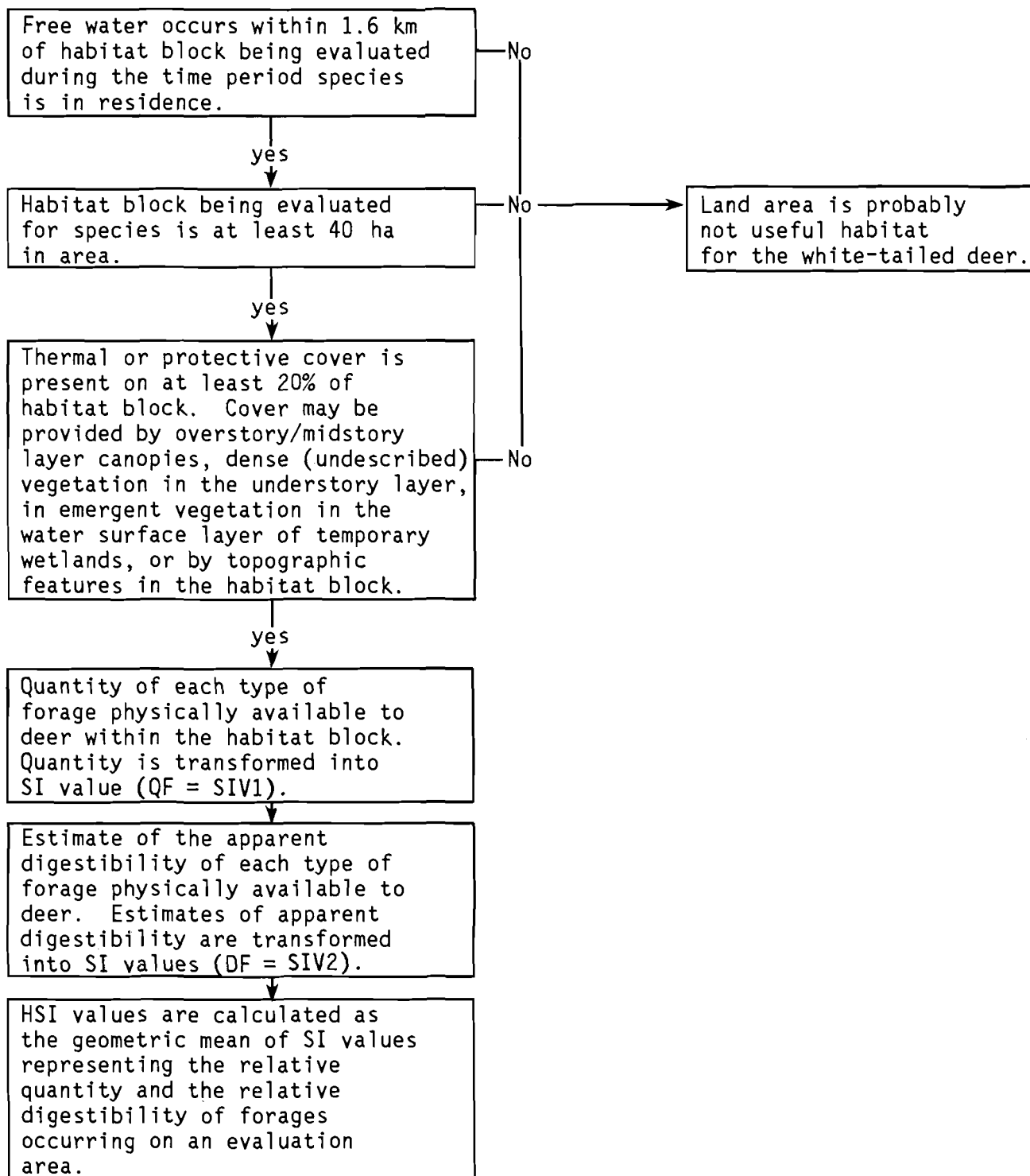
Figure 4. Logic used to develop HSI Model II for white-tailed deer based on SI curves representing the quantity of forage on an evaluation area and the apparent digestibility of those forages.
