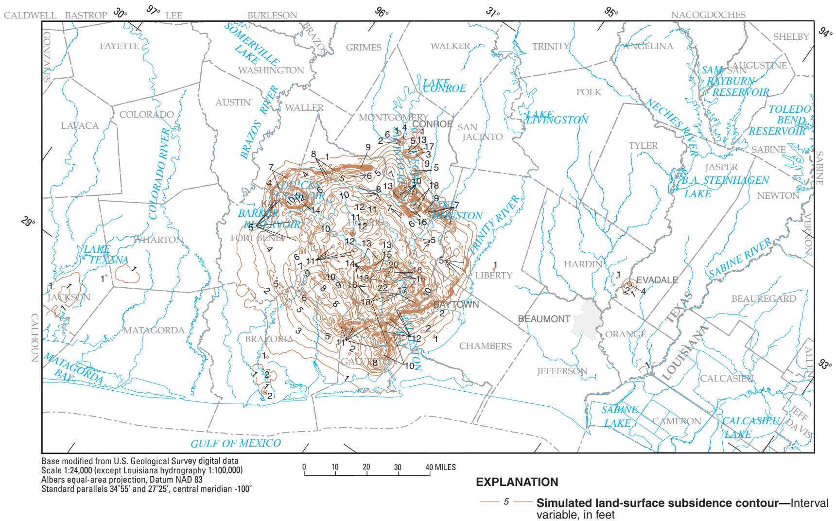
Figure 51. Simulated 2030 land-surface subsidence in the NGC GAM model area resulting from HGCSO withdrawal scenario.
