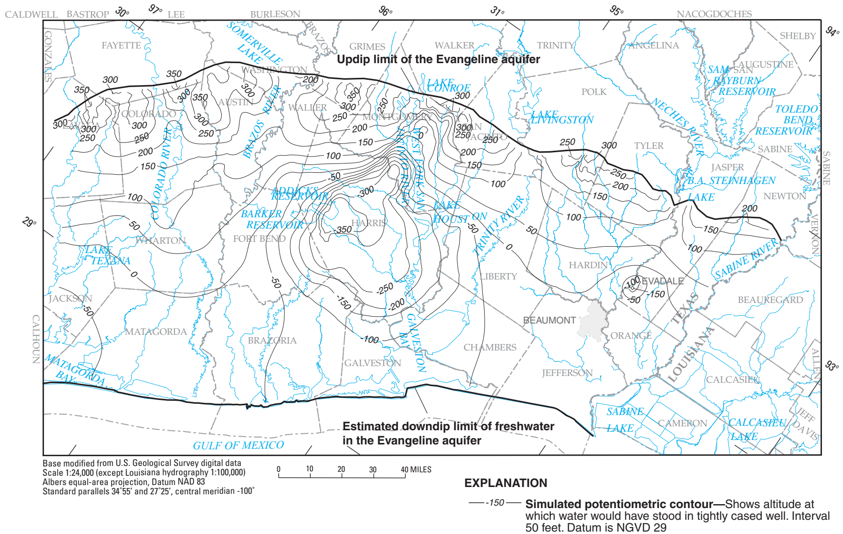
Figure 31. Simulated 2010 potentiometric surface of the Evangeline aquifer in the NGC GAM model area resulting from HGCSO withdrawal scenario.
