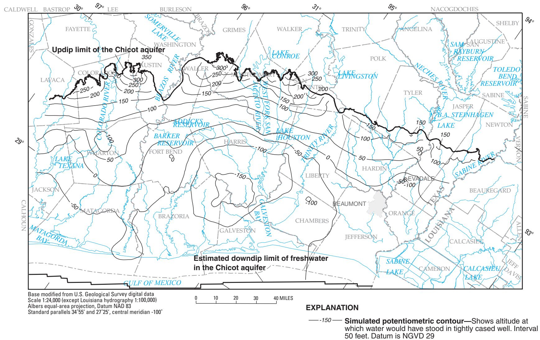
Figure 9. Simulated 2050 potentiometric surface of the Chicot aquifer in the NGC GAM model area resulting from TWDB withdrawal scenario.
