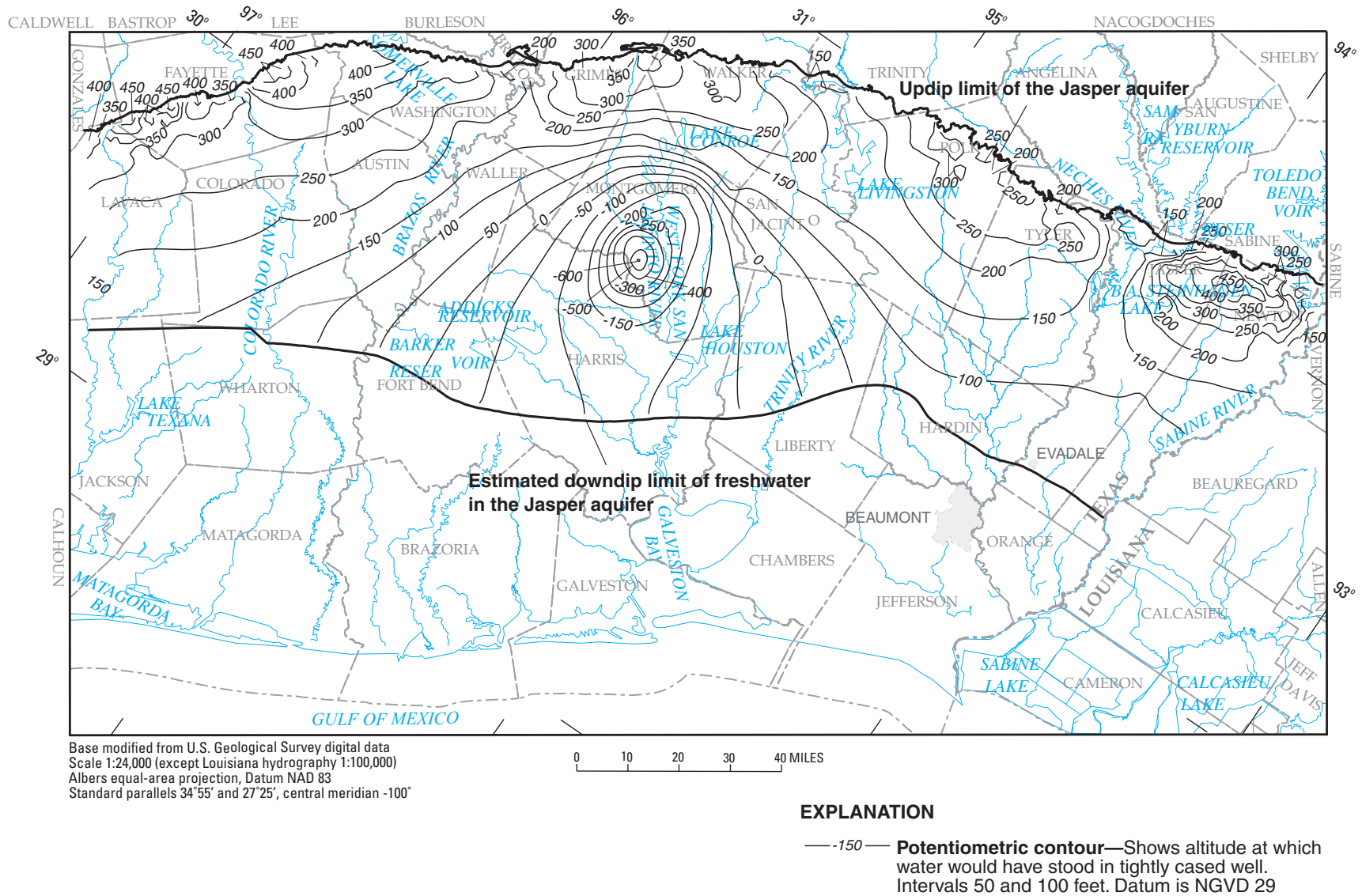
Figure 37. Simulated 2030 potentiometric surface of the Jasper aquifer in the NGC GAM model area resulting from HGCSD withdrawal scenario.
