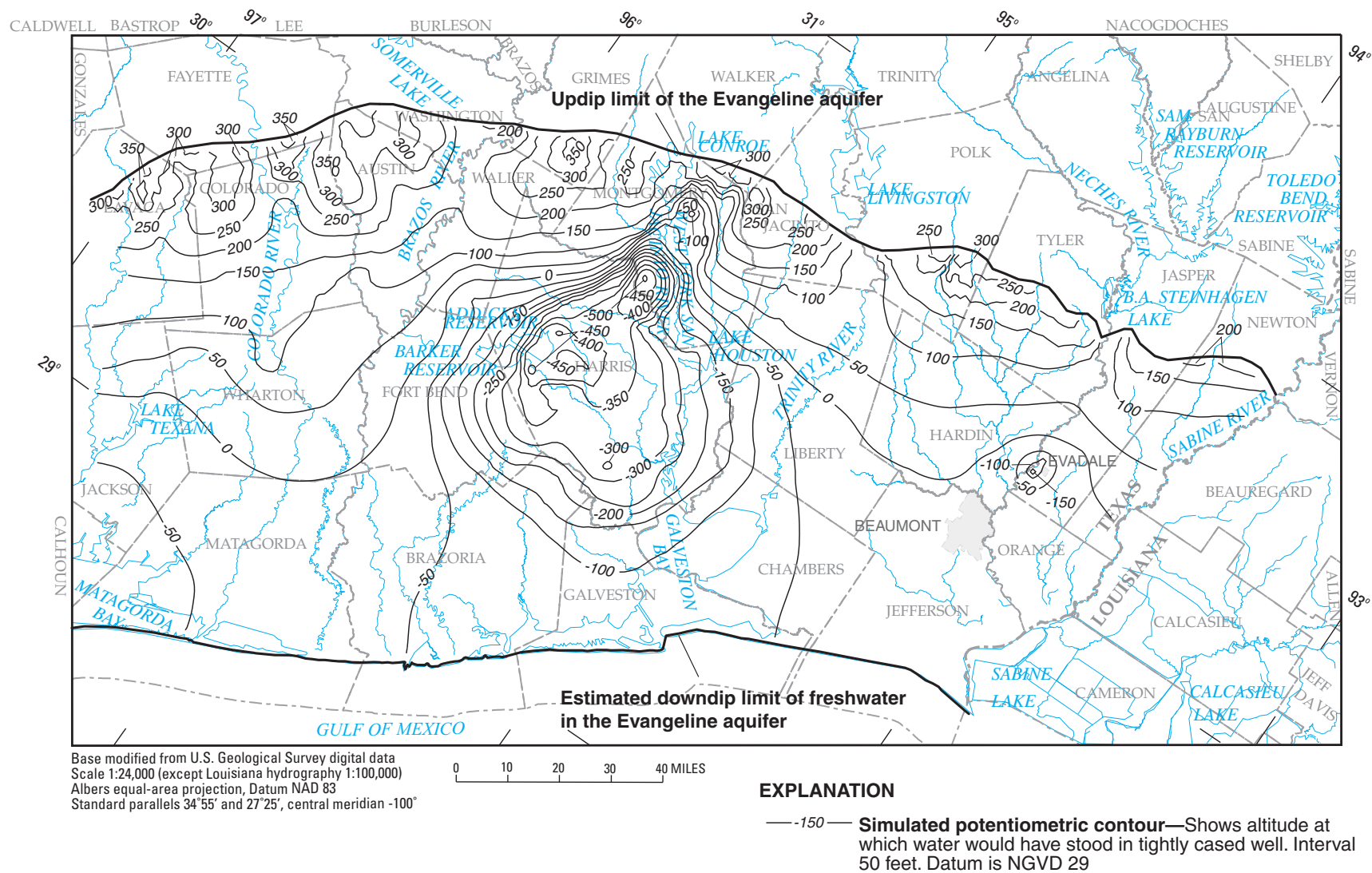
Figure 32. Simulated 2020 potentiometric surface of the Evangeline aquifer in the NGC GAM model area resulting from HGCS withdrawal scenario.
