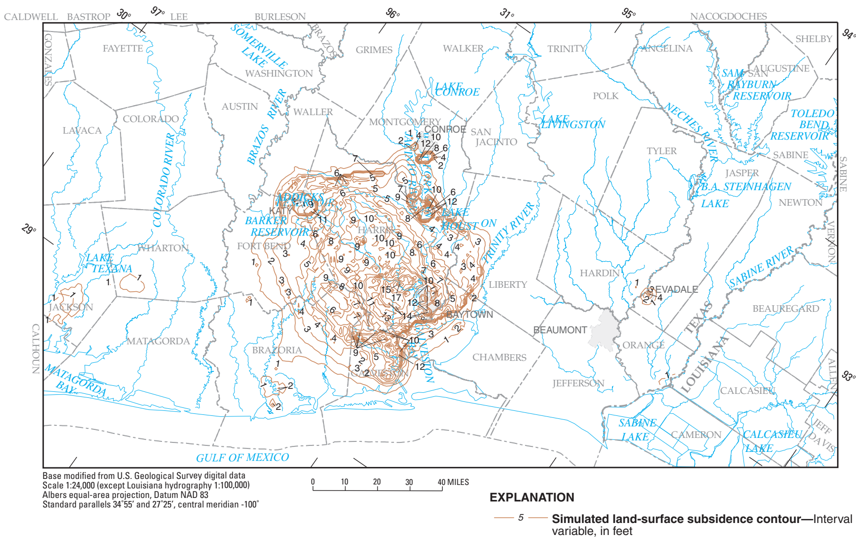
Figure 50. Simulated 2020 land-surface subsidence in the NGC GAM model area resulting from HGCSO withdrawal scenario.
