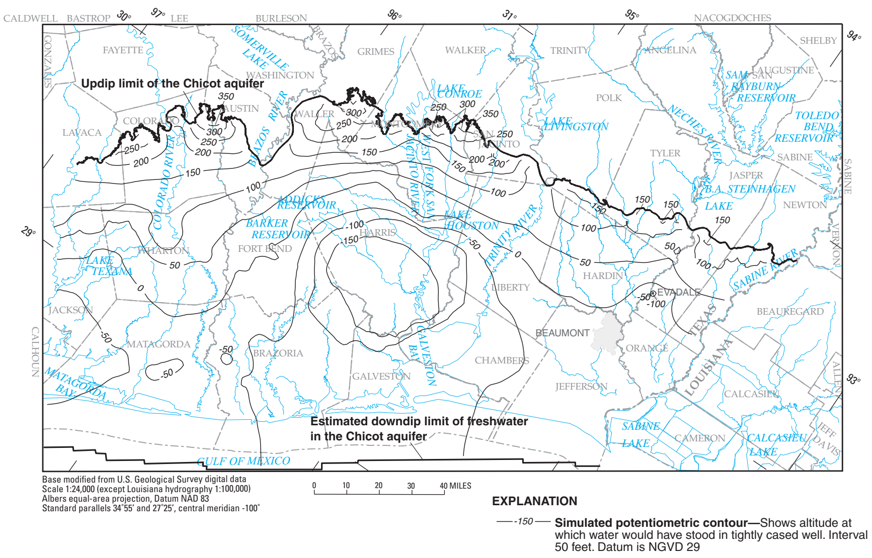
Figure 5. Simulated 2010 potentiometric surface of the Chicot aquifer in the NGC GAM model area resulting from TWDB withdrawal scenario.
