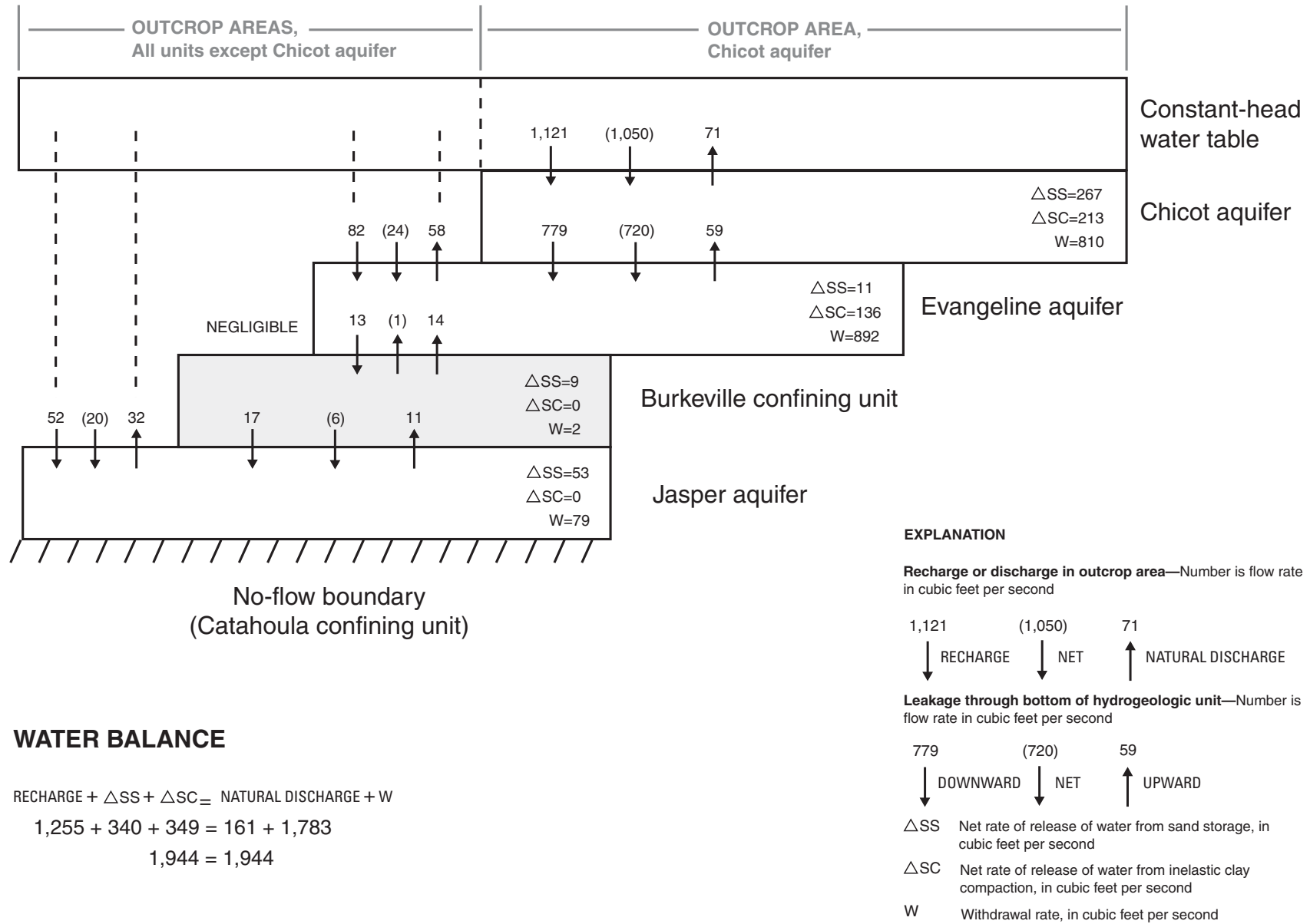
Figure 39. Simulated 2010 water-budget components of the hydrogeologic units of the NGC GAM model resulting from HGCSO withdrawal scenario.
