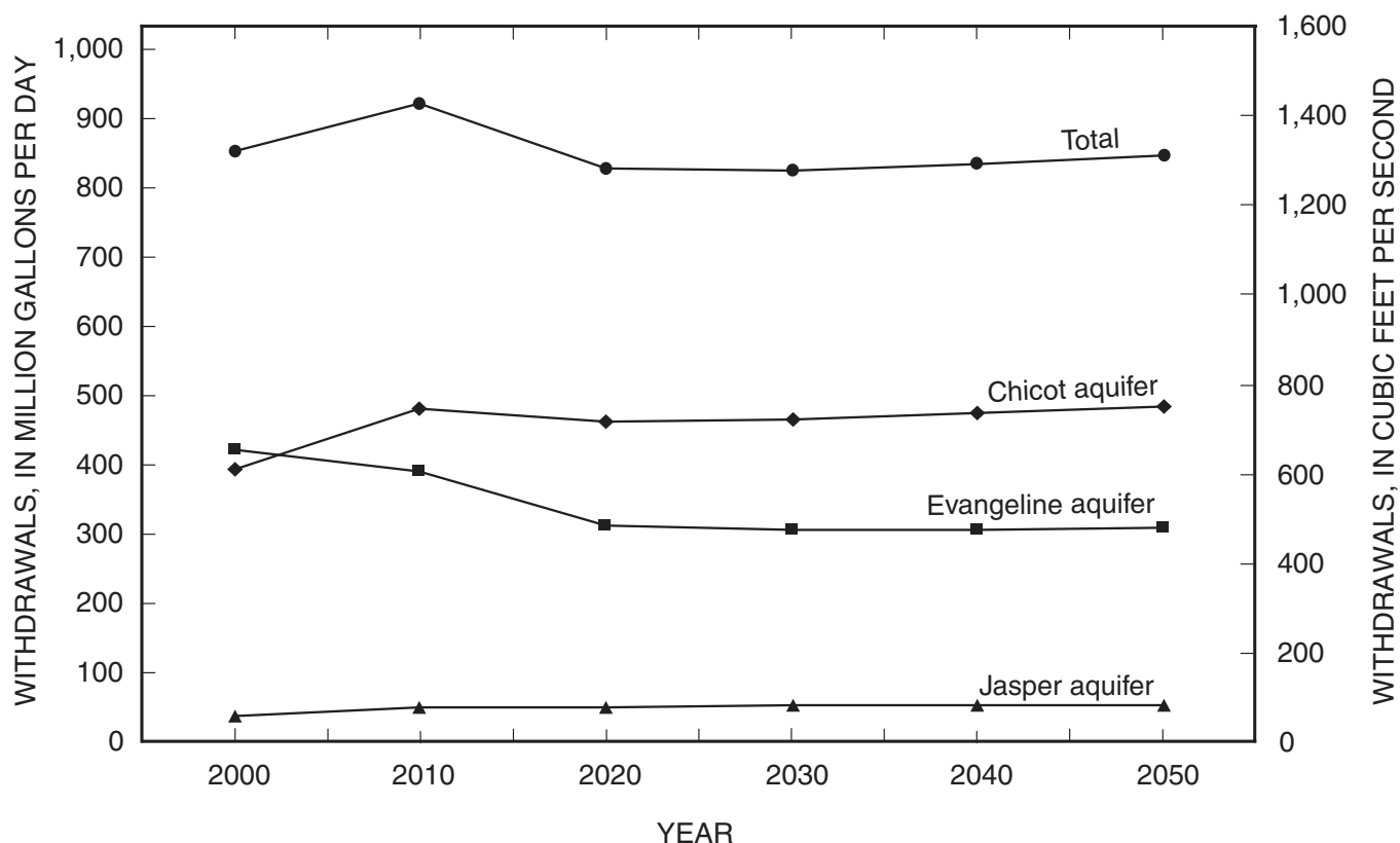
Figure 2. Withdrawals in the Chicot, Evangeline, and Jasper aquifers in the NGC GAM model area from 2000 to 2050, TWDB withdrawal scenario.
