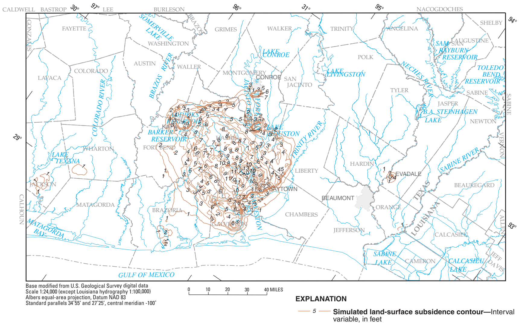
Figure 49. Simulated 2010 land-surface subsidence in the NGC GAM model area resulting from HGCS withdrawal scenario.
