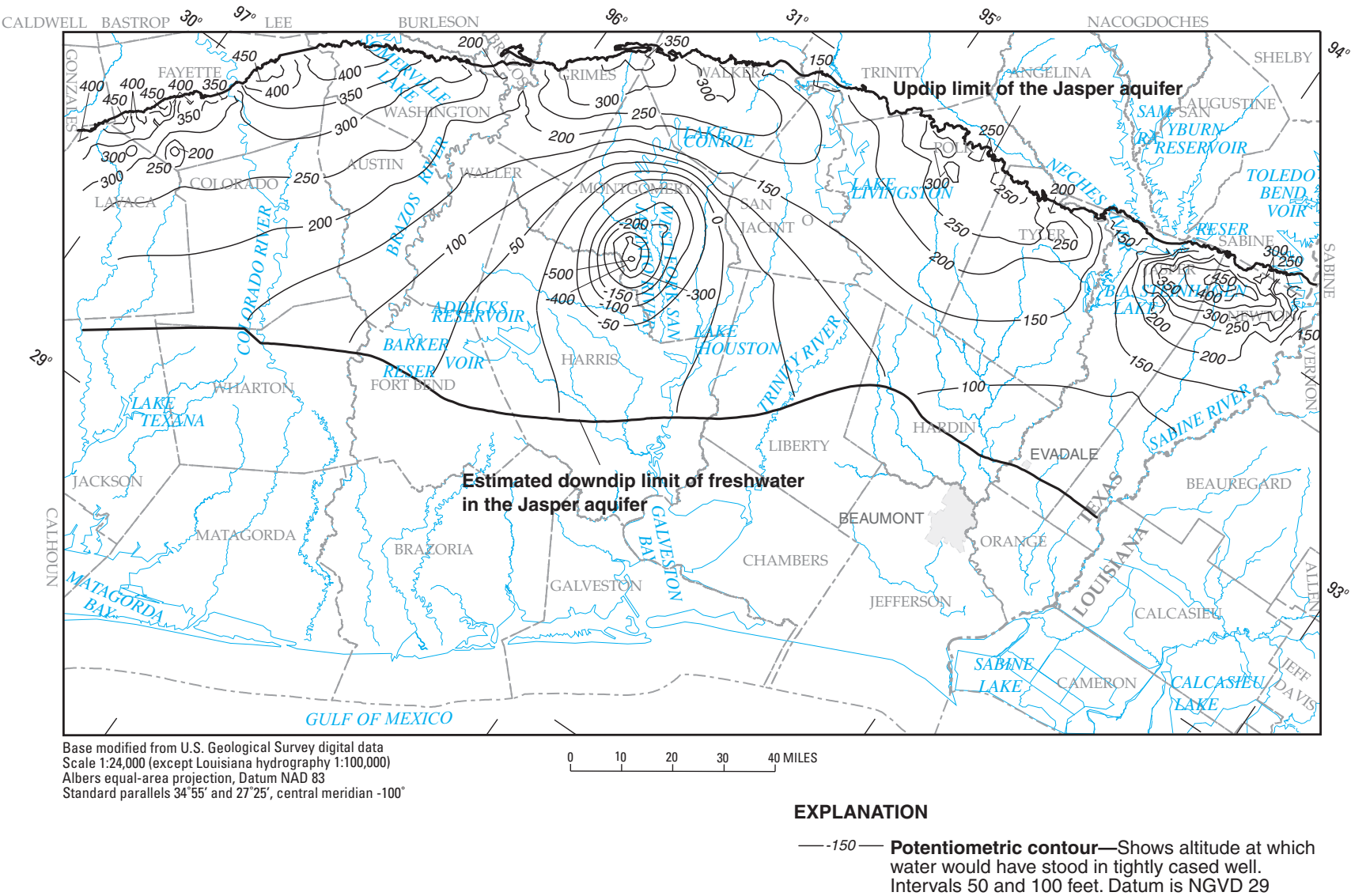
Figure 35. Simulated 2010 potentiometric surface of the Jasper aquifer in the NGC GAM model area resulting from HGCSD withdrawal scenario.
