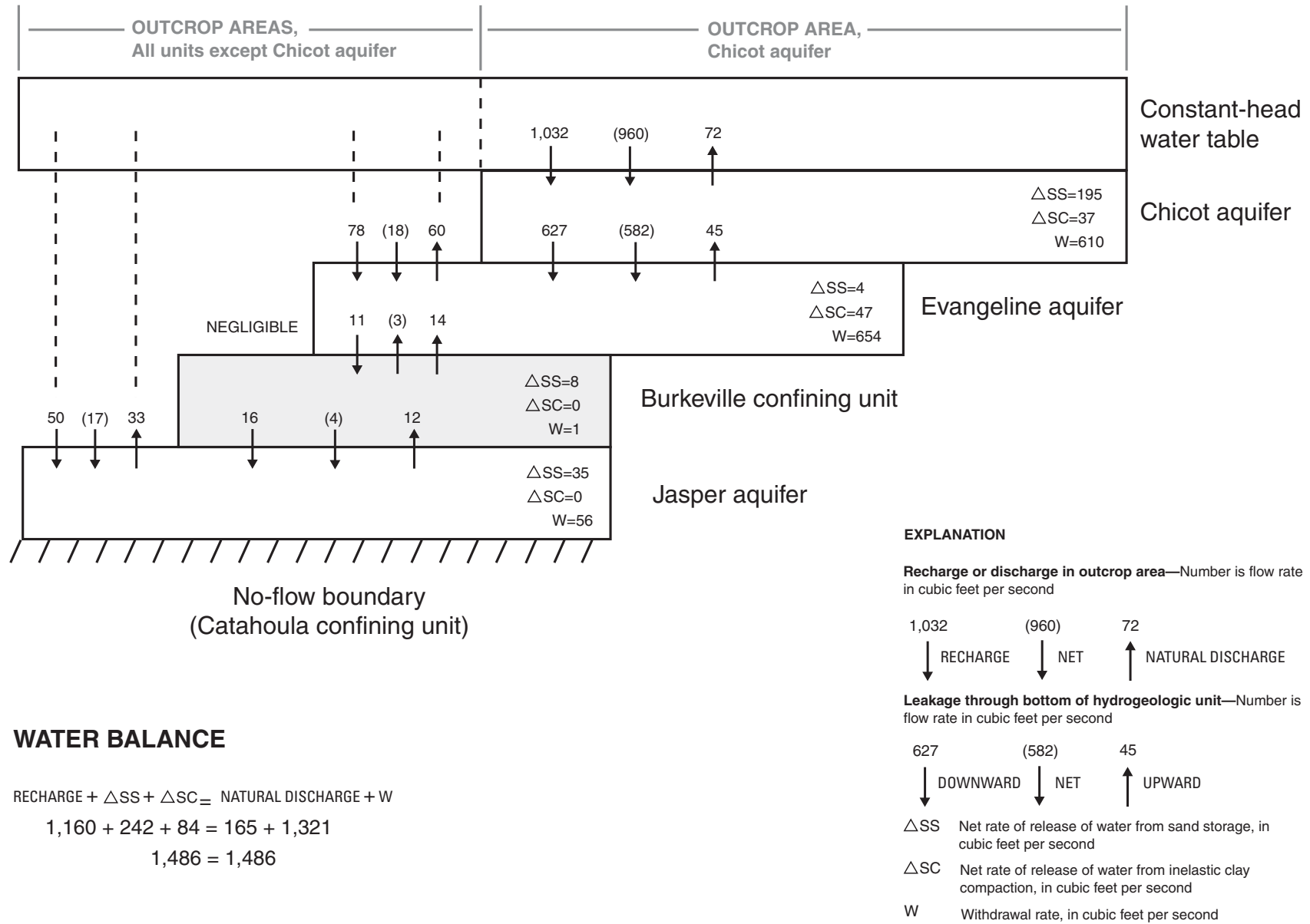
Figure 22. Simulated 2000 water-budget components of the hydrogeologic units of the NGC GAM model resulting from TWDB withdrawal scenario.
