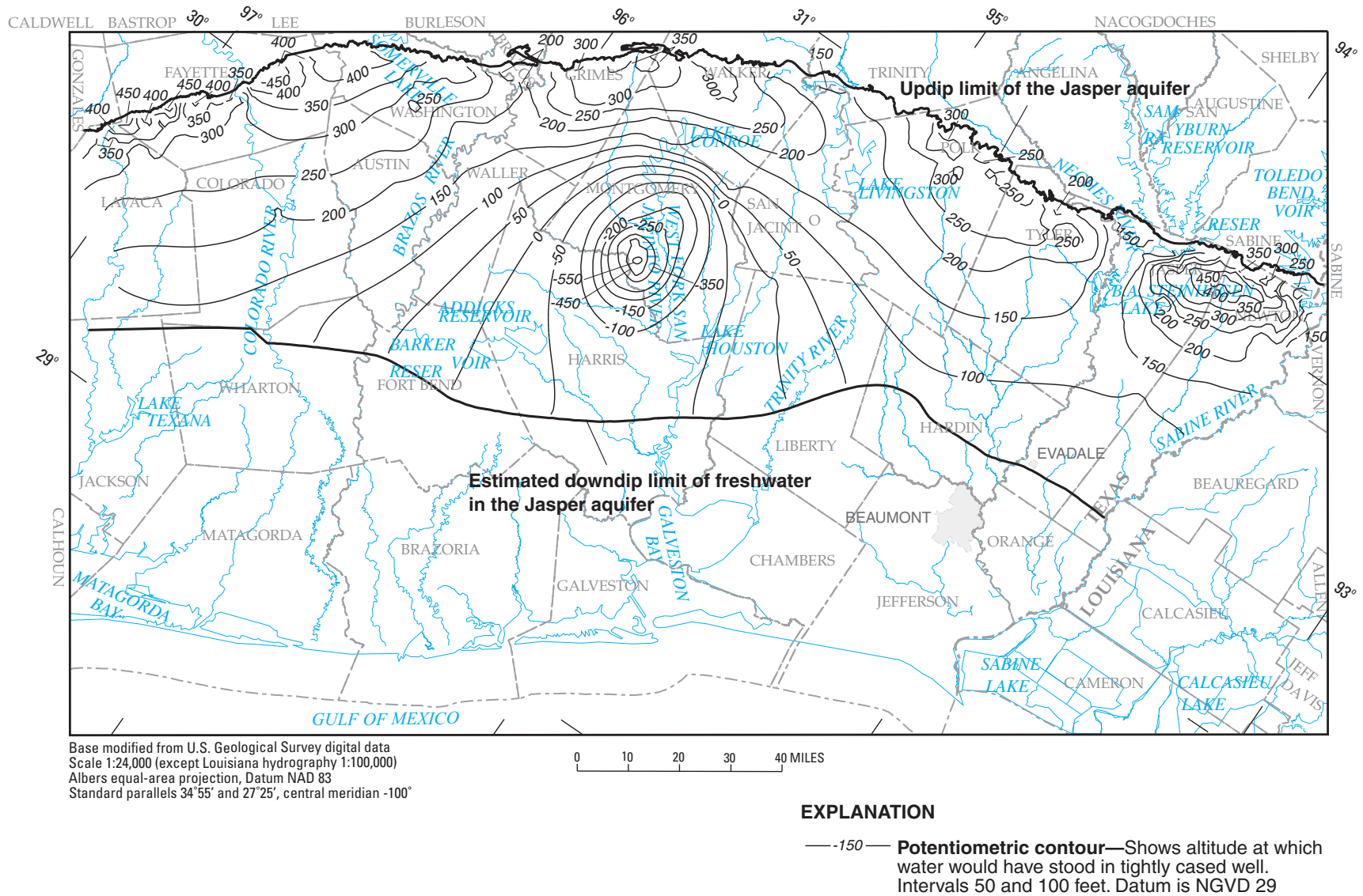
Figure 20. Simulated 2040 potentiometric surface of the Jasper aquifer in the NGC GAM model area resulting from TWDB withdrawal scenario.
