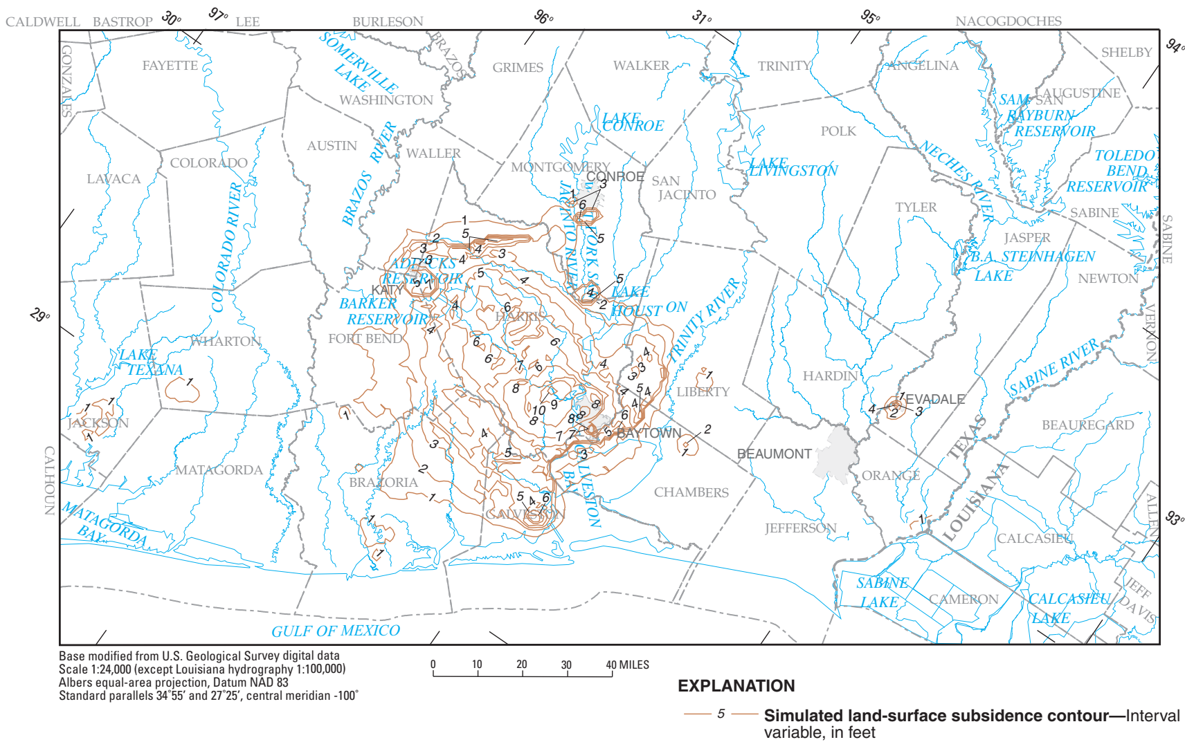
Figure 43. Simulated 2010 land-surface subsidence in the NGC GAM model area resulting from TWDB withdrawal scenario.
