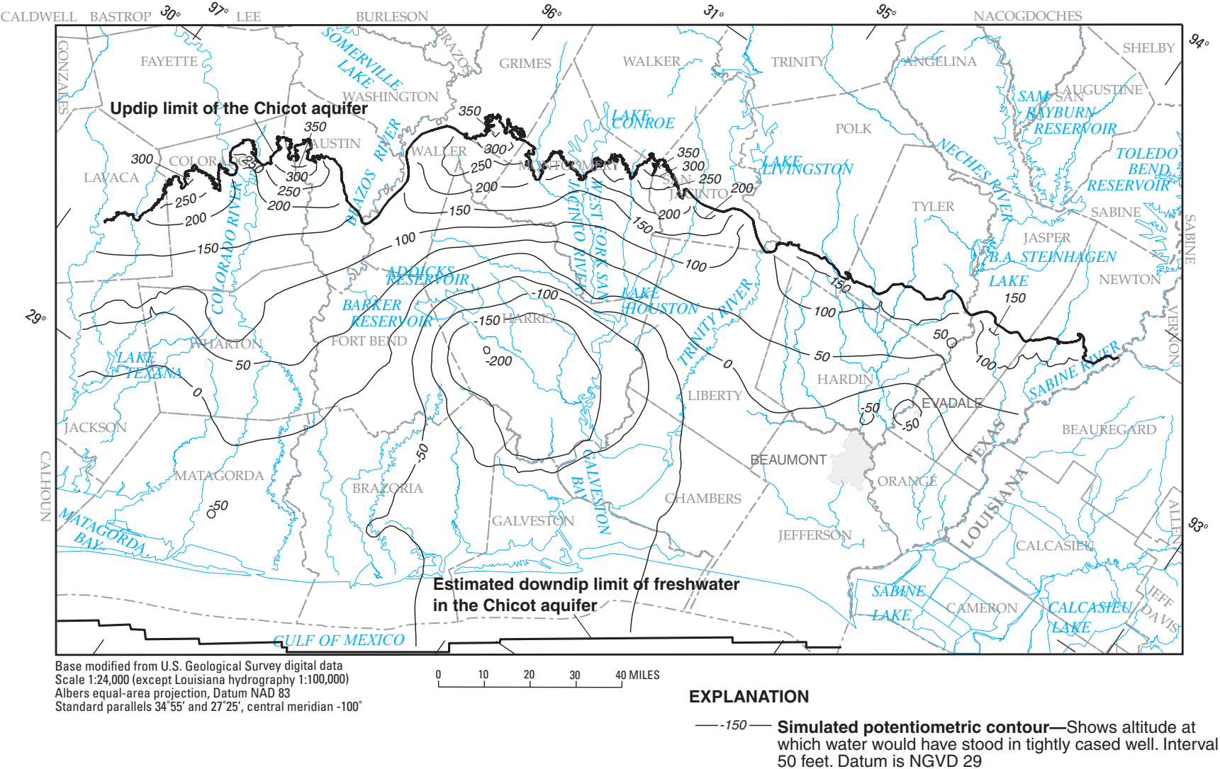
Figure 26. Simulated 1995 potentiometric surface of the Chicot aquifer in the NGC GAM model area resulting from HGCSO withdrawal scenario.
