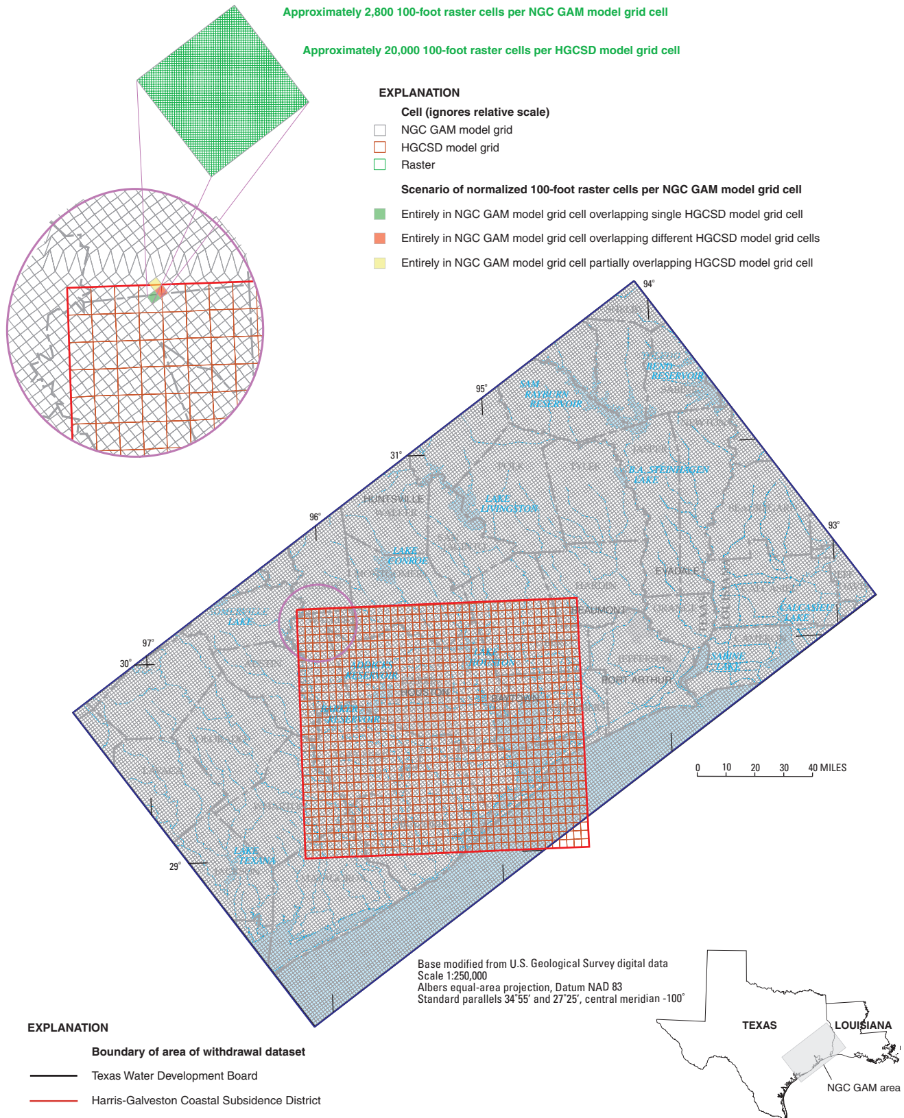
Figure a2.1. Relations between NGC GAM model grid cells, HGCSO model grid cells, and raster cells associated with merge of HGCSO dataset into TWDB dataset.
