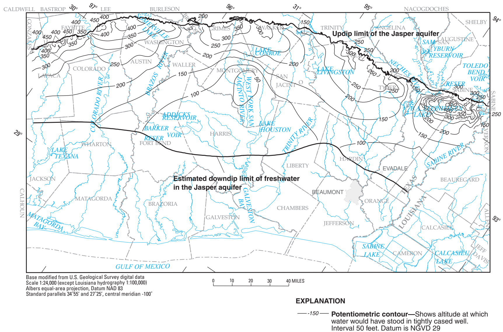
Figure 16. Simulated 2000 potentiometric surface of the Jasper aquifer in the NGC GAM model area resulting from TWDB withdrawal scenario.
