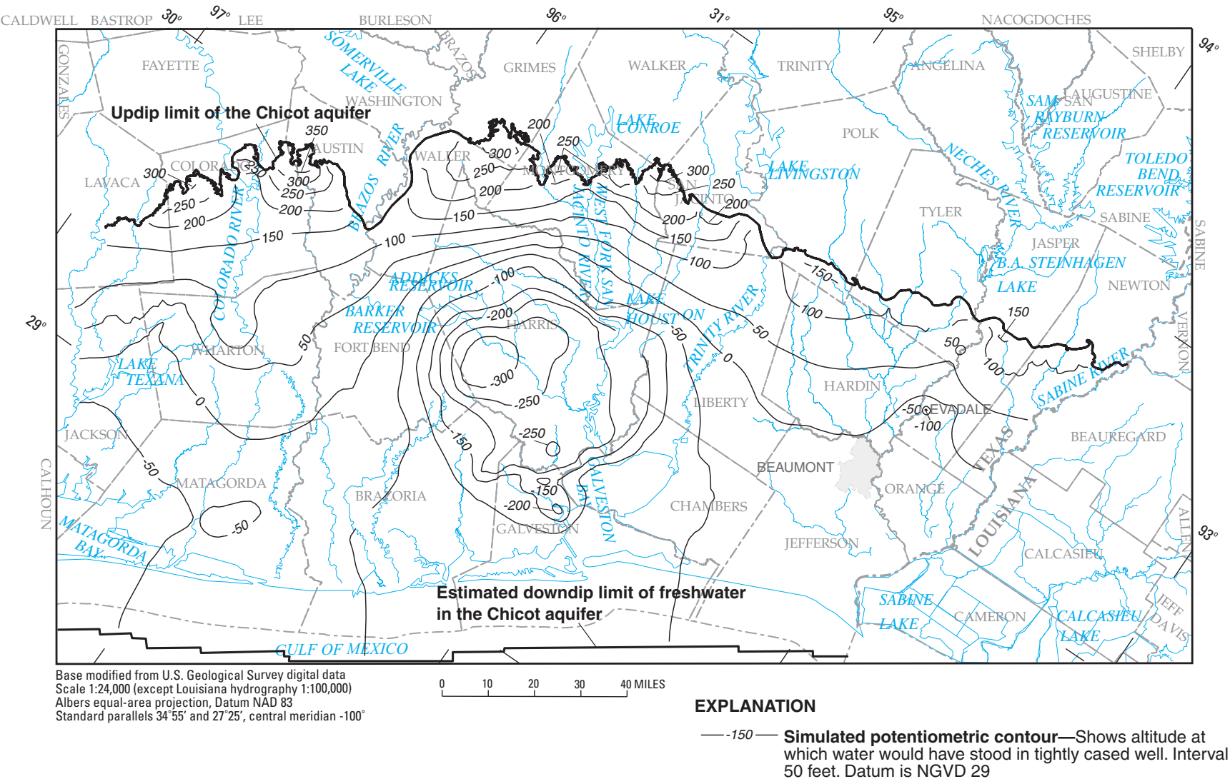
Figure 28. Simulated 2020 potentiometric surface of the Chicot aquifer in the NGC GAM model area resulting from HGCSO withdrawal scenario.
