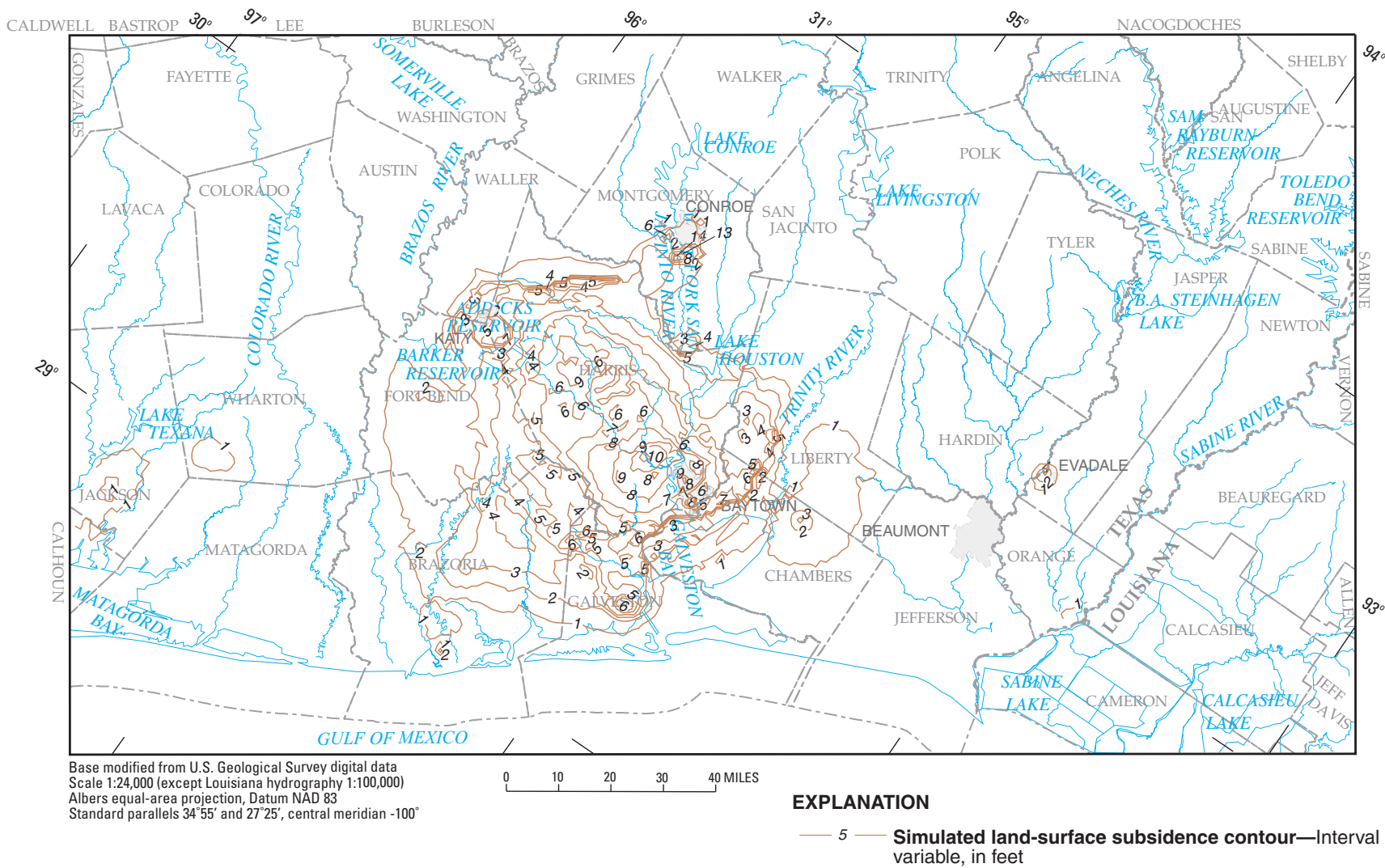
Figure 47. Simulated 2050 land-surface subsidence in the NGC GAM model area resulting from TWDB withdrawal scenario.
