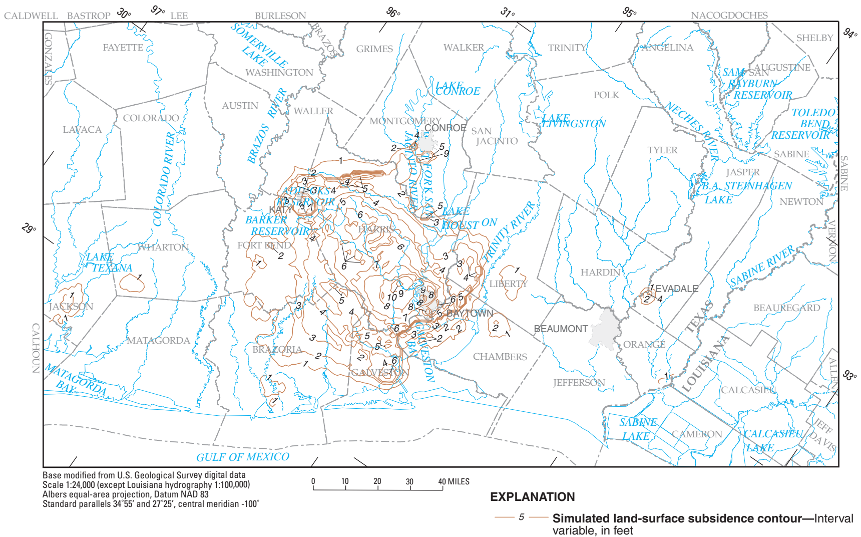
Figure 44. Simulated 2020 land-surface subsidence in the NGC GAM model area resulting from TWDB withdrawal scenario.
