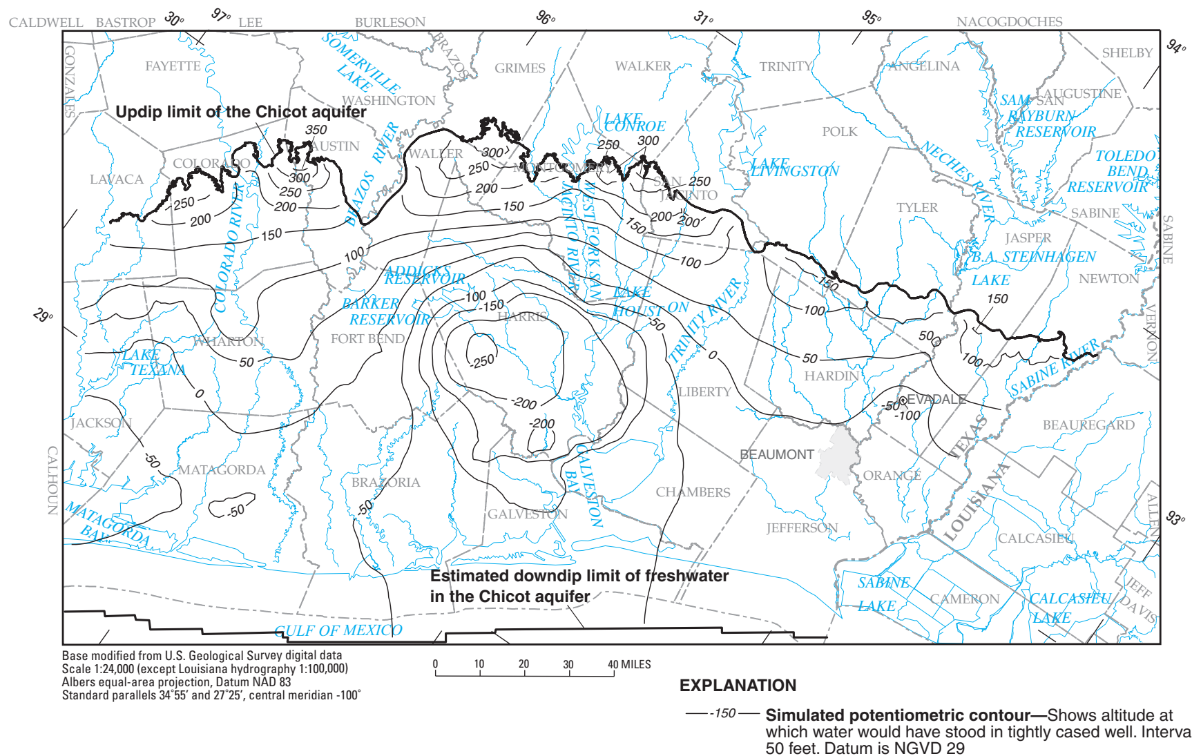
Figure 27. Simulated 2010 potentiometric surface of the Chicot aquifer in the NGC GAM model area resulting from HGCSO withdrawal scenario.
