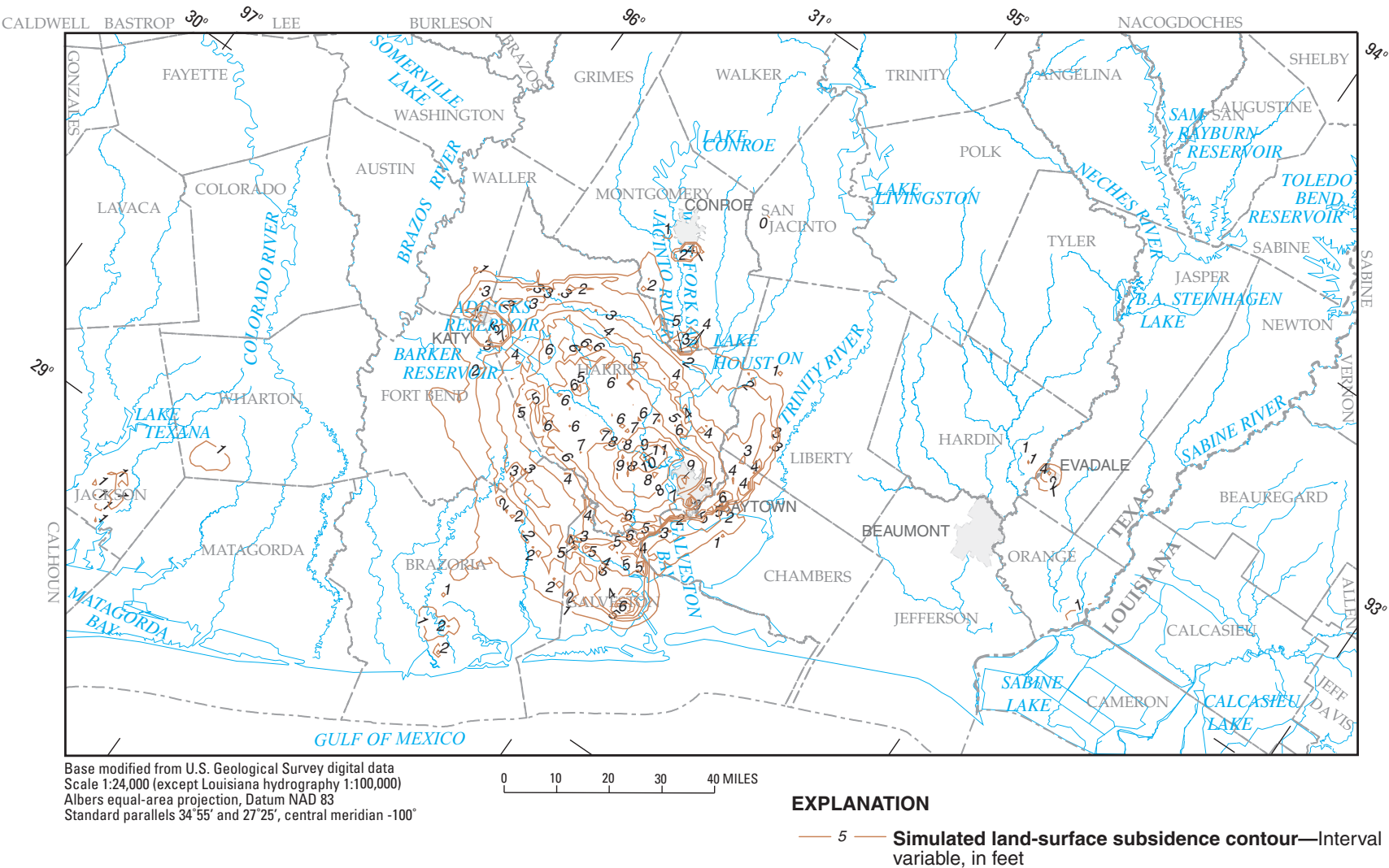
Figure 48. Simulated 1995 land-surface subsidence in the NGC GAM model area resulting from HGCSO withdrawal scenario.
