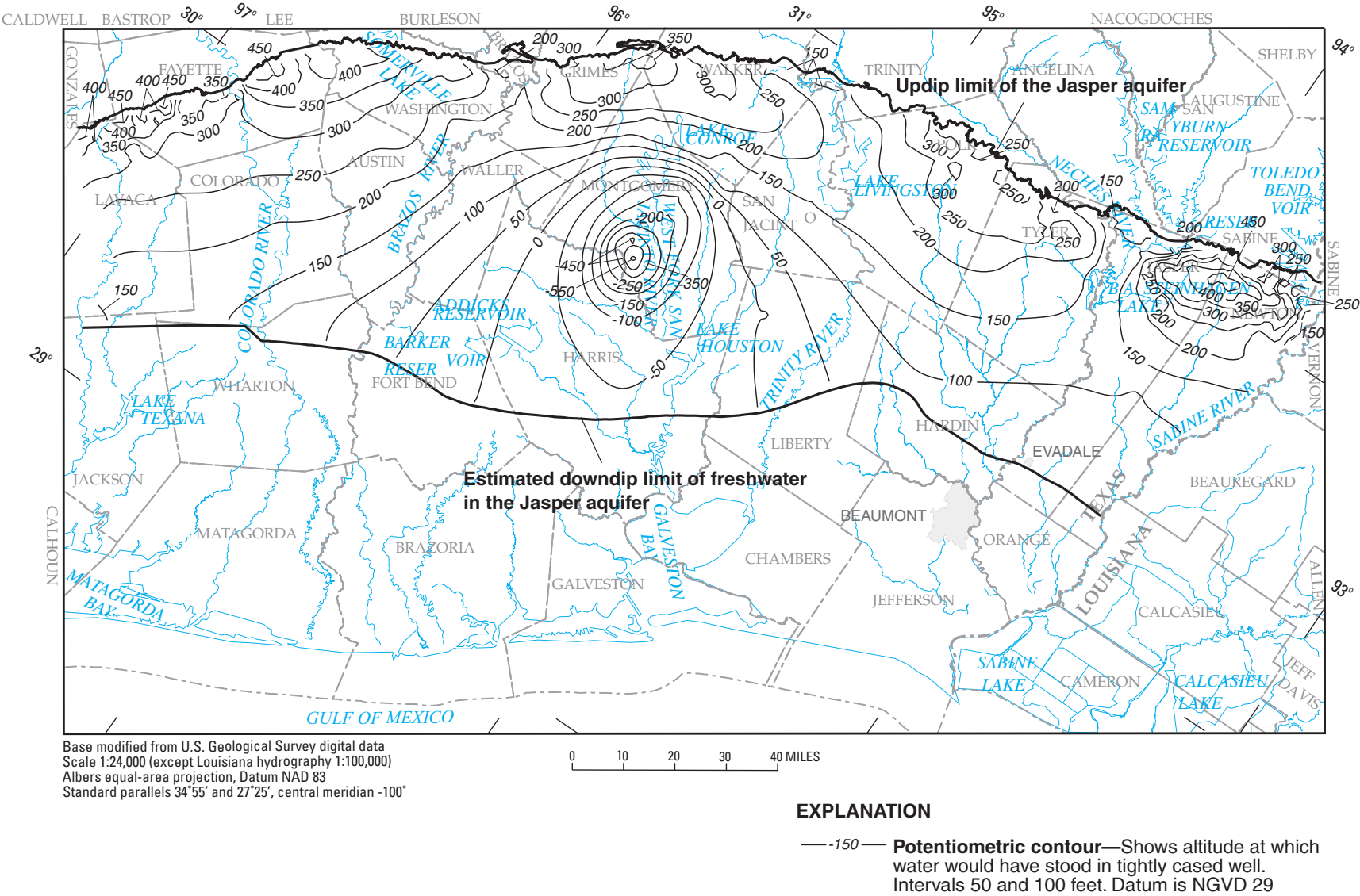
Figure 18. Simulated 2020 potentiometric surface of the Jasper aquifer in the NGC GAM model area resulting from TWDB withdrawal scenario.
