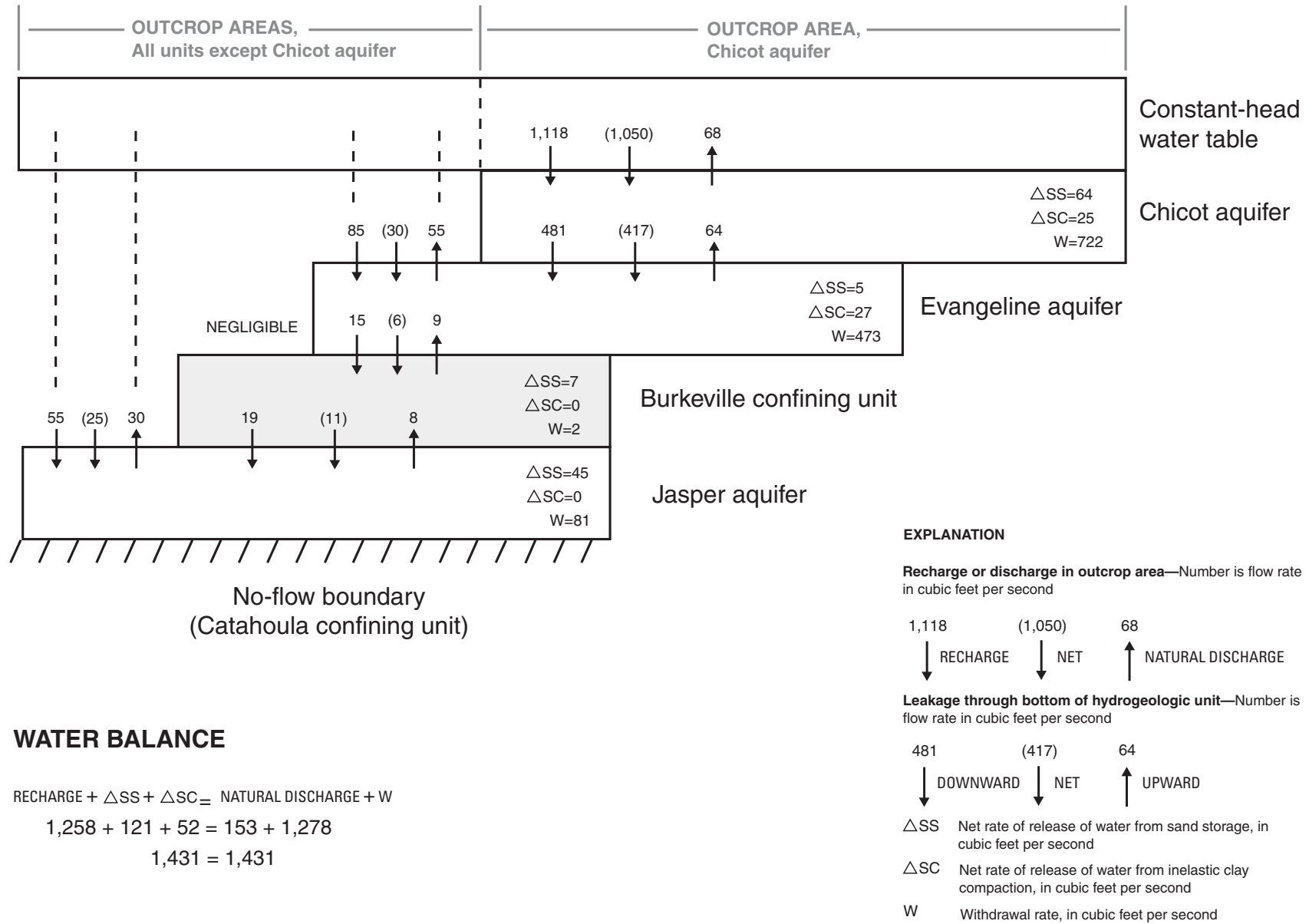
Figure 24. Simulated 2030 water-budget components of the hydrogeologic units of the NGC GAM model resulting from TWDB withdrawal scenario.
