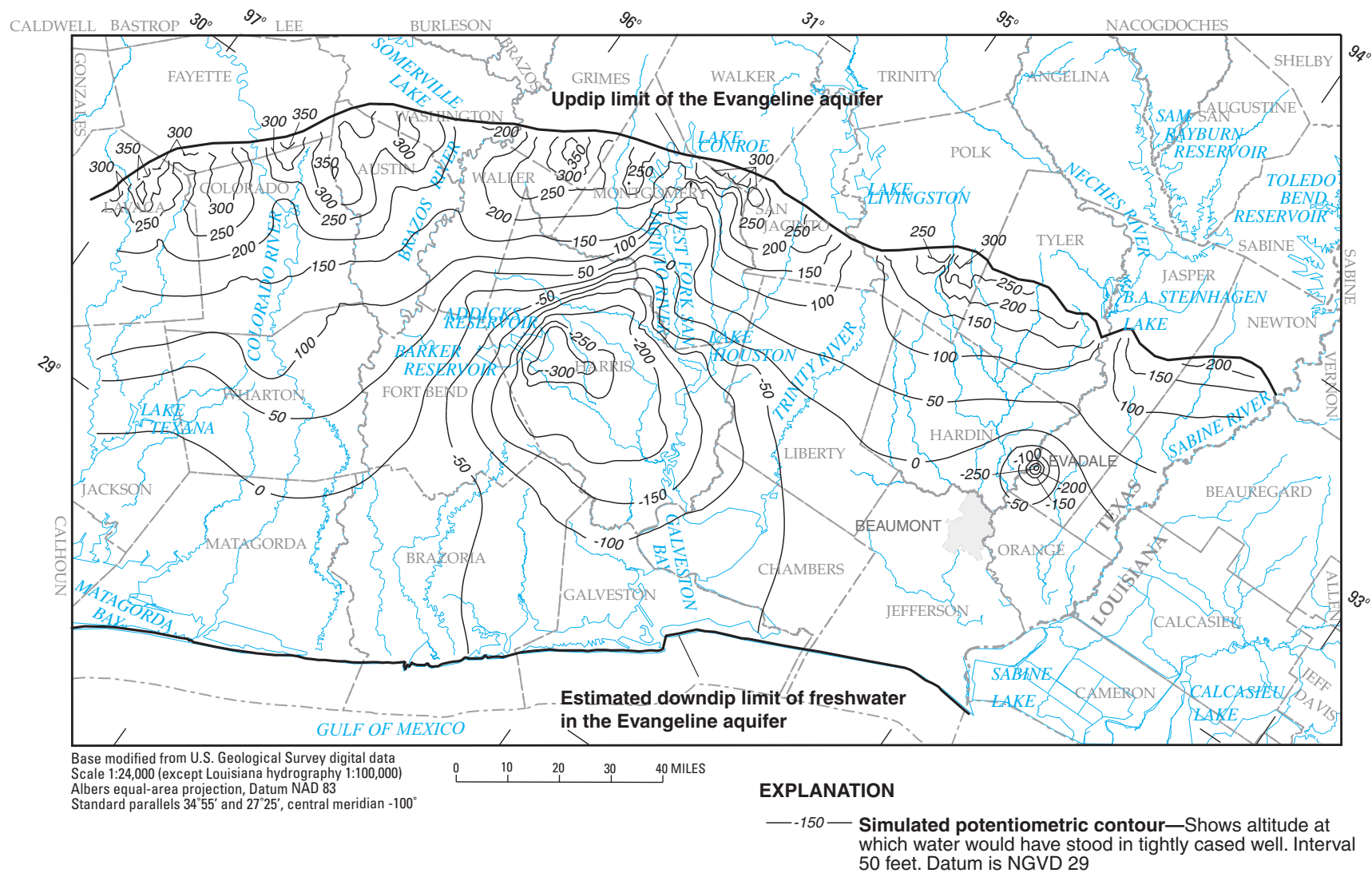
Figure 30. Simulated 1995 potentiometric surface of the Evangeline aquifer in the NGC GAM model area resulting from HGCSO withdrawal scenario.
