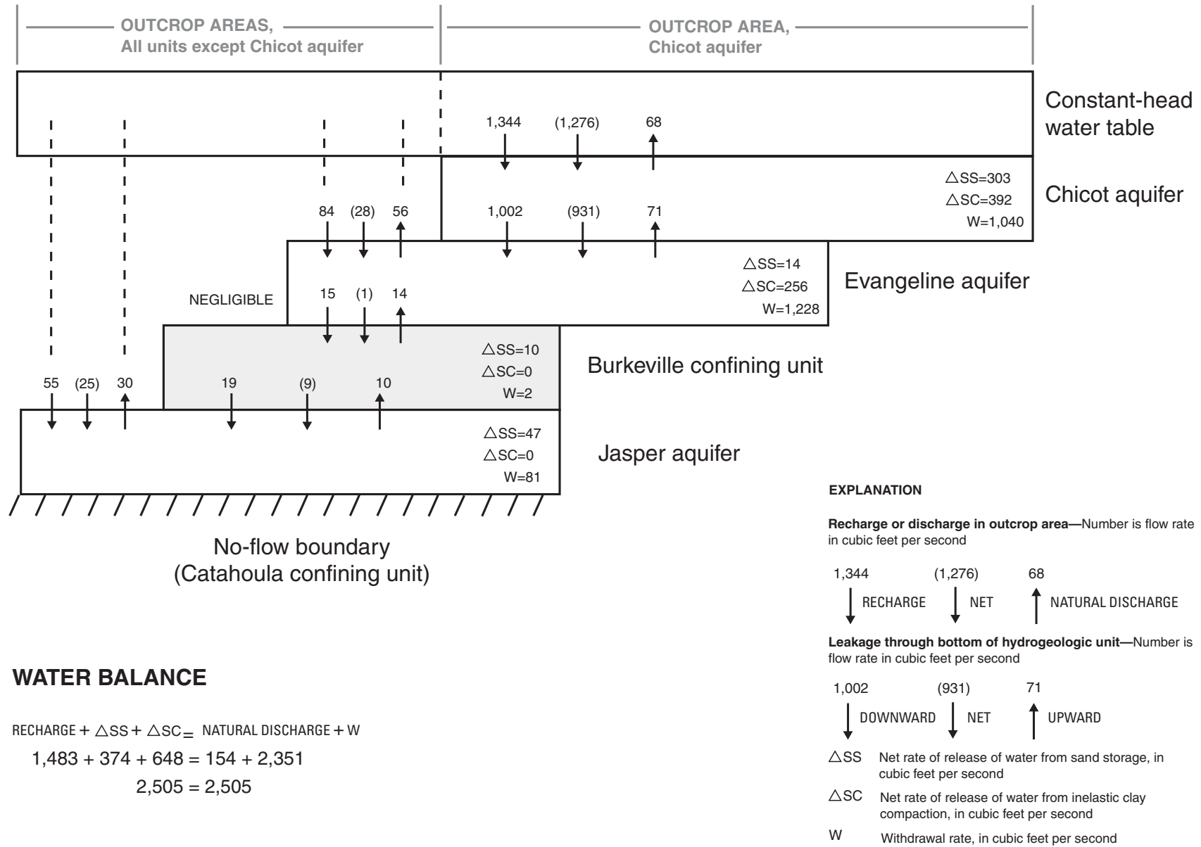
Figure 41. Simulated 2030 water-budget components of the hydrogeologic units of the NGC GAM model resulting from HGCSD withdrawal scenario.
