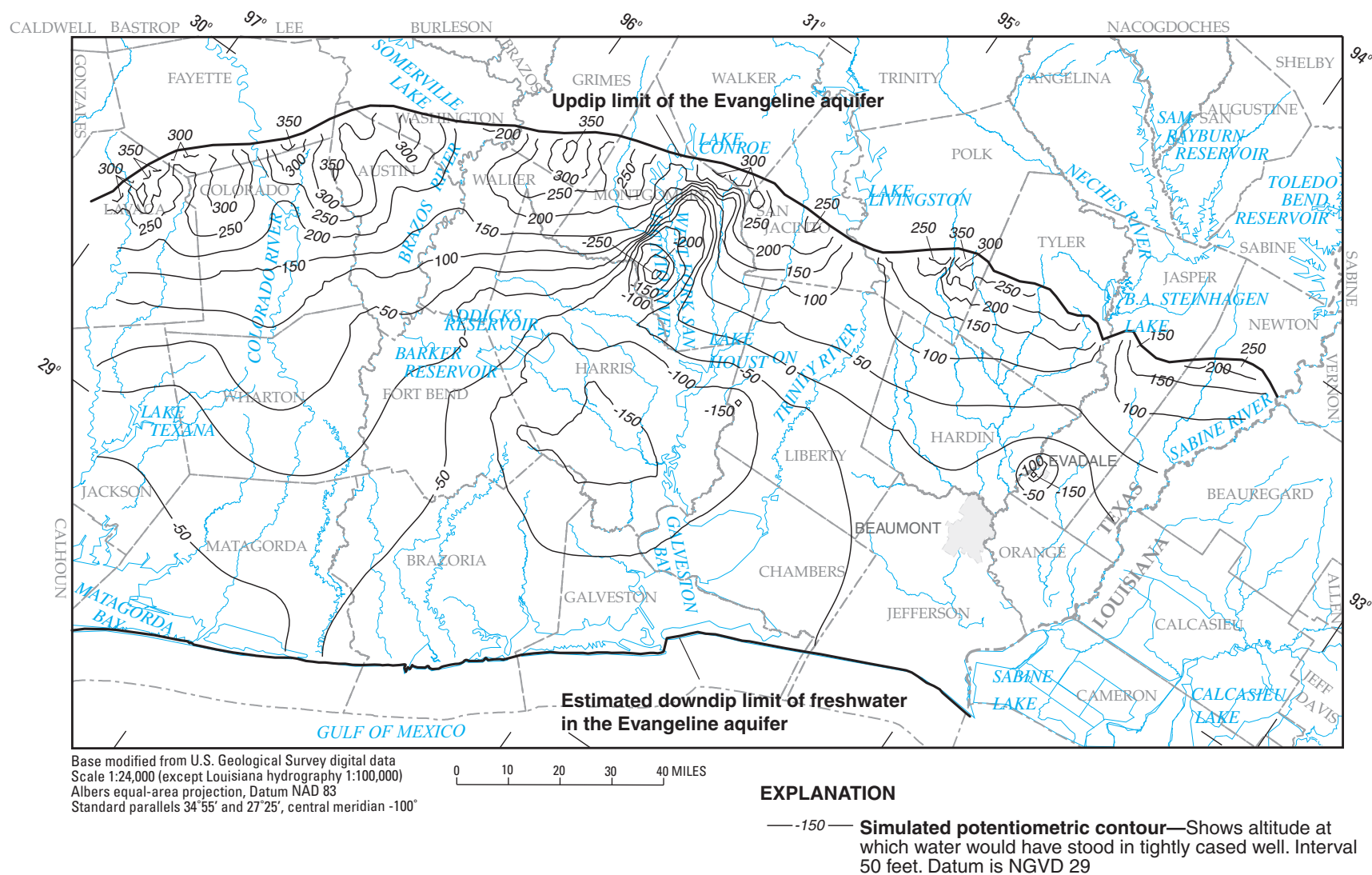
Figure 14. Simulated 2040 potentiometric surface of the Evangeline aquifer in the NGC GAM model area resulting from TWDB withdrawal scenario.
