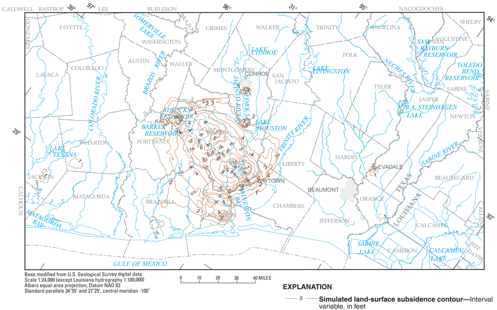
Figure 42. Simulated 2000 land-surface subsidence in the NGC GAM model area resulting from TWDB withdrawal scenario.
