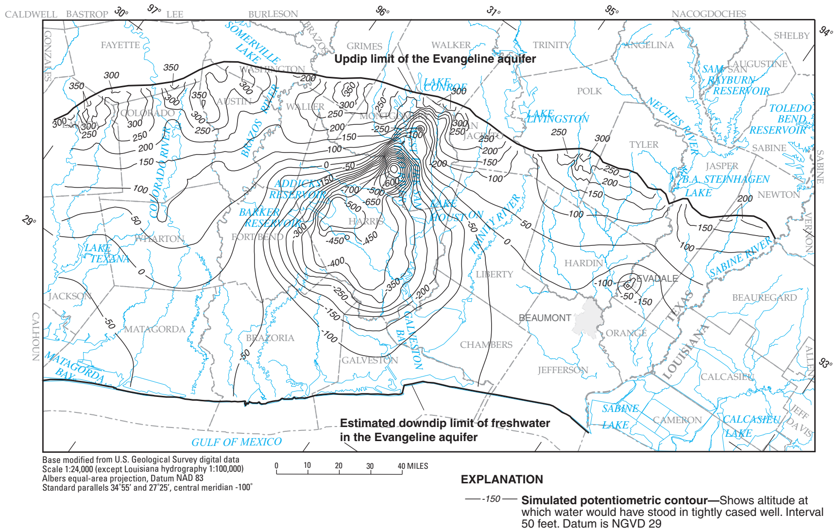
Figure 33. Simulated 2030 potentiometric surface of the Evangeline aquifer in the NGC GAM model area resulting from HGCSO withdrawal scenario.
