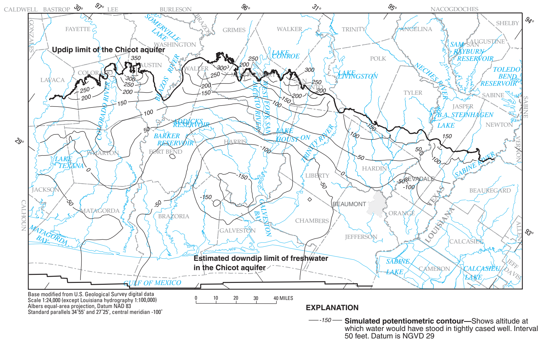
Figure 7. Simulated 2030 potentiometric surface of the Chicot aquifer in the NGC GAM model area resulting from TWDB withdrawal scenario.
