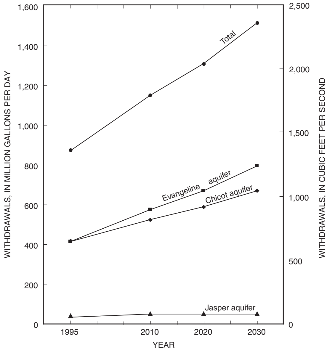
Figure 3. Withdrawals in the Chicot, Evangeline, and Jasper aquifers in the NGC GAM model area from 1995 to 2030, HGCSO withdrawal scenario.
