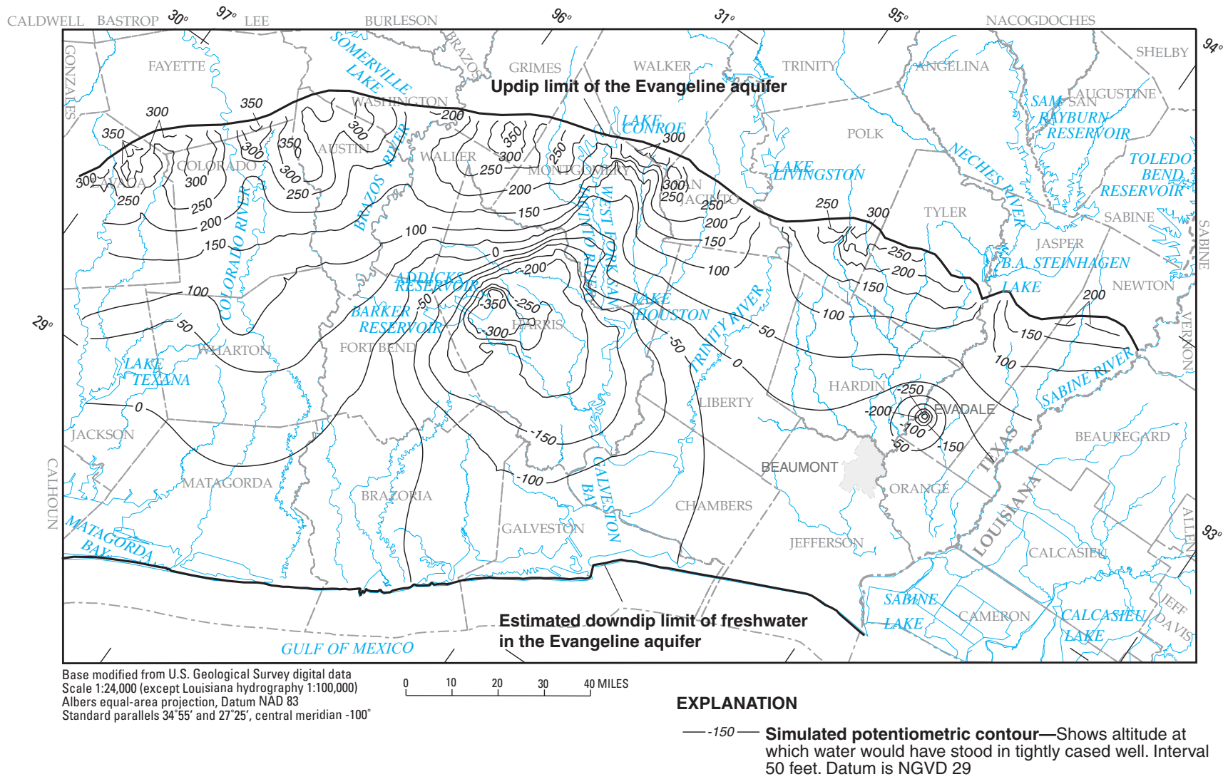
Figure 10. Simulated 2000 potentiometric surface of the Evangeline aquifer in the NGC GAM model area resulting from TWDB withdrawal scenario.
