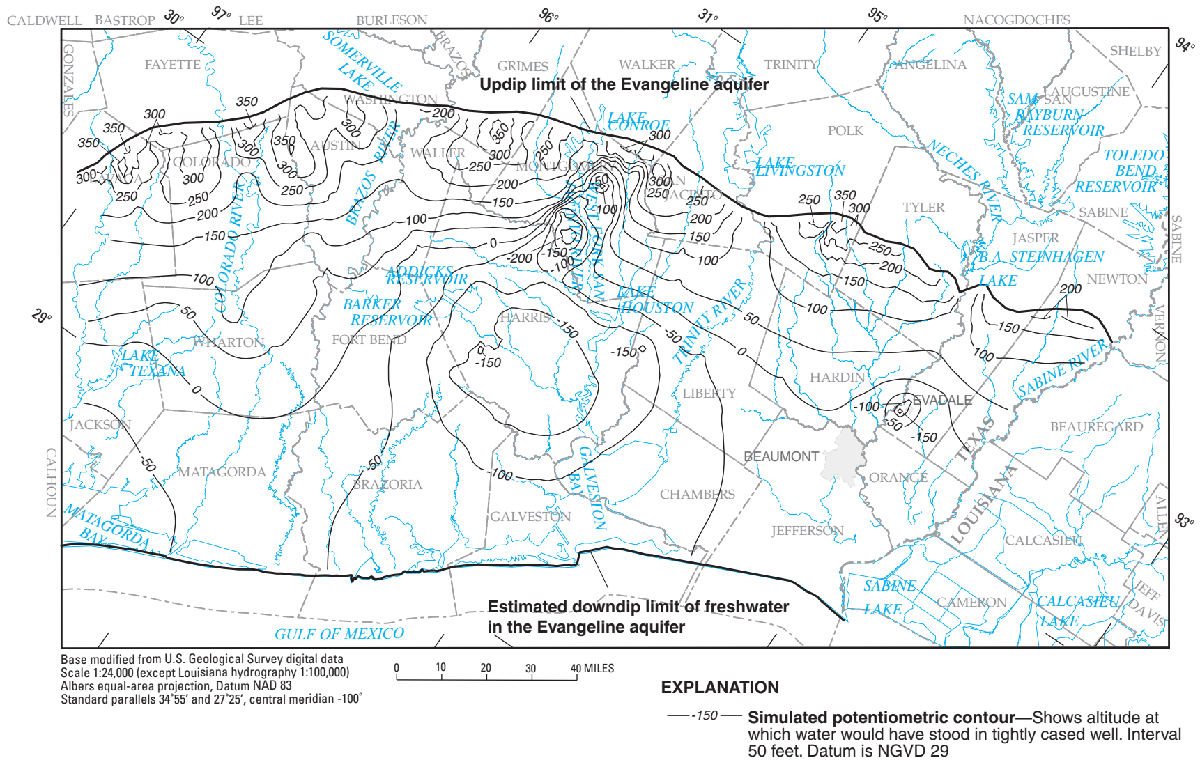
Figure 12. Simulated 2020 potentiometric surface of the Evangeline aquifer in the NGC GAM model area resulting from TWDB withdrawal scenario.
