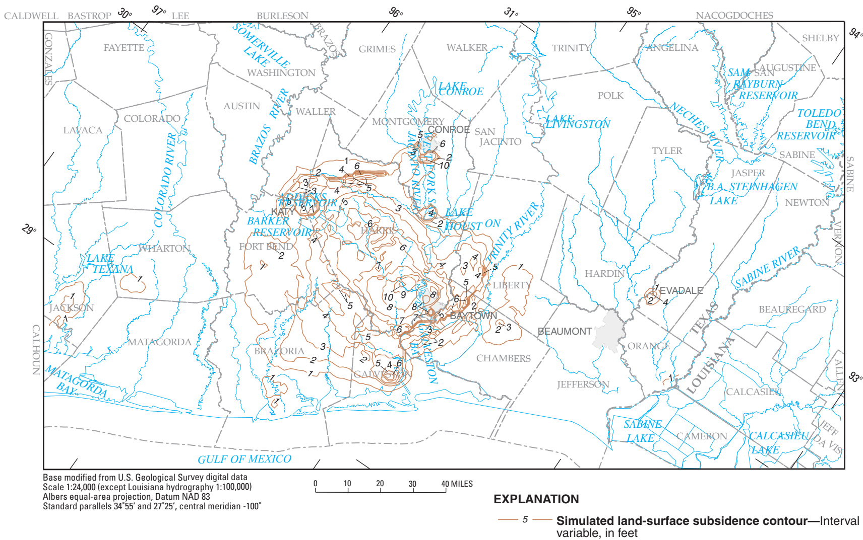
Figure 45. Simulated 2030 land-surface subsidence in the NGC GAM model area resulting from TWDB withdrawal scenario.
