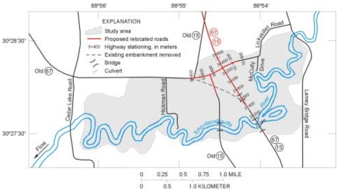
Figure 4. Proposed principal roads in the study area.
