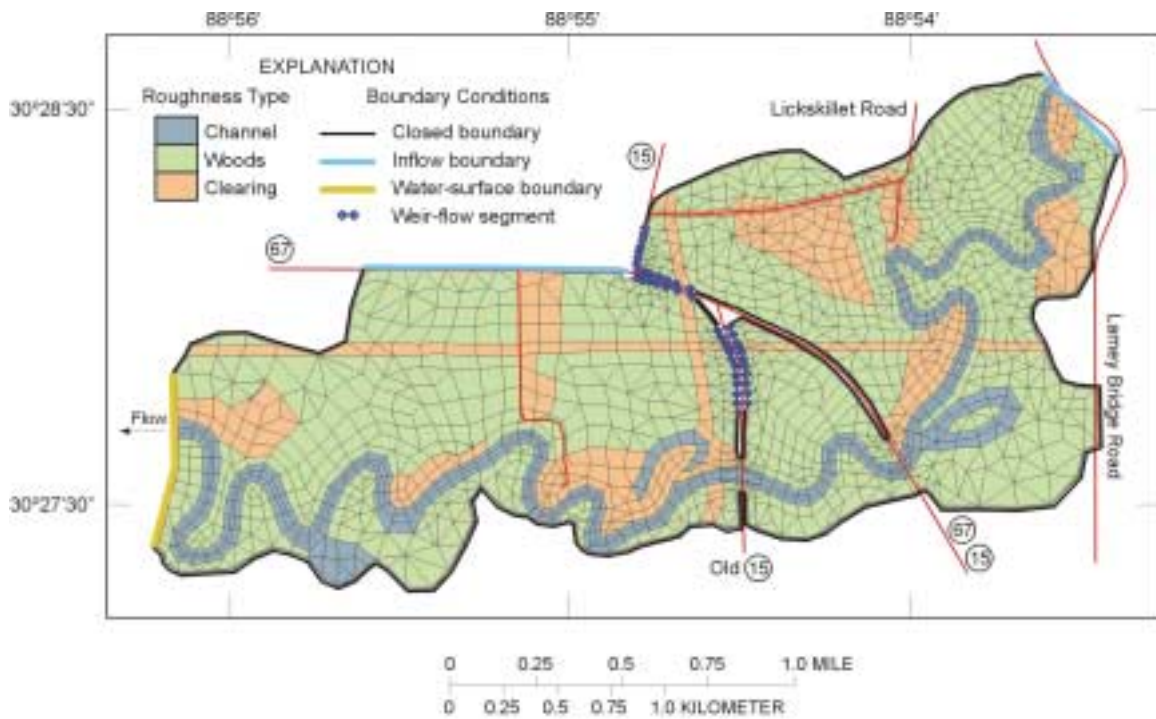
Figure 7. Finite-element grid for existing conditions with roughness types shaded.
