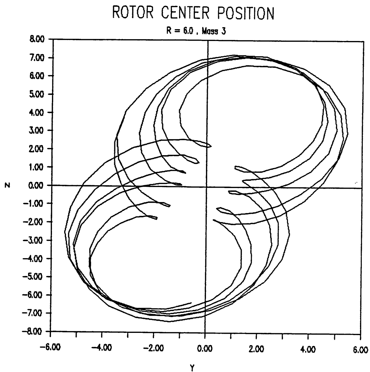
Fig. 4.26. Rotor Response at Mass 3 with R = 6 , \bar{g} = 10 .
