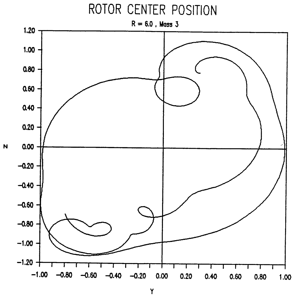
Fig. 4.22. Rotor Response at Mass 3 with R = 6 , \bar{g} = 1 .
