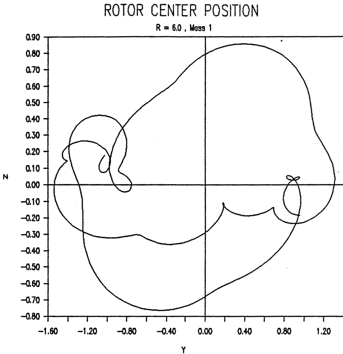
Fig. 4.20. Rotor Response at Mass 1 with R = 6 , \bar{g} = 1 .
