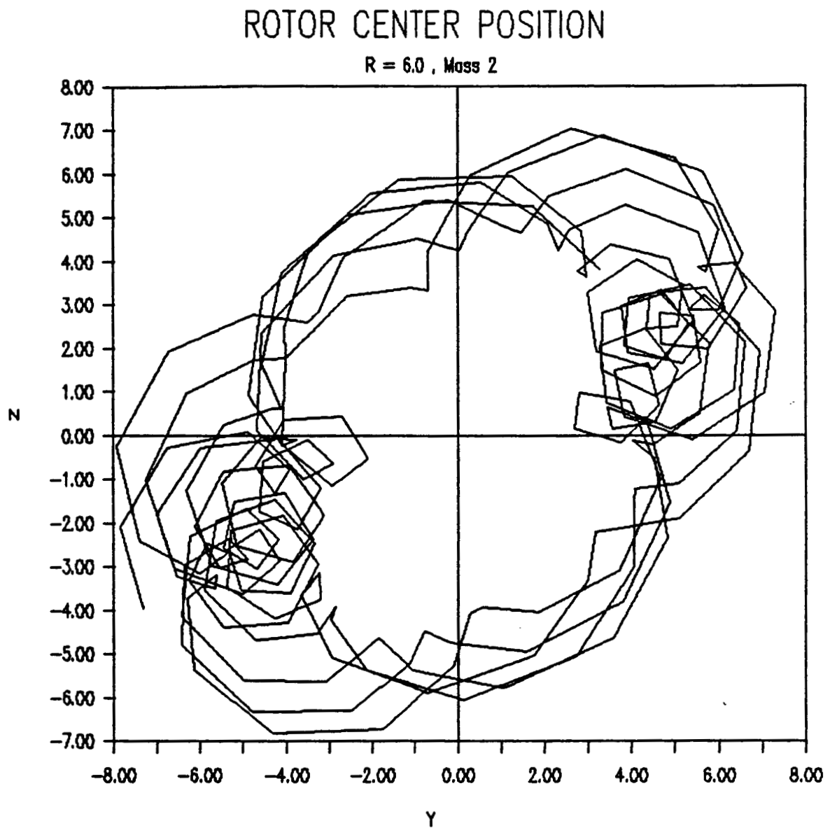
Fig. 4.25. Rotor Response at Mass 2 with R = 6 , \bar{g} = 10 .
