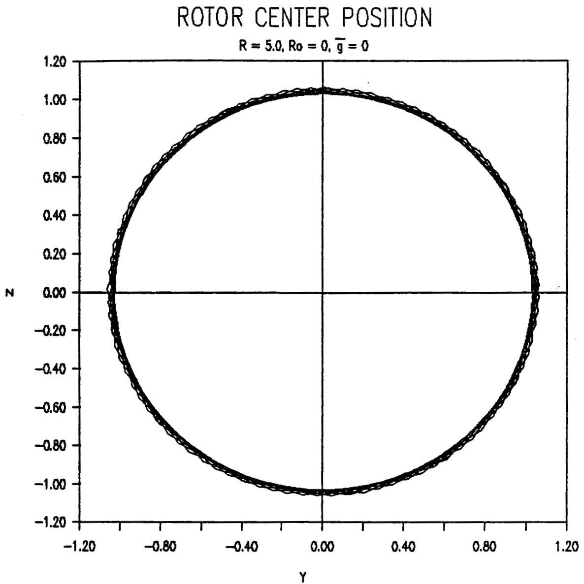
Fig. 3.6. Rotor Response at R = 5, \bar{g} = 0 .
