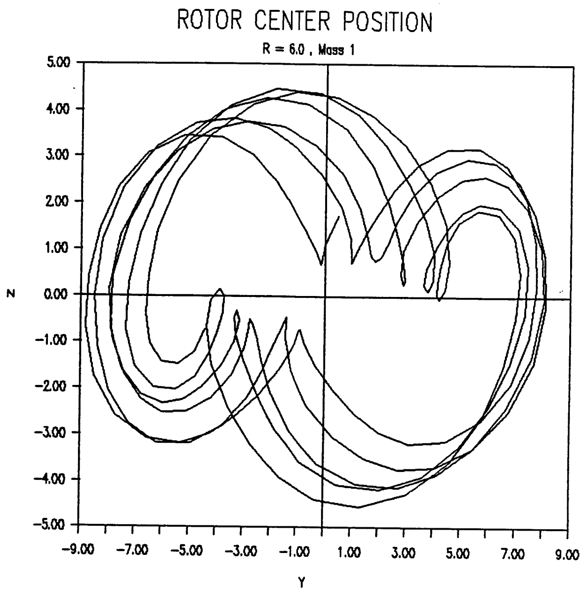
Fig. 4.24. Rotor Response at Mass 1 with R = 6 , \bar{g} = 10 .
