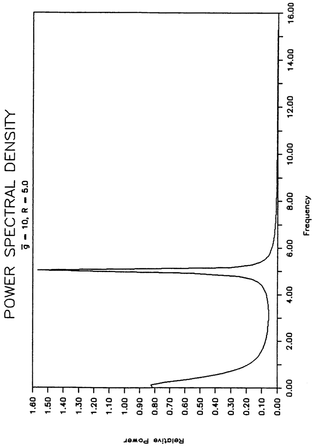
Fig. 3.11. Power Spectral Density for Response of Fig. 3.10.
