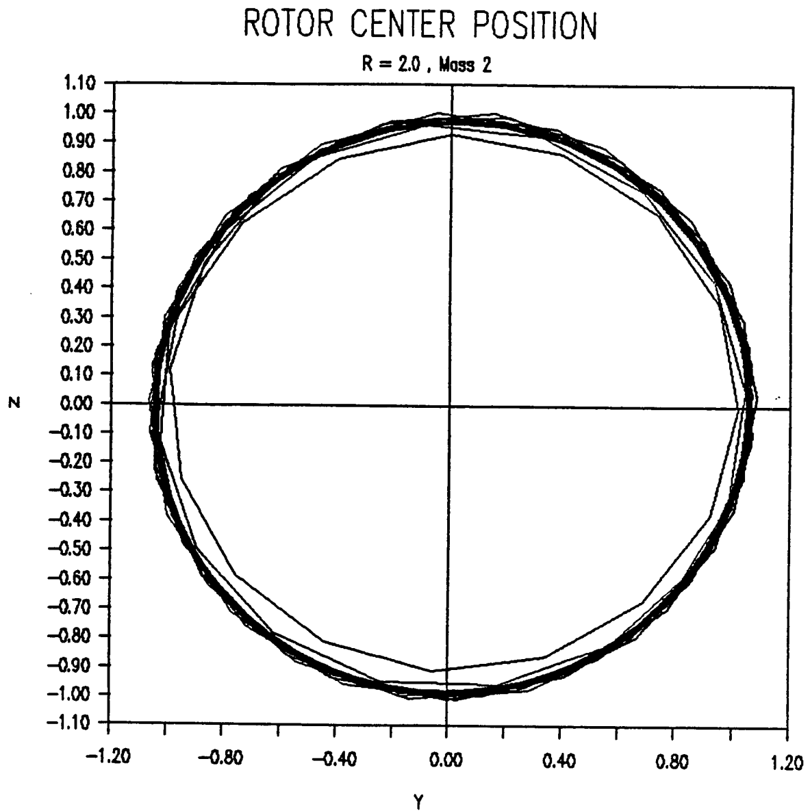
Fig. 4.18. Rotor Response at Mass 2 with R = 2 , \bar{g} = 1 .
