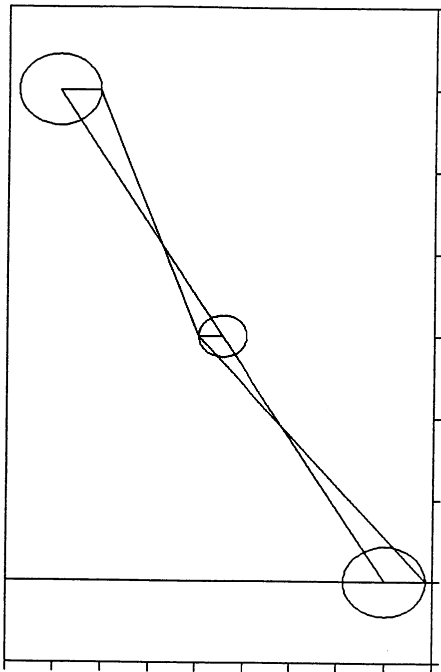
Fig. 4.5. Modal Orbit Shape of Third Unstable Mode at R = 4.65 .
