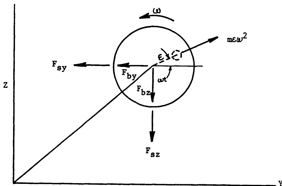
Fig. 3.2. Force Diagram for Rotor Model
