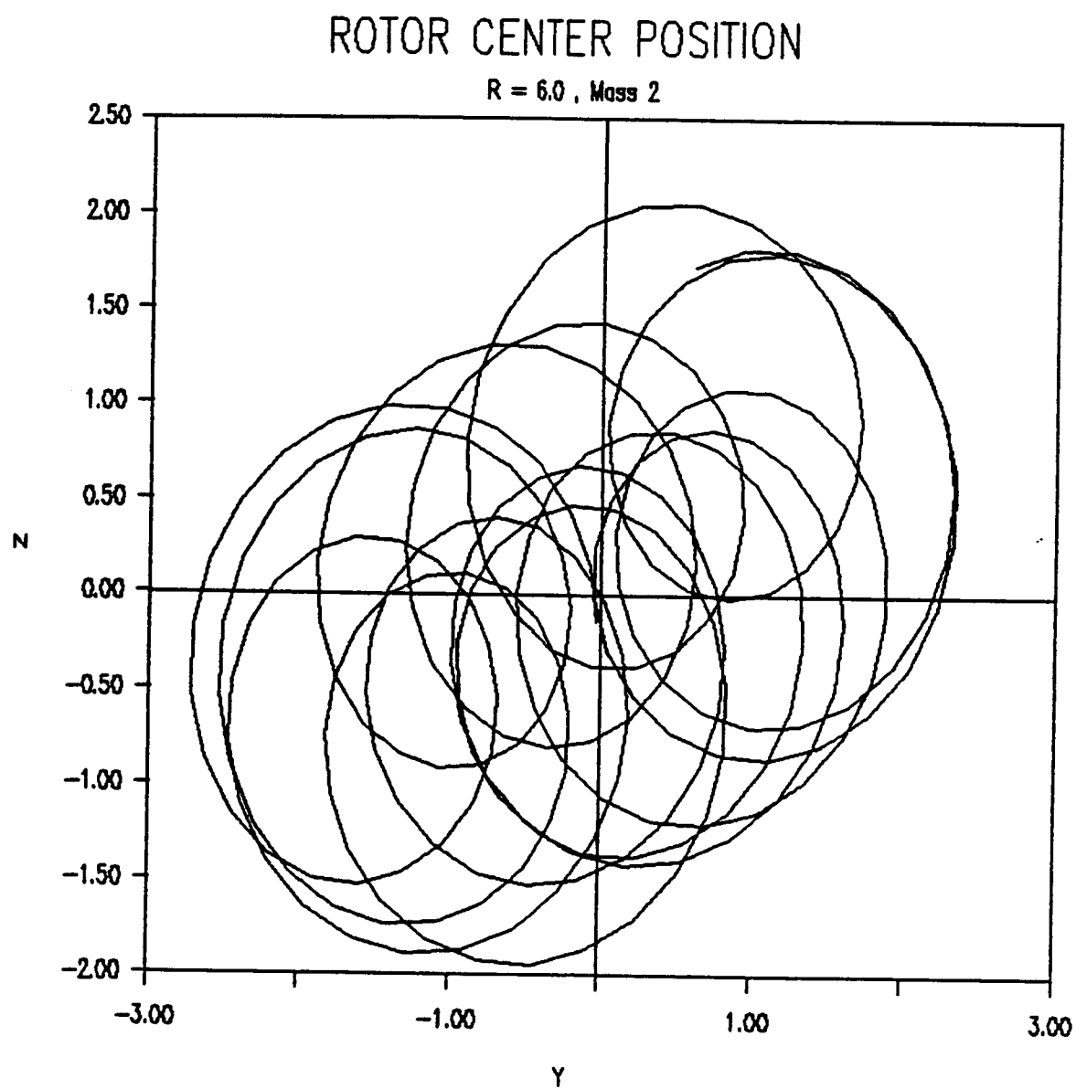
Fig. 4.21. Rotor Response at Mass 2 with R = 6 , \bar{g} = 1 .
