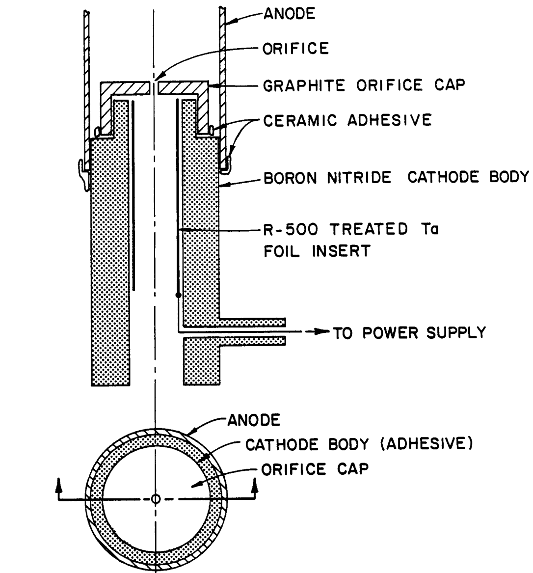
a. GRAPHITE ORIFICE CAP CONFIGURATION (WITH CYLINDRICAL CAP HAVING ORIFICE ON CENTER)
