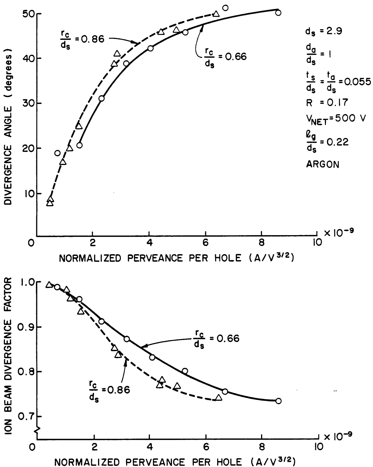
Fig. 77 Effect of Constraining Mesh Radius on Curvature on Divergence Characteristics
