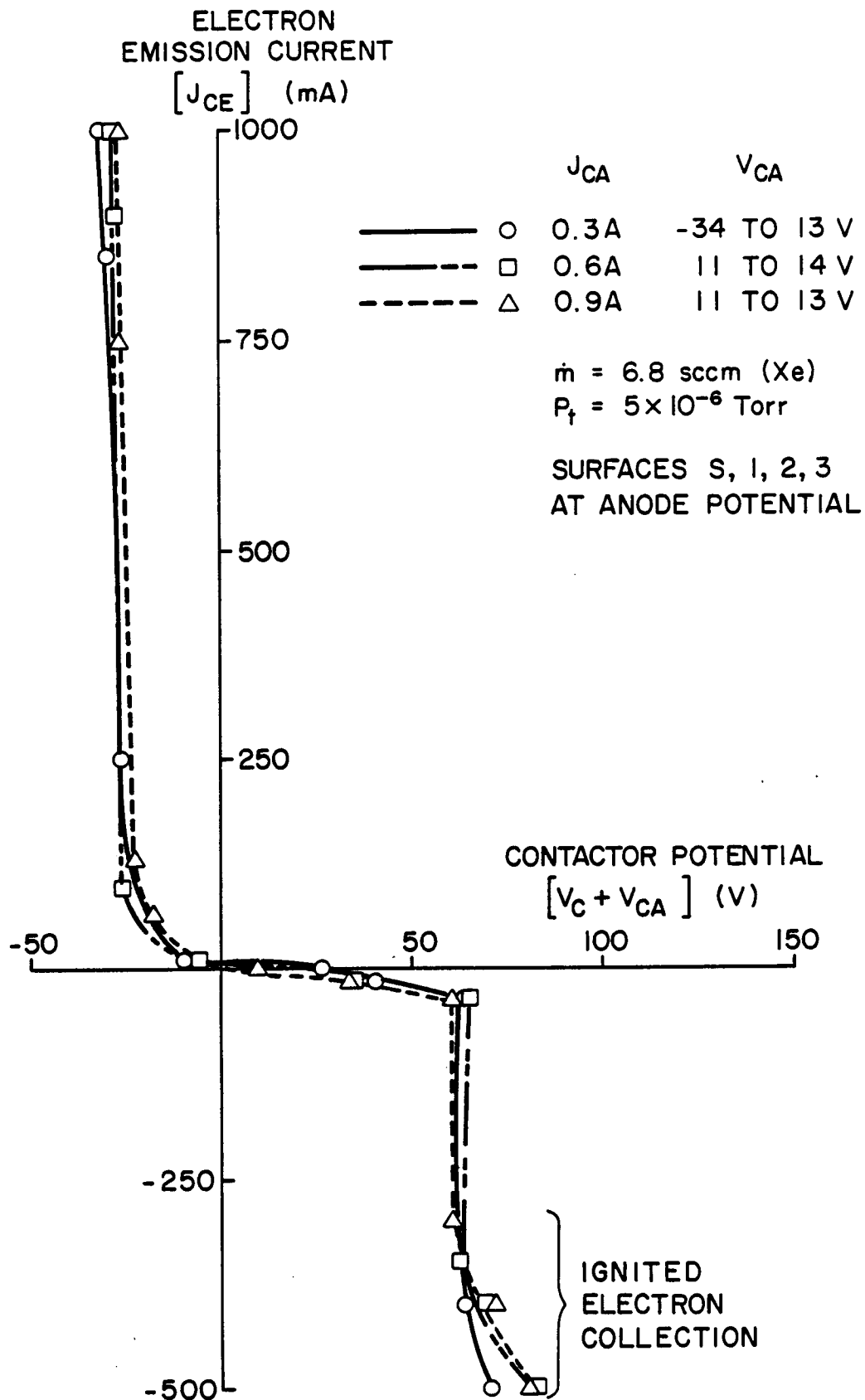
Fig. 28 Effect of Contactor Anode Current on Performance at a High Flowrate
