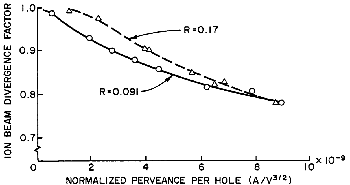
Fig. 76 Effect of Net-to-Total Accelerating Voltage Ratio on Divergence Characteristics
