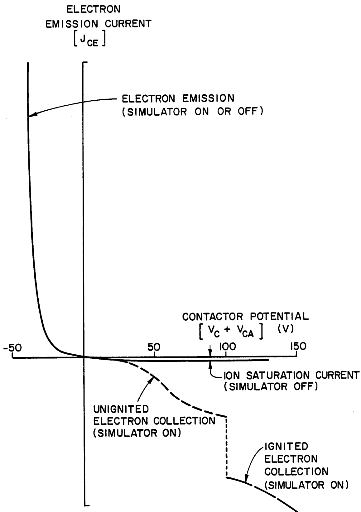
Fig. 8 Generic Contactor Characteristics
