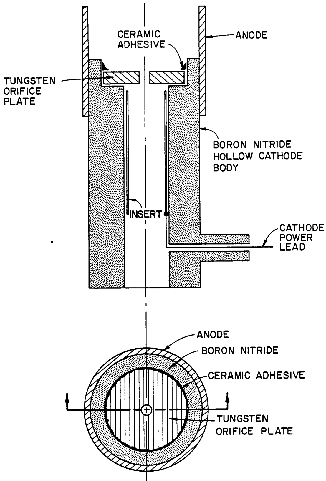
Fig. 44 Boron Nitride Body/Tungsten Orifice Plate Hollow Cathode
