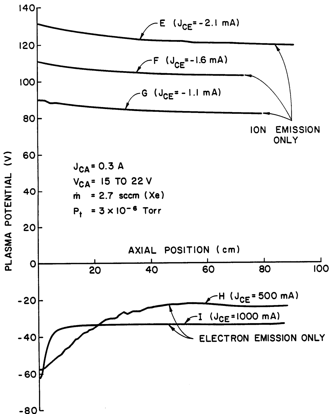
Fig. 14 Typical Plasma Potential Profiles for Conventional contactor with Simulator off
