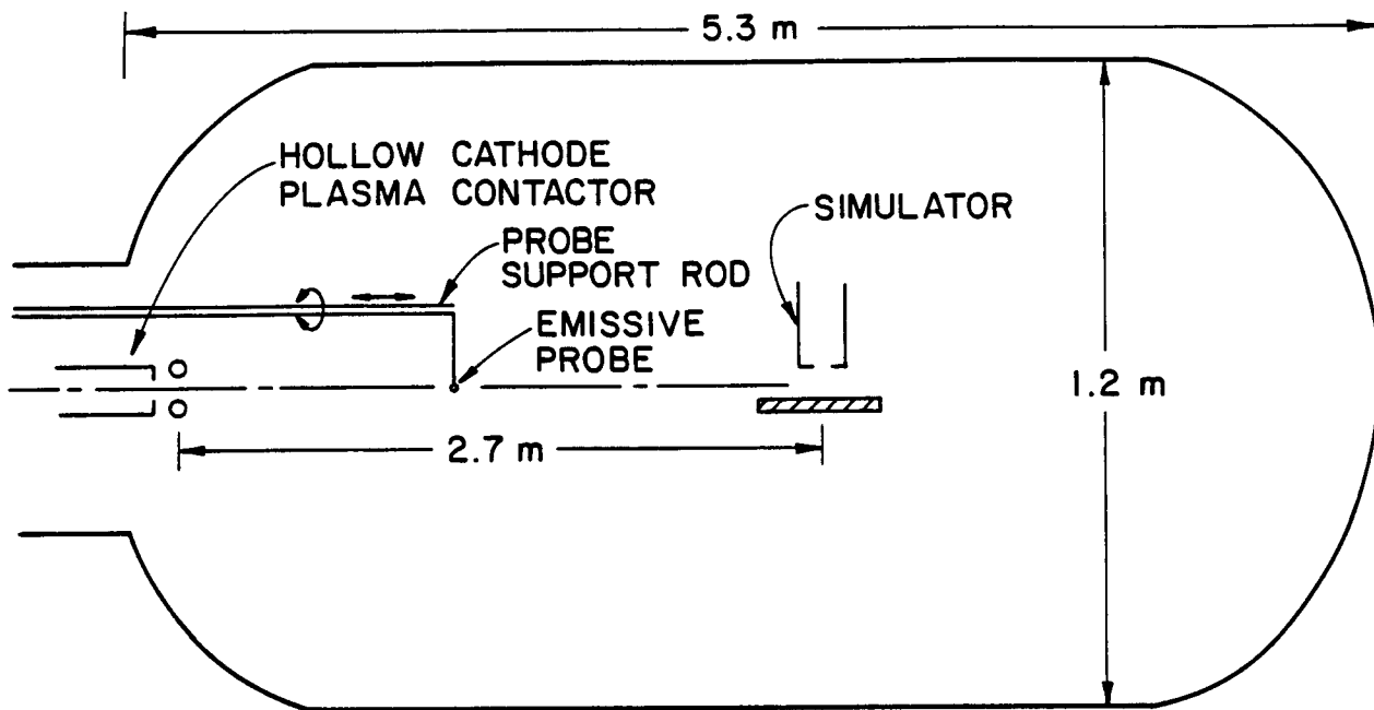
a. MECHANICAL
