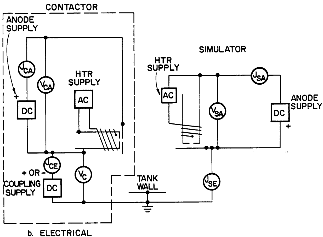
Fig. 3 Schematic Diagrams
