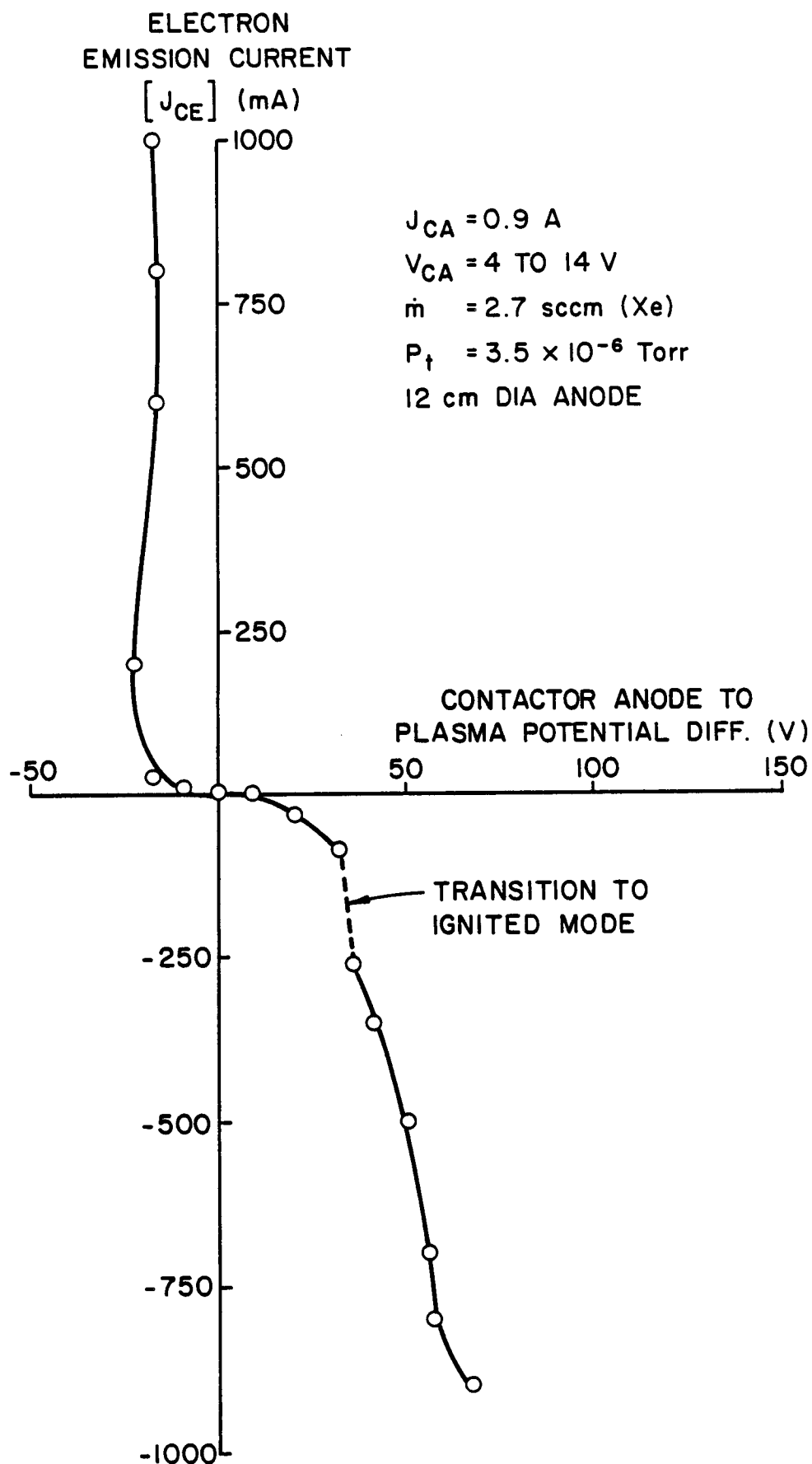
Fig. 40 Contactor Anode-to Ambient Plasma Potential Difference vs. Emission Current-High Anode Current Case
