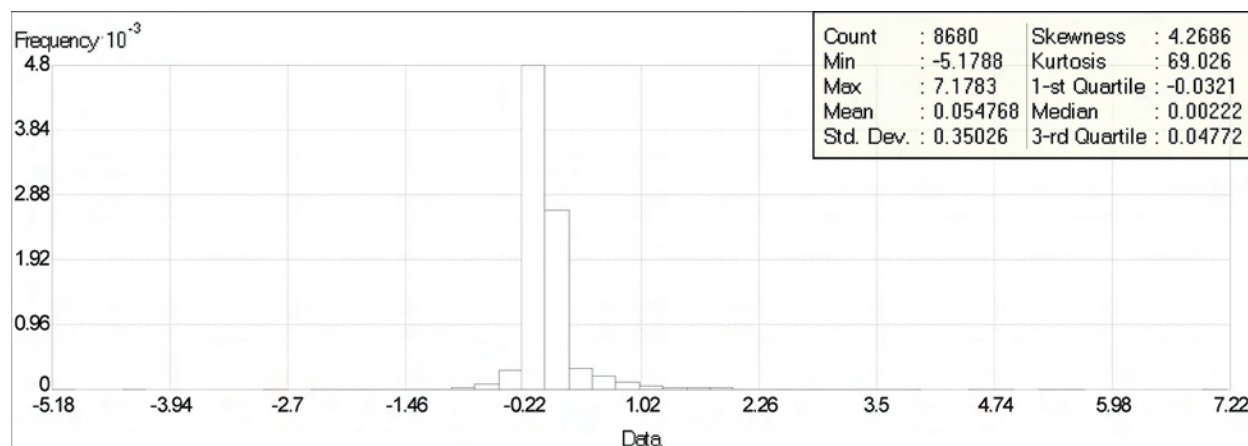
Figure 18. Histogram of the difference between NOS hydrographic survey H10236 (relatively dense survey in North Bay) and the 1 arc-second pre-surfaced bathymetric grid. Discrepancies between survey soundings and the pre-surface grid result from the averaging of several closely spaced soundings.
