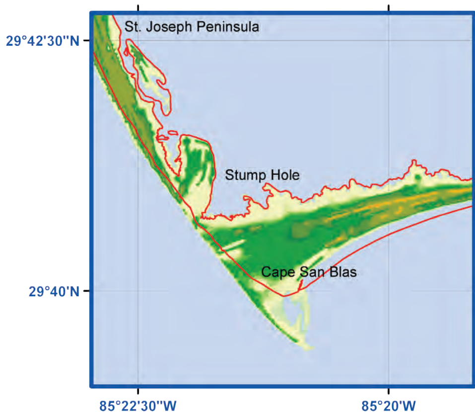
Figure 13. Color image of the NED DEM in the vicinity of Cape San Blas. Blue represents “zero” values in NED DEM over the open ocean. Combined coastline, derived from post-Dennis LiDAR survey, in red illustrates the magnitude of coastal change that has occurred in this area.
