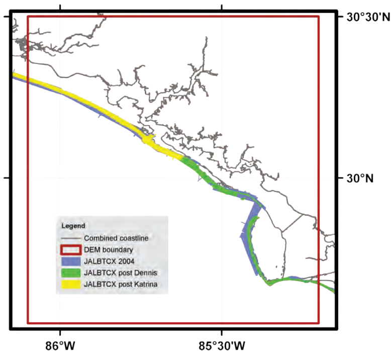
Figure 14. Spatial coverage of JALBTCX high-resolution (5-meter point spacing) coastal bathymetric–topographic LiDAR surveys utilized in DEM development.
