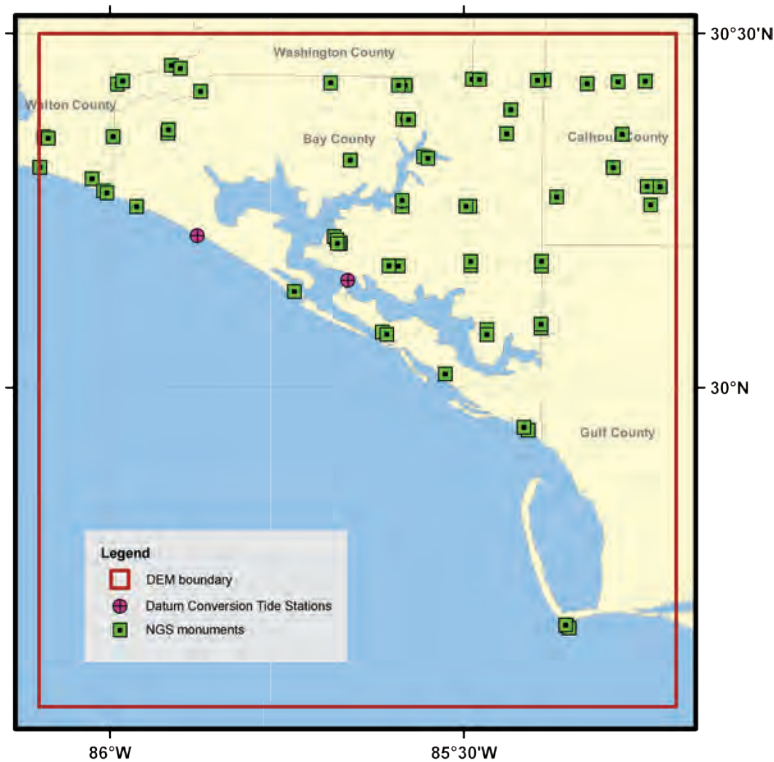
Figure 23. Location of NGS monuments and NOAA tide stations in the Panama City region. Tide stations used to convert between vertical datums; NGS monument elevations used to evaluate the DEM.
