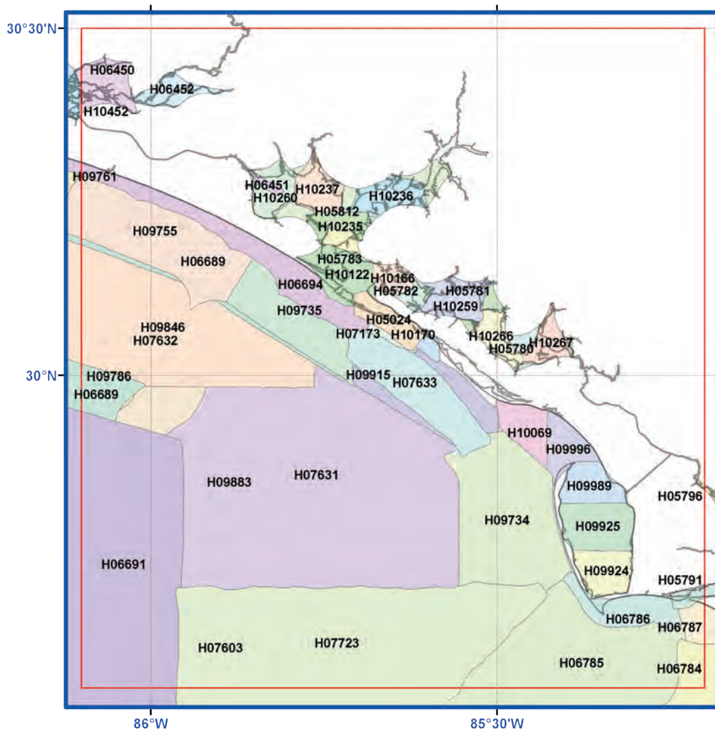
Figure 8. Digital NOS hydrographic survey coverage in the Panama City region. DEM boundary in red, combined coastline in gray.
