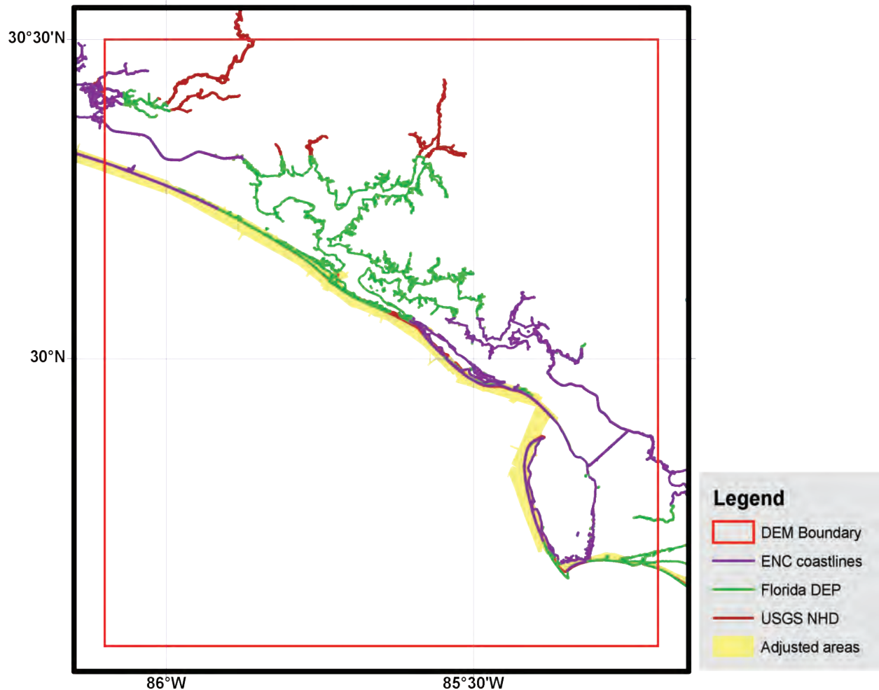
Figure 6. Digital coastline segments used to create a 'combined coastline' for the Panama City region. Areas in yellow highlight coastline segments that were manually adjusted to match recent bathymetric–topographic LiDAR surveys.
