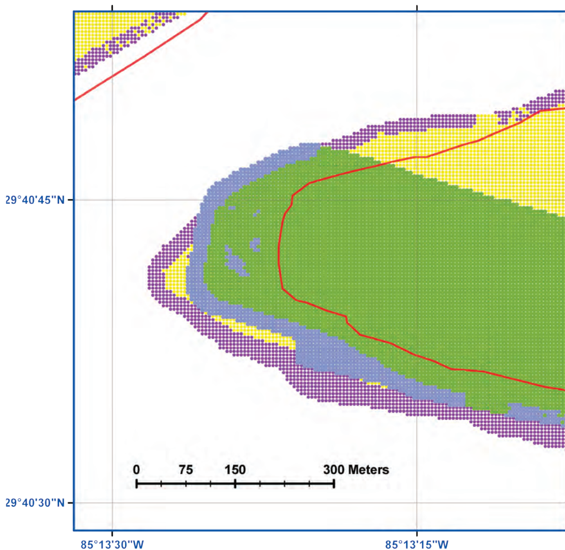
Figure 7. Example of the difference in coastal morphology around Indian Pass between 2004 and 2005 LiDAR surveys. Green–blue transition represents the MHW coastline in the 2004 JALBTCX LiDAR survey. Yellow–purple transition represents the MHS coastline in the 2005 post-Dennis JALBTCX LiDAR survey. The FDEP shoreline is shown in red.
