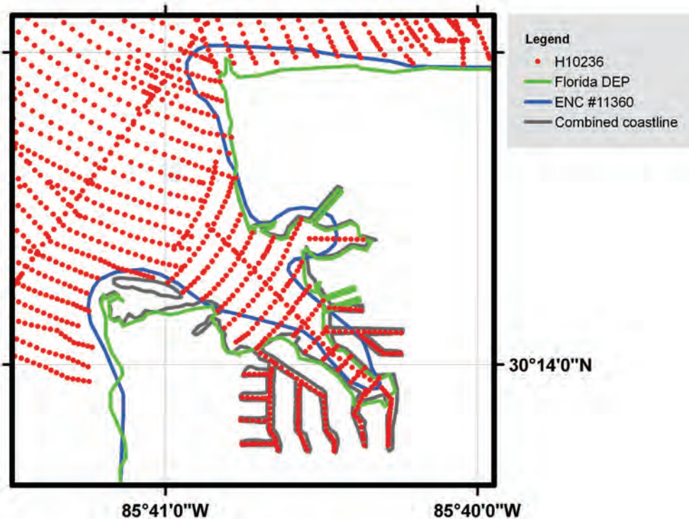
Figure 5A. Detail of coastline datasets for Upper Goose Bayou. 1987 NOS survey H10236, in red, extended into upper reaches of the bayou. Neither the FDEP coastline (green) nor coastline from ENC #11360 (blue, scale 1:456,394) captured the intricate details of the bayou. The combined coastline (gray) was built by digitizing the coastline from RNC #11390 (scale 1:40,000; see Fig 5B).
