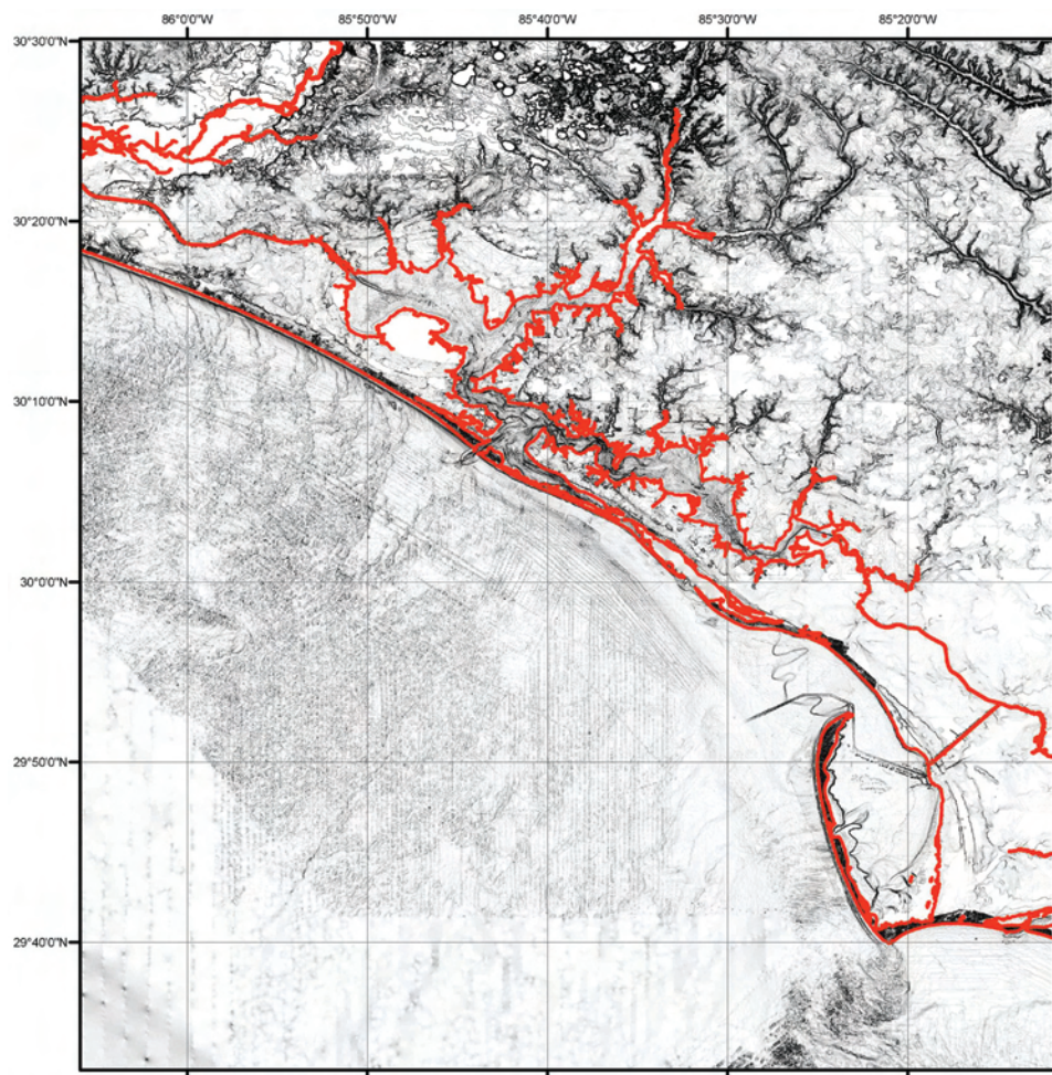
Figure 19. Slope map of the Panama City DEM. Flat-lying slopes are white; dark shading denotes steep slopes; combined coastline in red.
