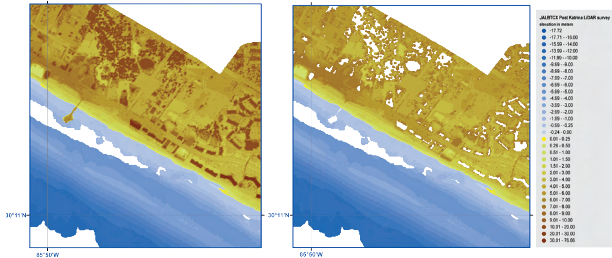
Figure 15. Post-Hurricane Katrina JALBTCX data before (left) and after (right) NGDC processing to simulate bare earth. Note pier and beach-front structures present before processing.
