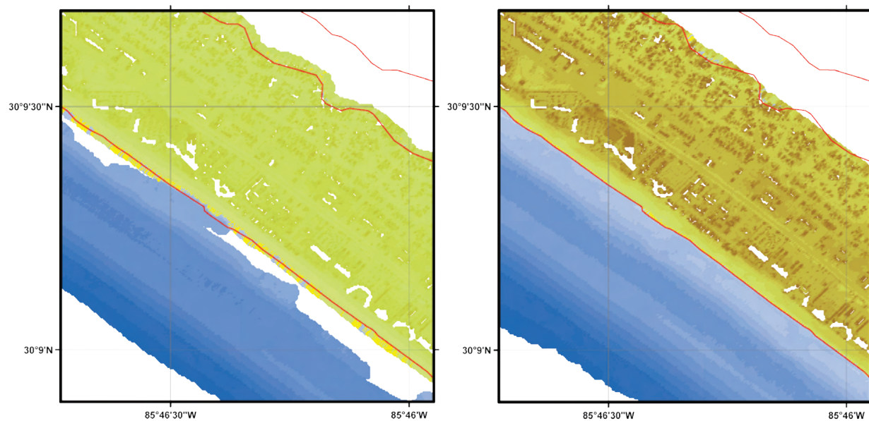
Figure 16. Indistinct MHW coastline in post-Hurricane Dennis JALBTCX survey (left). Clearly defined MHW coastline in post-Hurricane Katrina JALBTCX survey (right).
