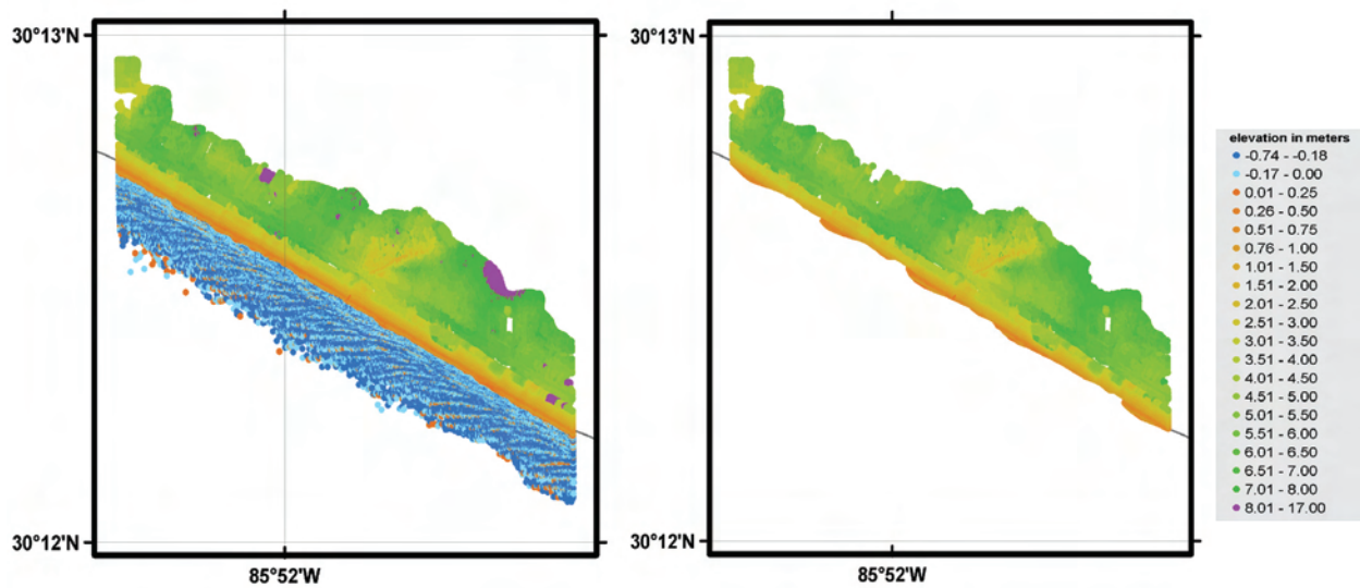
Figure 12. FDEP topographic LiDAR data before (left) and after (right) NGDC processing.
