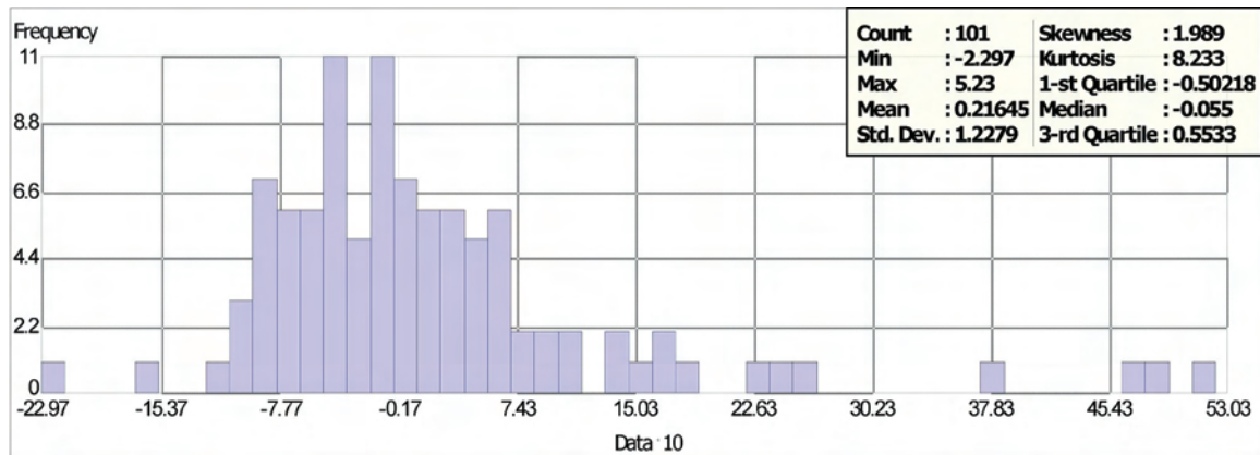
Figure 22. Histogram of the differences between NGS geodetic monument elevations and the Panama City DEM.
