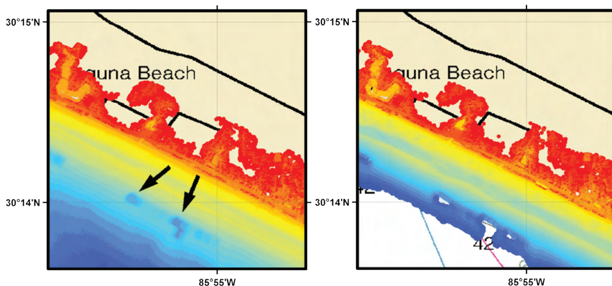
Figure 17. Beach replenishment areas offshore Laguna Beach. JALBTCX 2004 survey data, on left, reveals numerous geometric shapes of deeper than expected elevations (arrows), which are dredged source areas for beach restoration and replenishment projects in the Panama City region. Right panel shows the 2005 post-Hurricane Katrina dataset in the same area, which also reveals these pits.
