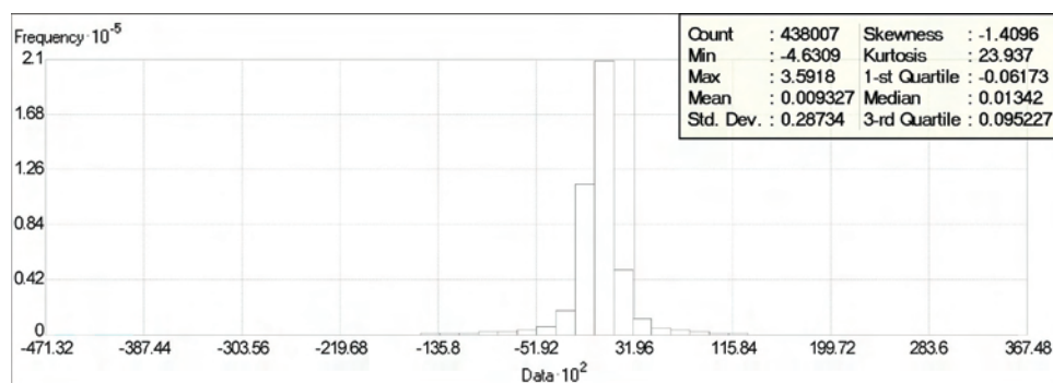
Figure 21. Histogram of the difference between one file of the post-Katrina JALBTCX coastal bathymetric–topographic LiDAR survey (438,007 points) and the Panama City DEM.
