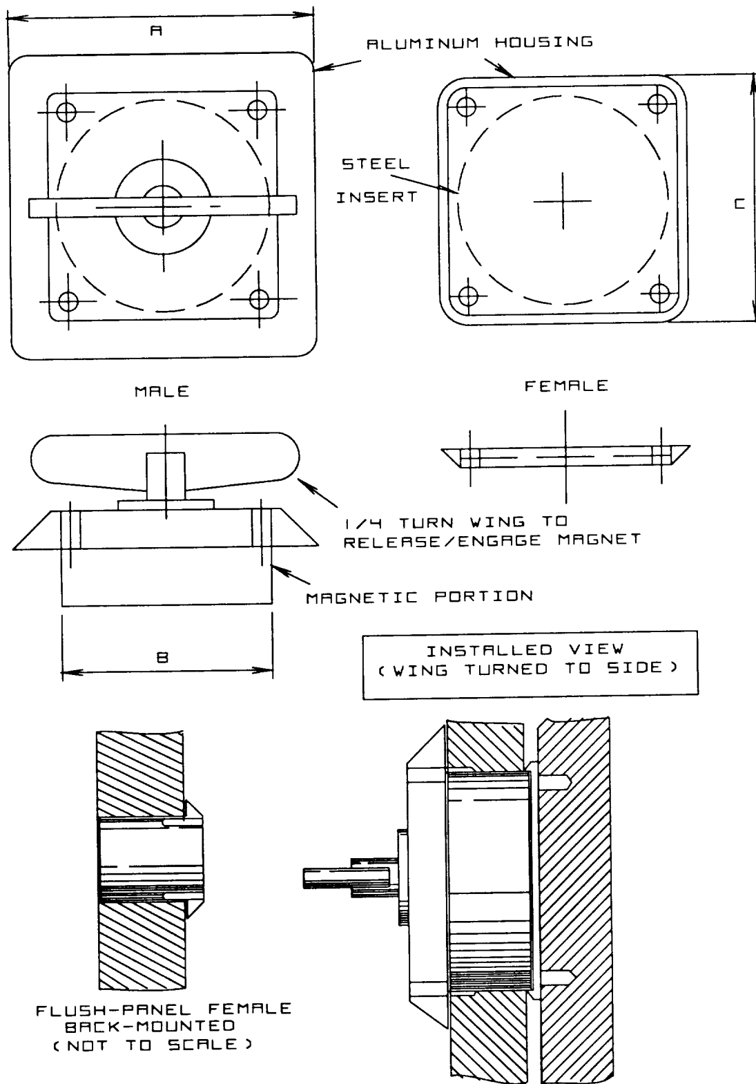
Figure 3 DISENGAGABLE MAGNETIC FASTENER
