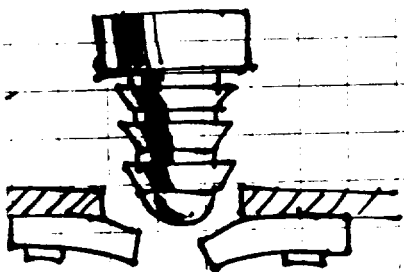
SEMI-FLEXIBLE LEAVES
