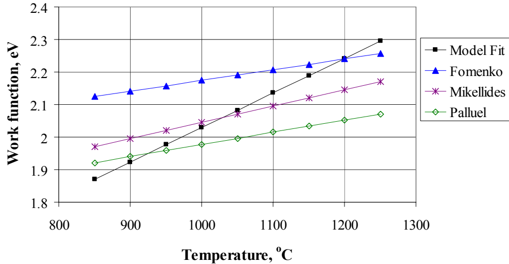
Figure 5.—Work function used to fit temperature data compared to other published values (Fomenko (ref. 23), Mikellides (ref. 24), and Palluel (ref. 18)).
