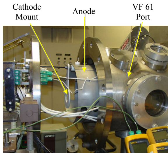
Figure 8.—Picture showing VF61 port 1 test setup.
