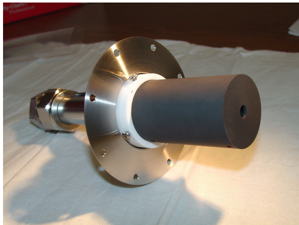
Figure 7.—Pretest photograph taken of the lab model hollow cathode assembly with graphite keeper.
