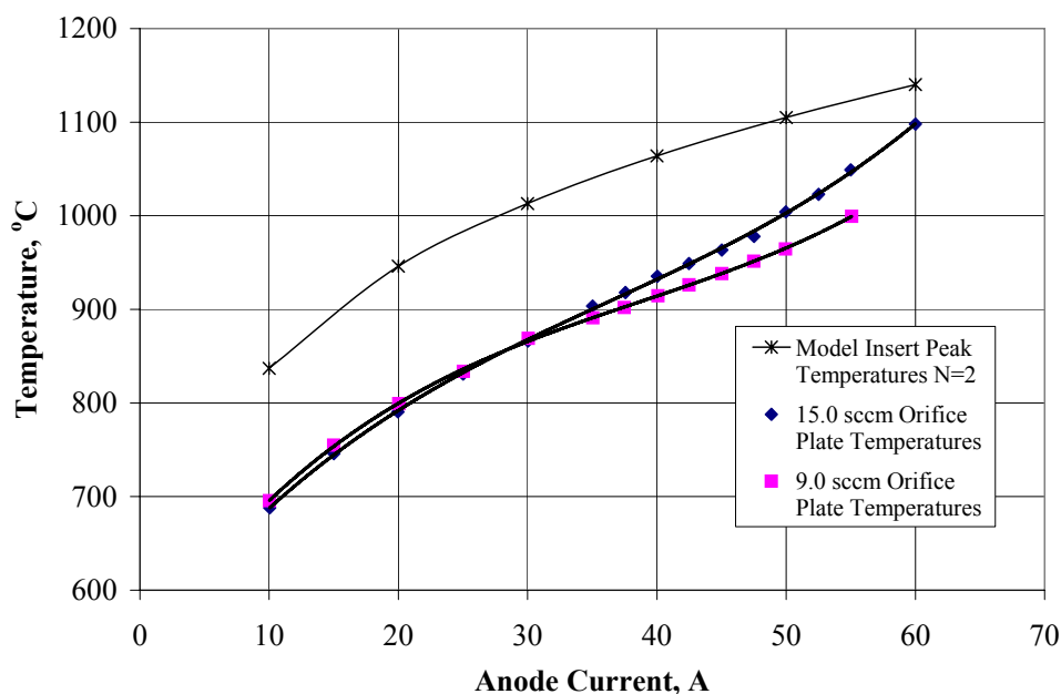
Figure 10.—Graph showing cathode orifice plate temperature for varying anode currents.
