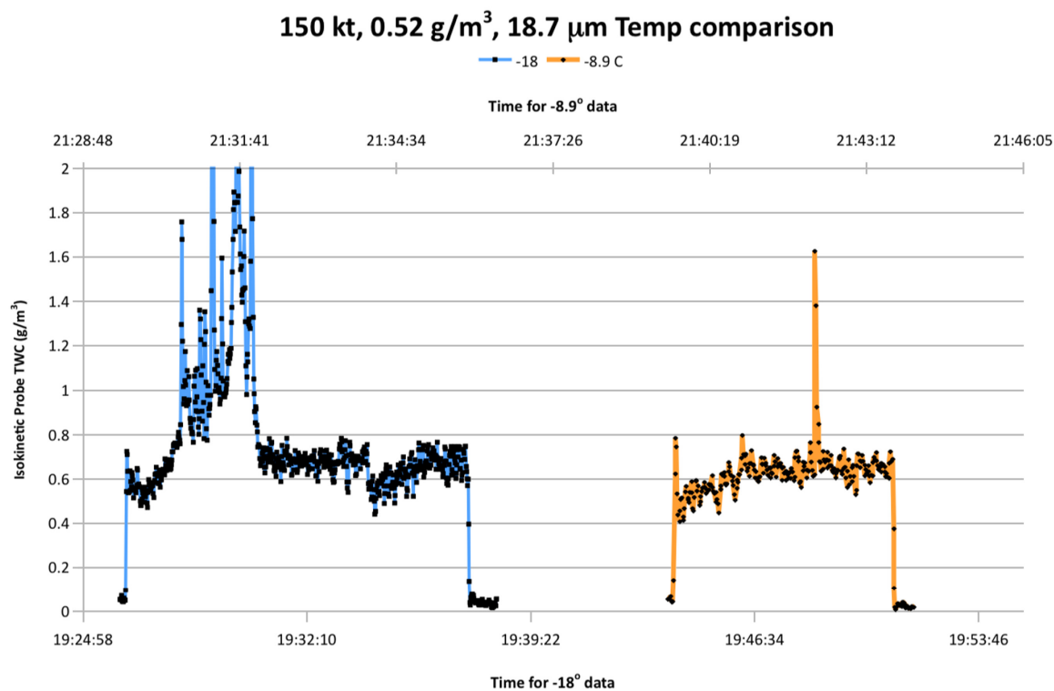
Figure 24.—Temperature comparisons at 150 kts and 0.5 g/m 3 .
