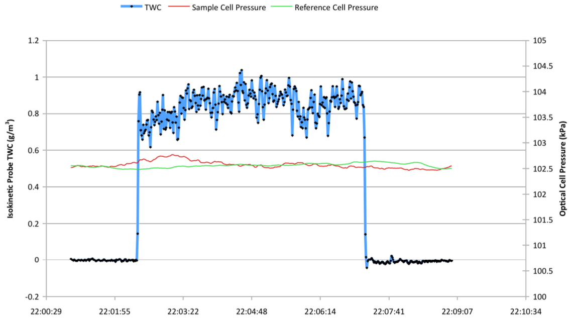
Figure 5.—Measurement cell pressure tracings.
