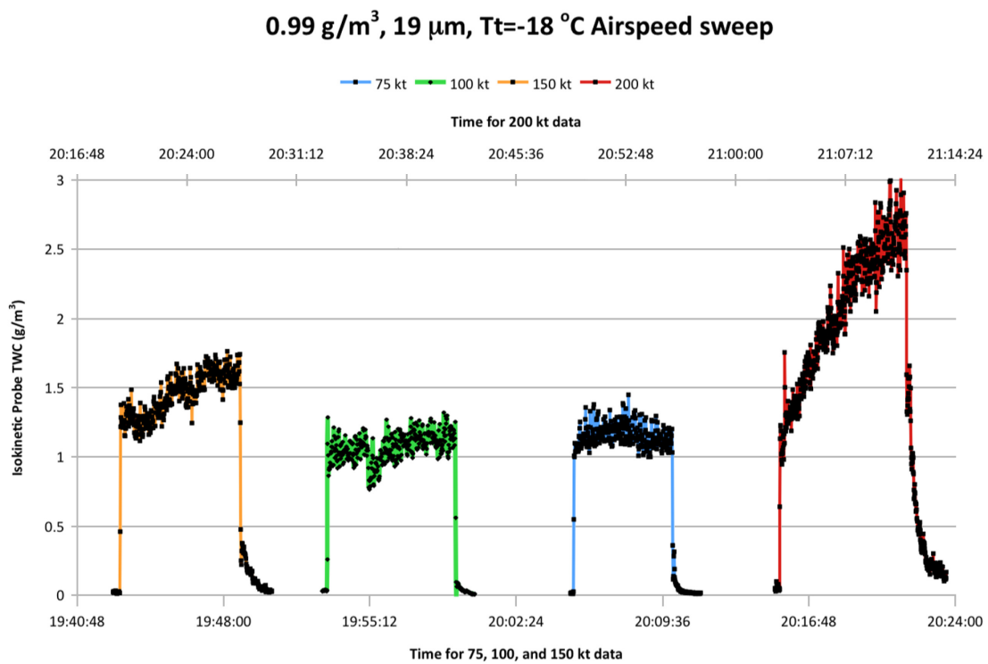
Figure 16.—Airspeed sweep at 0.99 g/m 3 .
