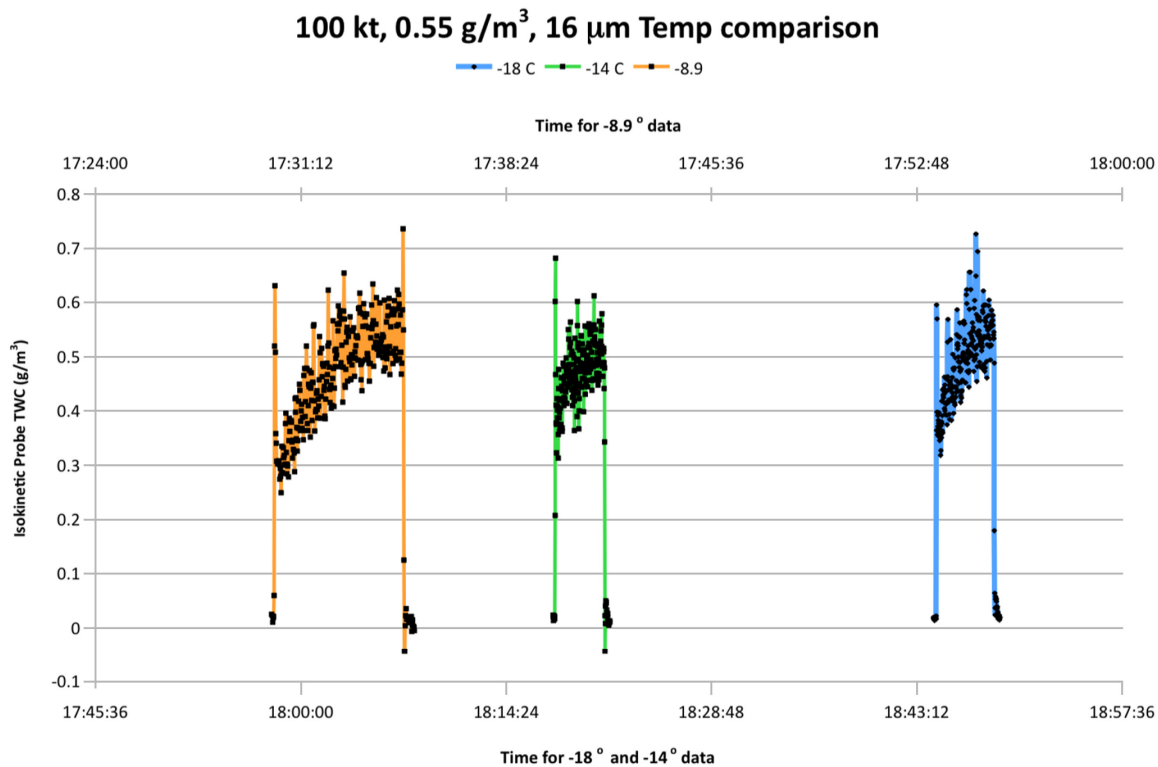
Figure 23.—Temperature comparisons at 100 kts.
