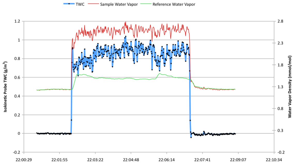
Figure 6.—Water vapor tracings.
