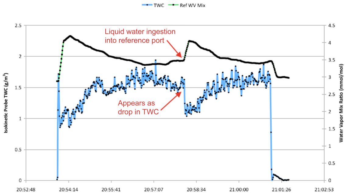
Figure 8.—Ingested water into reference port (run 35).
