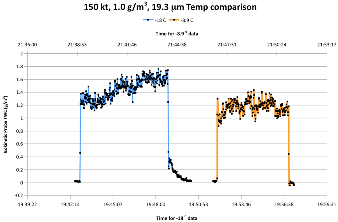
Figure 25.—Temperature comparisons at 150 kts and 1.0 g/m 3 .
