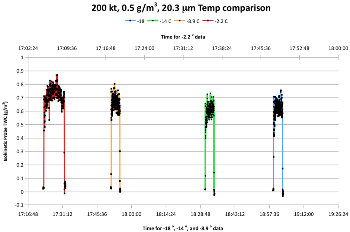
Figure 26.—Temperature comparisons at 200 kt and 0.5 g/m 3 .
