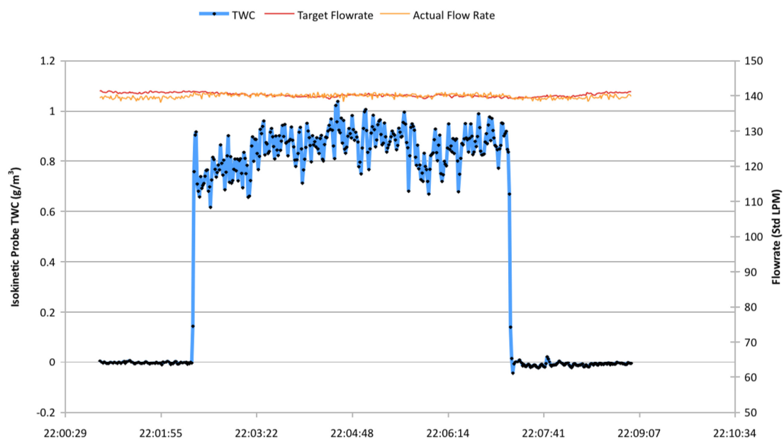
Figure 4.—Flow rate tracings (target and actual).
