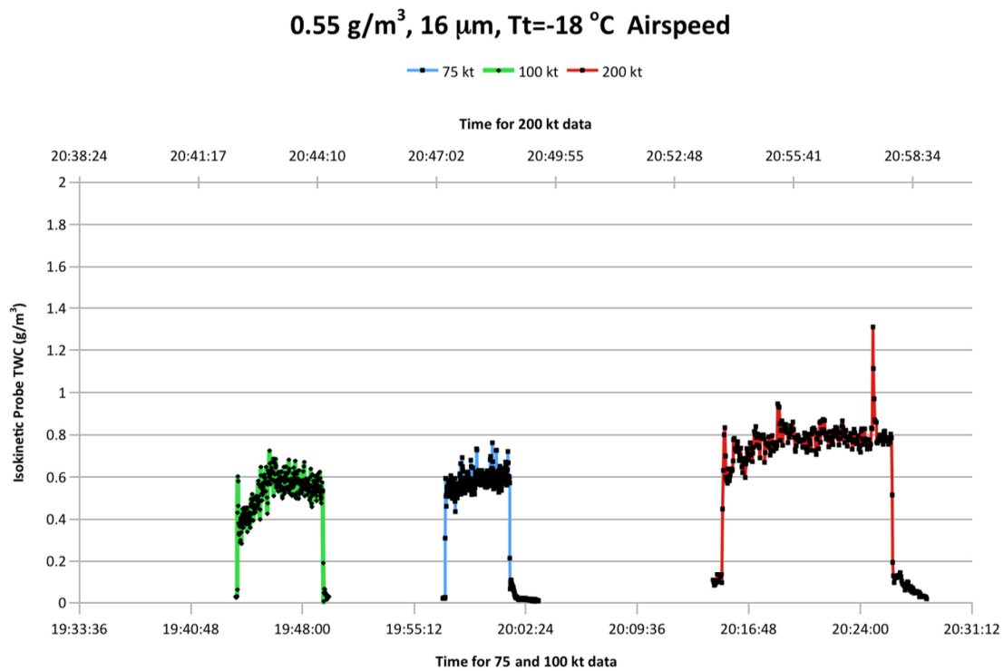
Figure 15.—Airspeed sweep at 0.55 g/m 3 .
