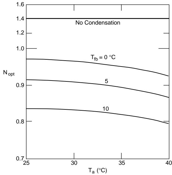
Figure 17. Optimum fin parameter, N_{opt} , for a vertical rectangular fin with moisture condensation. Adapted from Kilic and Onat (1981).
