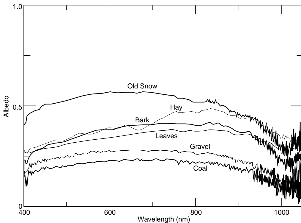
Figure 4. Albedo measurements of the dusted surfaces (March 1994).
