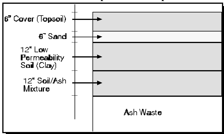
Cross-Section Diagram of the Chisman Creek Superfund Site Cap
