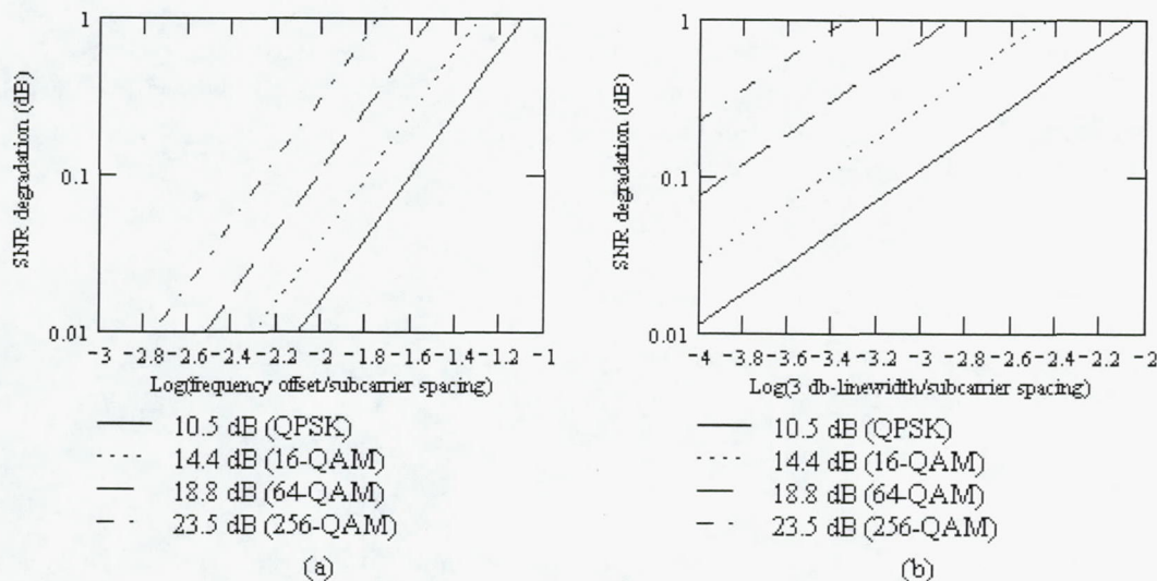
Figure 3: SNR degradation in dB versus the normalized frequency offset (a) and the normalized phase noise linewidth (b). The original SNRs are the values at which BER = 10^{-6} : 23.5 dB for 256-QAM, 18.8 dB for 64-QAM, 14.4 dB for 16-QAM, and 10.5 dB for QPSK.
