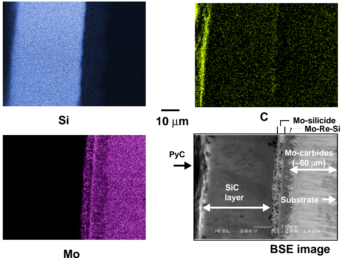
Fig. 16 Elemental x-ray maps for uncoated PM Mo-47.5Re with PyC/SiC deposition and heat treated at 2000°F for 200 hr (#29).
