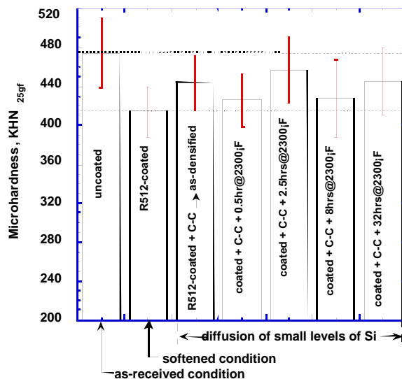
Fig. 10 Microhardness of AC Mo-41Re substrate.
