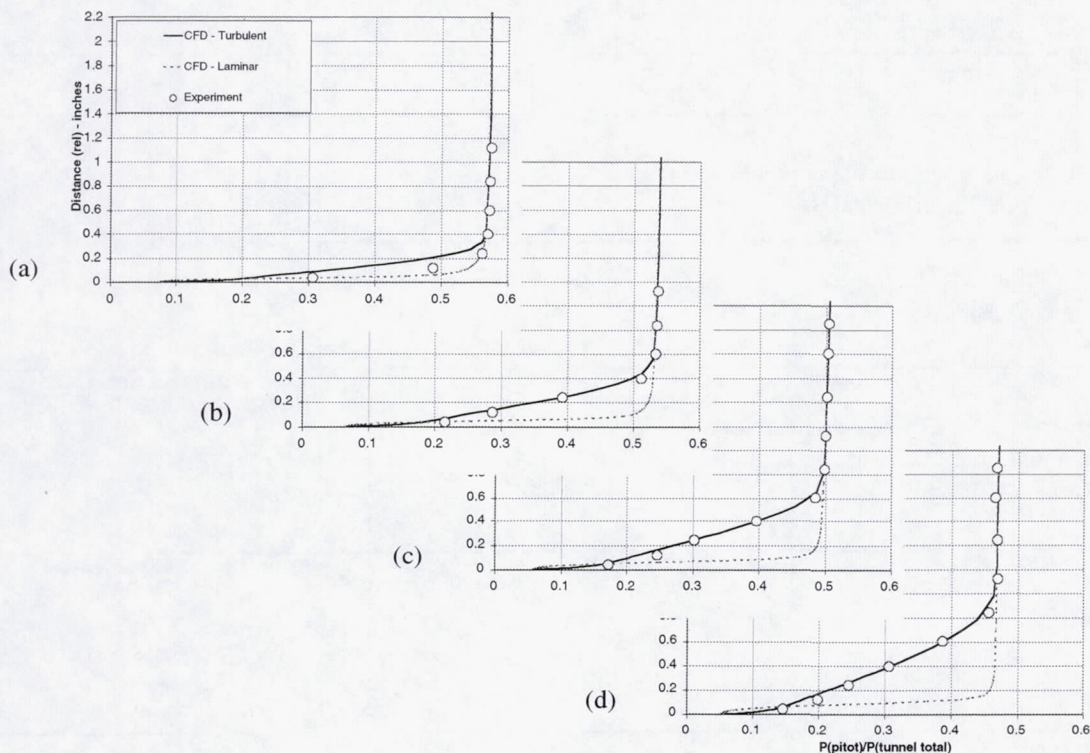
Figure 8 (a-d) – Blunt-nose Boundary-Layer Rake Normalized Pitot Pressure Profiles along the forebody at various axial stations (turbulent and laminar CFD vs. experimental (all without grit)), Mach 2.5, \alpha=0^\circ , (a) x=32.5 inches, (b) x=53.94 inches, (c) x=75.38 inches, (d) x=100.33 inches.
