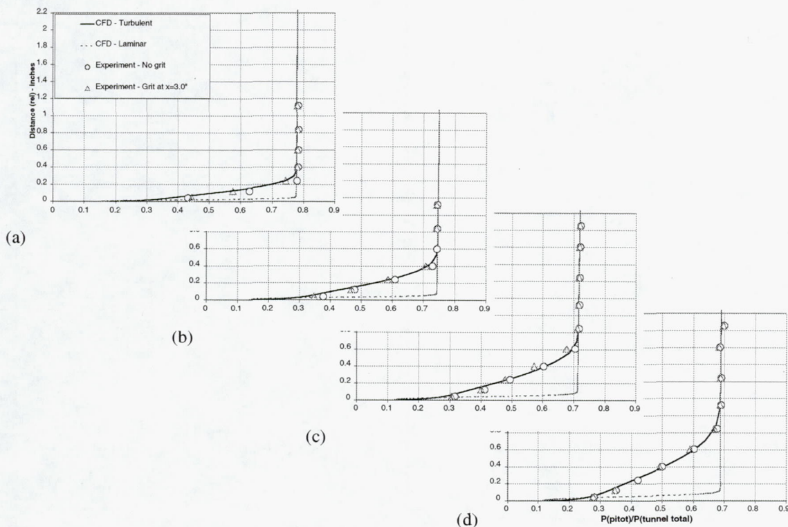
Figure 7 (a-d) – Sharp-nose Boundary-Layer Rake Normalized Pitot Pressure Profiles along the forebody at various axial stations (turbulent and laminar CFD vs. experimental (with and without grit)), Mach 2.0, \alpha=0^\circ , (a) x=32.5 inches, (b) x=53.94 inches, (c) x=75.38 inches, (d) x=100.33 inches.
