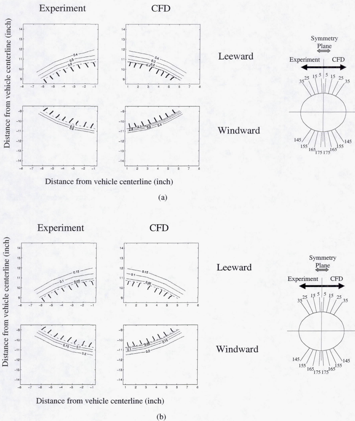
Figure 5 – Sharp-nose Flowfield Rake Normalized Pitot Pressure Contour Plots for \alpha=3^\circ at x=98.95 inches (experiment vs. turbulent CFD), (a) Mach 2.5, \alpha=3^\circ , (b) Mach 3.5, \alpha=3^\circ .
