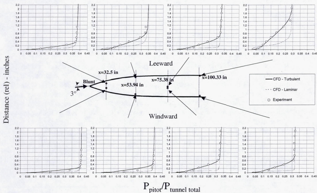
Figure 9 – Blunt-nose Boundary-Layer Rake Normalized Pitot Pressure Profiles along the forebody at various axial stations, Mach 3.0, \alpha=3^\circ .
