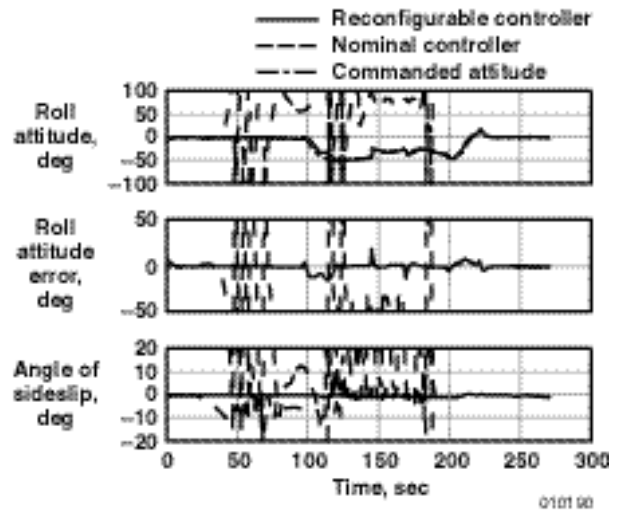
(b) Lateral-directional.
