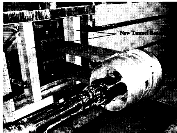
Fig. 12. Wind Tunnel Modifications for RAN Installation
