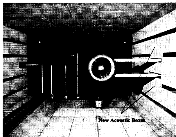
Fig. 13. Front View of RAN Hardware in LSWT
