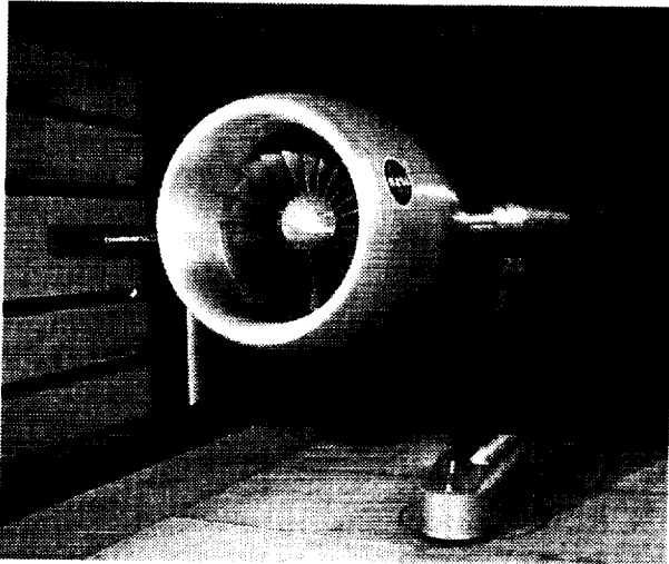
Fig. 1. Turbofan Simulation Test in NASA Glenn 9'x15' LSWT in Standard Acoustic Configuration
