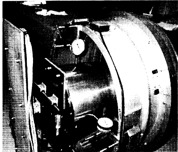
Fig. 11. Checkout of RAN w/PACS Traverse
