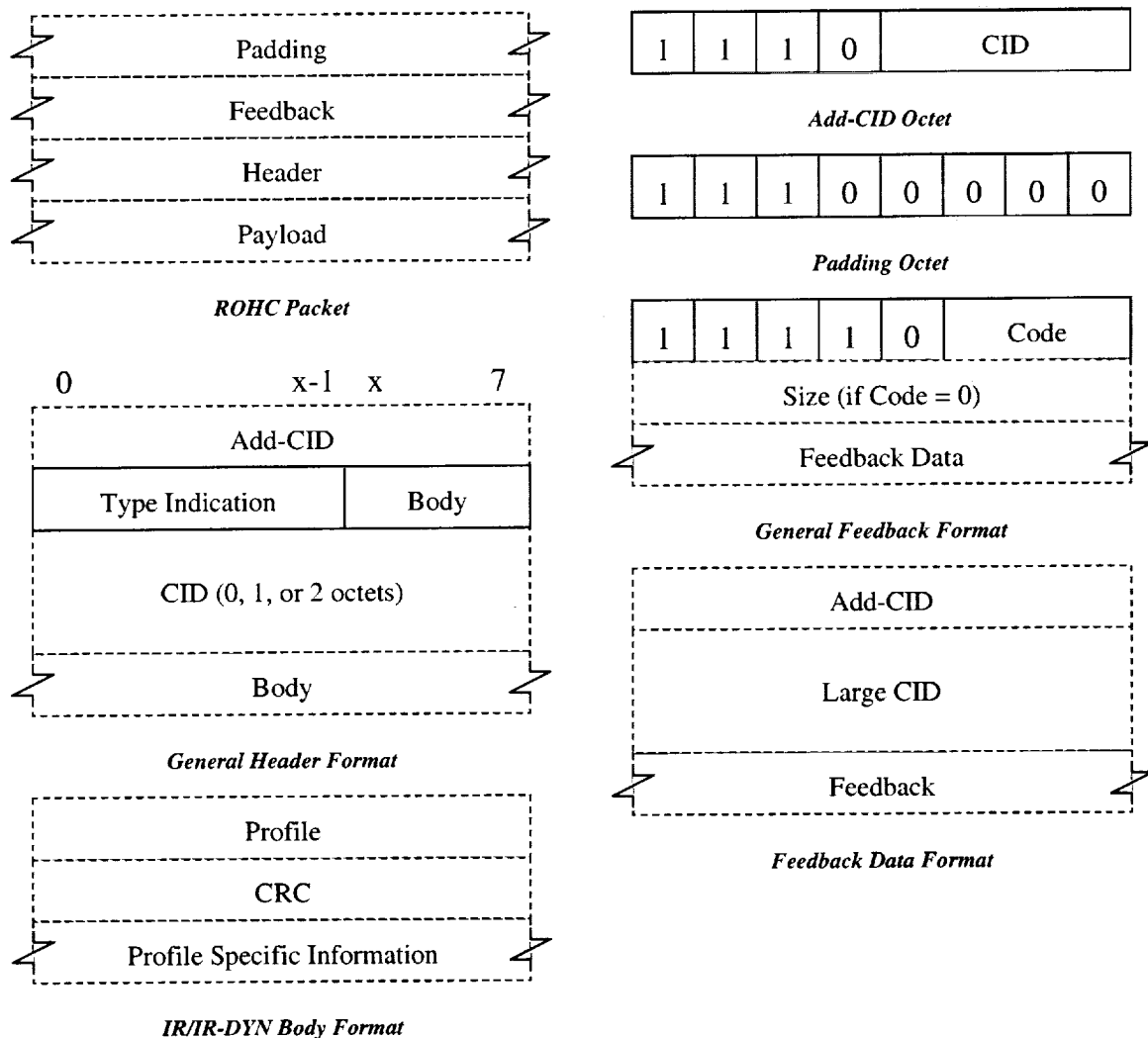
Figure 12: ROHC Framework
