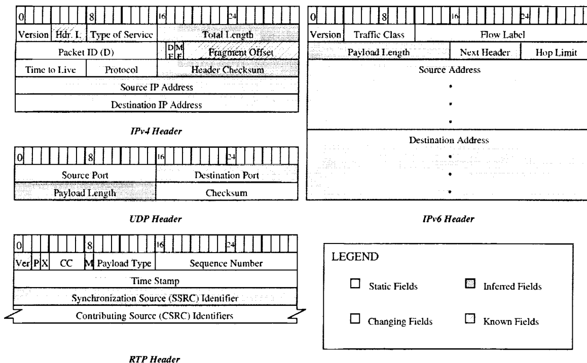
Figure 13: Activity of various protocol headers [ROHC]
