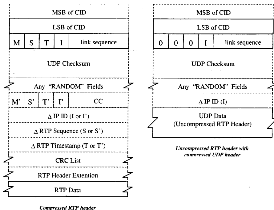
Figure 11: Compressed RTP Header Formats [RFC2508]
