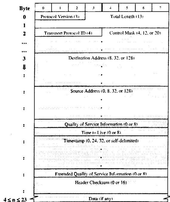
Figure 4: SCPS Network Protocol Header
