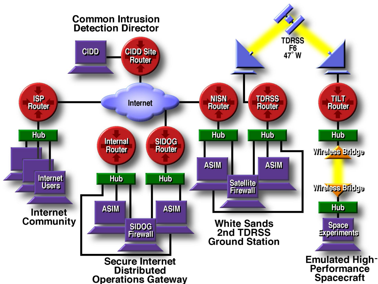
Figure 3.—Security architecture that protected the space-based network.
