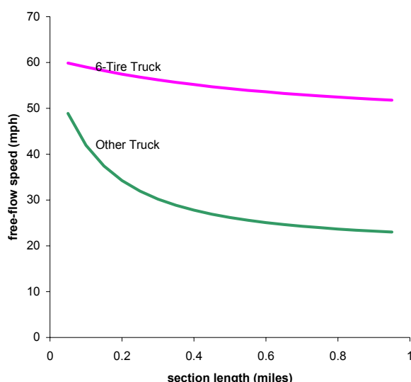
FIGURE 5-9. Grades and speed for trucks.
