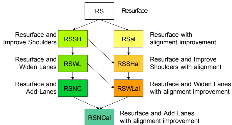
FIGURE 4-4. Resurfacing improvement hierarchy.
