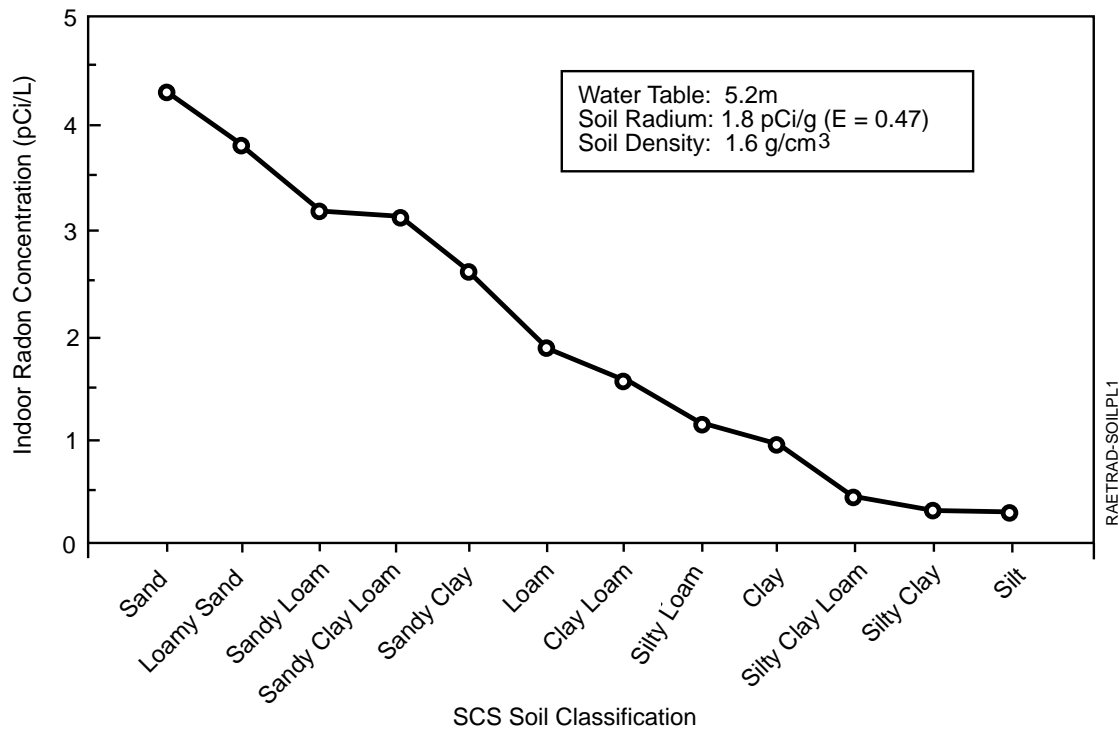
Figure 1. Sensitivity of indoor radon to soil textural class.
