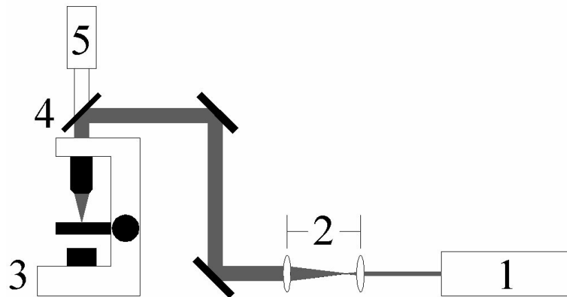
Figure 1. 1. Laser; 2. Beam Expander; 3. Microscope; 4. Dichroic Filter; 5. CCD Camera
