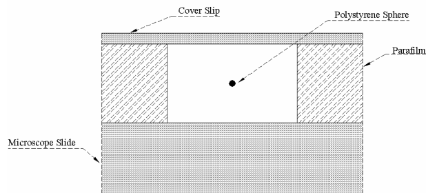
Figure 2. Trapping Well
