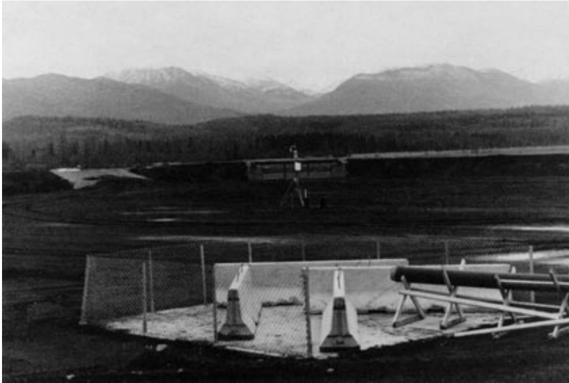
Figure 22. Spoils line outlet pads.
