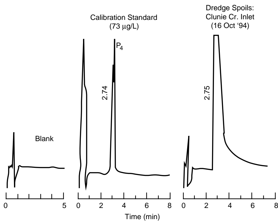
Figure 28. Comparative chromatograms for spoils analysis.
