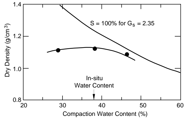
Figure 11. Results of Proctor tests of peaty silt.
