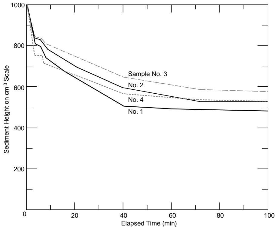
Figure 1. Results of preliminary sedimentation tests.
