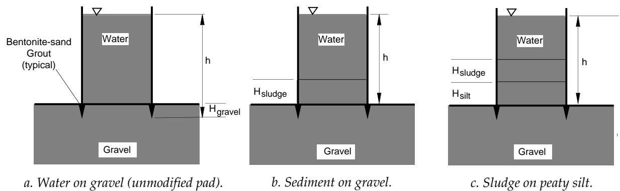
Figure 14. Schematics of barrel tests on EOD pad.
