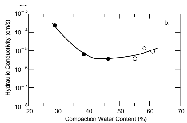
b. Hydraulic conductivity vs. water content.
