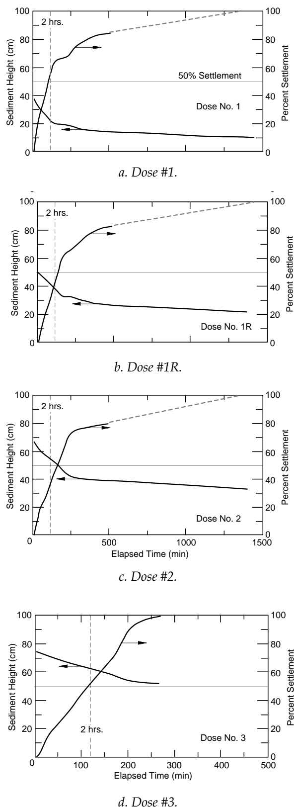
Figure 3. Sedimentation test results in Montgomery tube.
