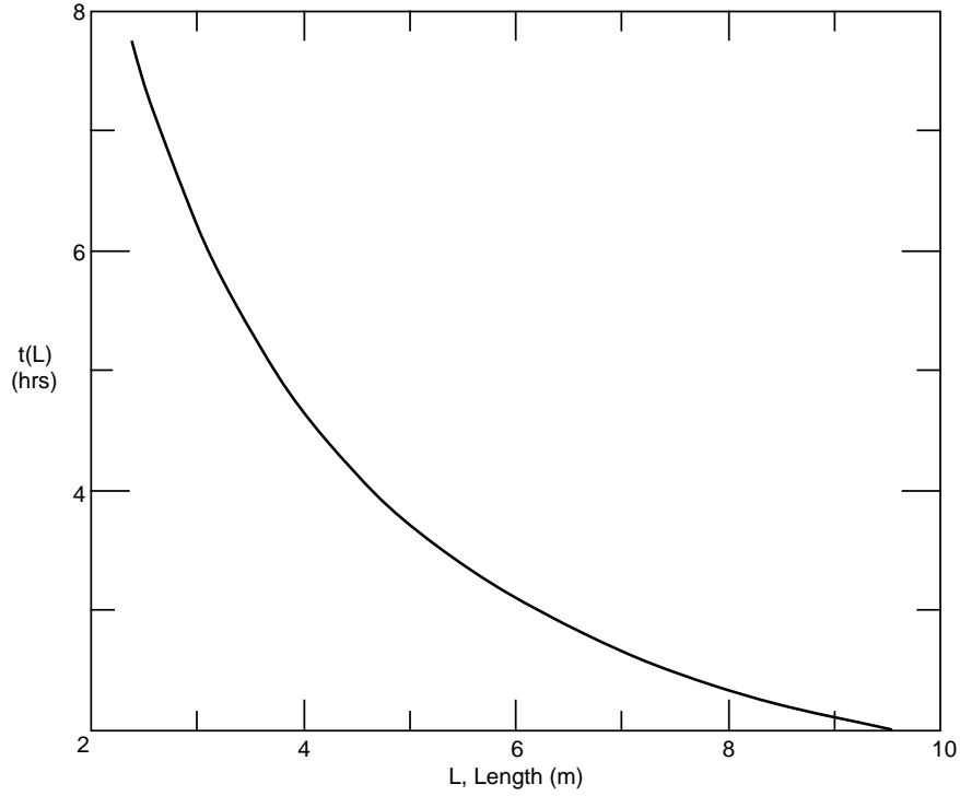
Figure 7. Basin drainage times as a function of weir length.
