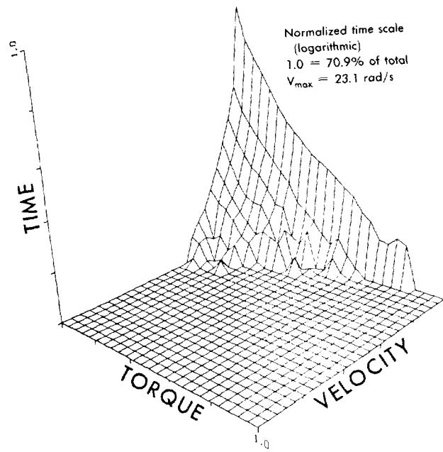
Figure 16. - Mechanical power grid for wrist roll.
