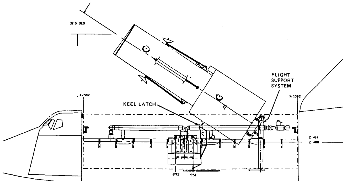
Figure 2. - Stowed/reboost configuration.
