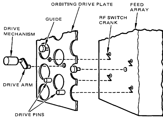
Figure 5. - RF switch positioner concept.
