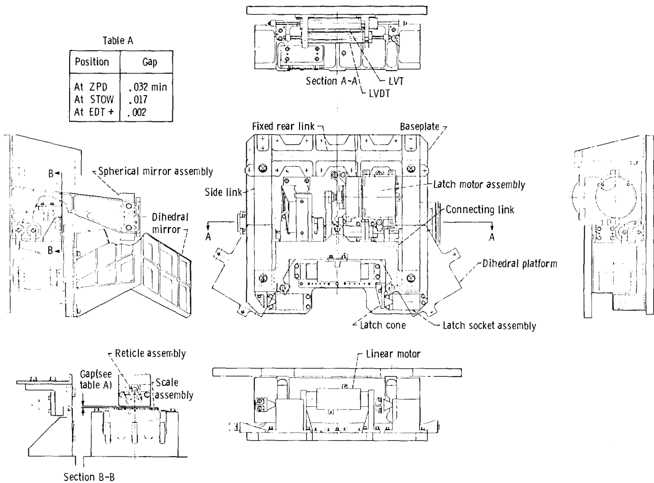
Figure 5. Mirror transport mechanism assembly.
