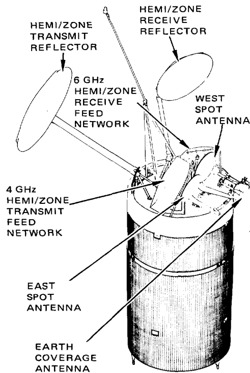
Figure 1. - Antenna farm configuration for INTELSAT VI.
