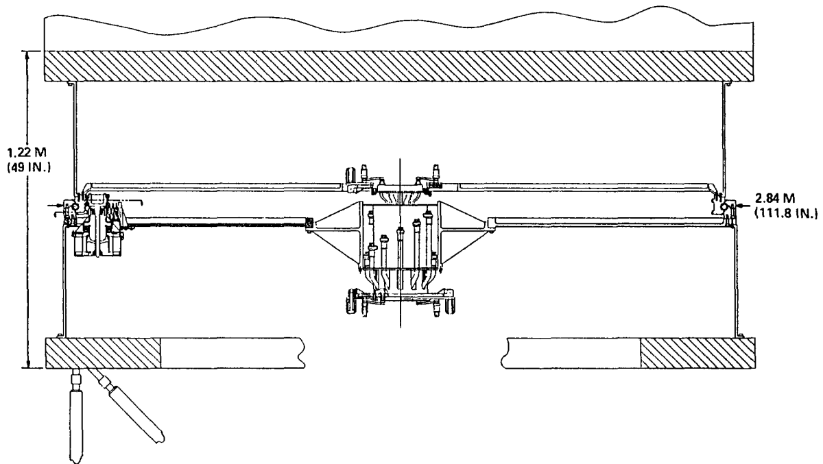
Figure 2. - Solar alpha joint.
