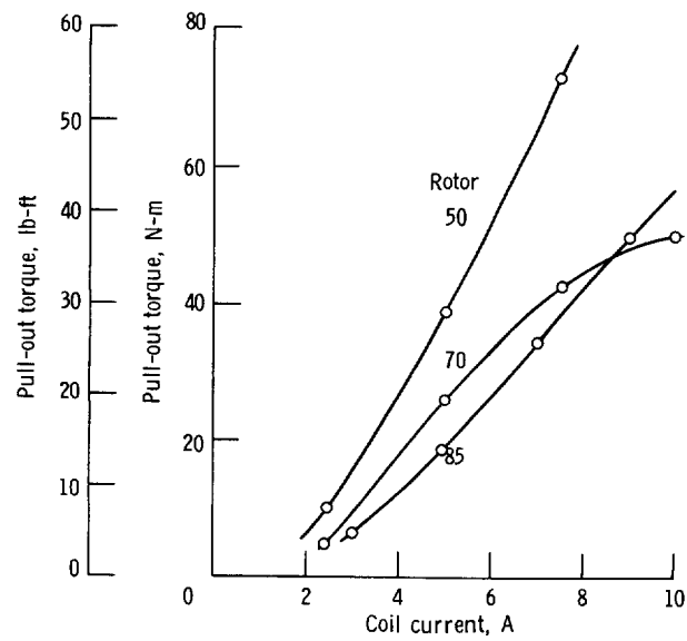
Figure 3. - Static pull-out torque as function of coil current for three test rotors.
