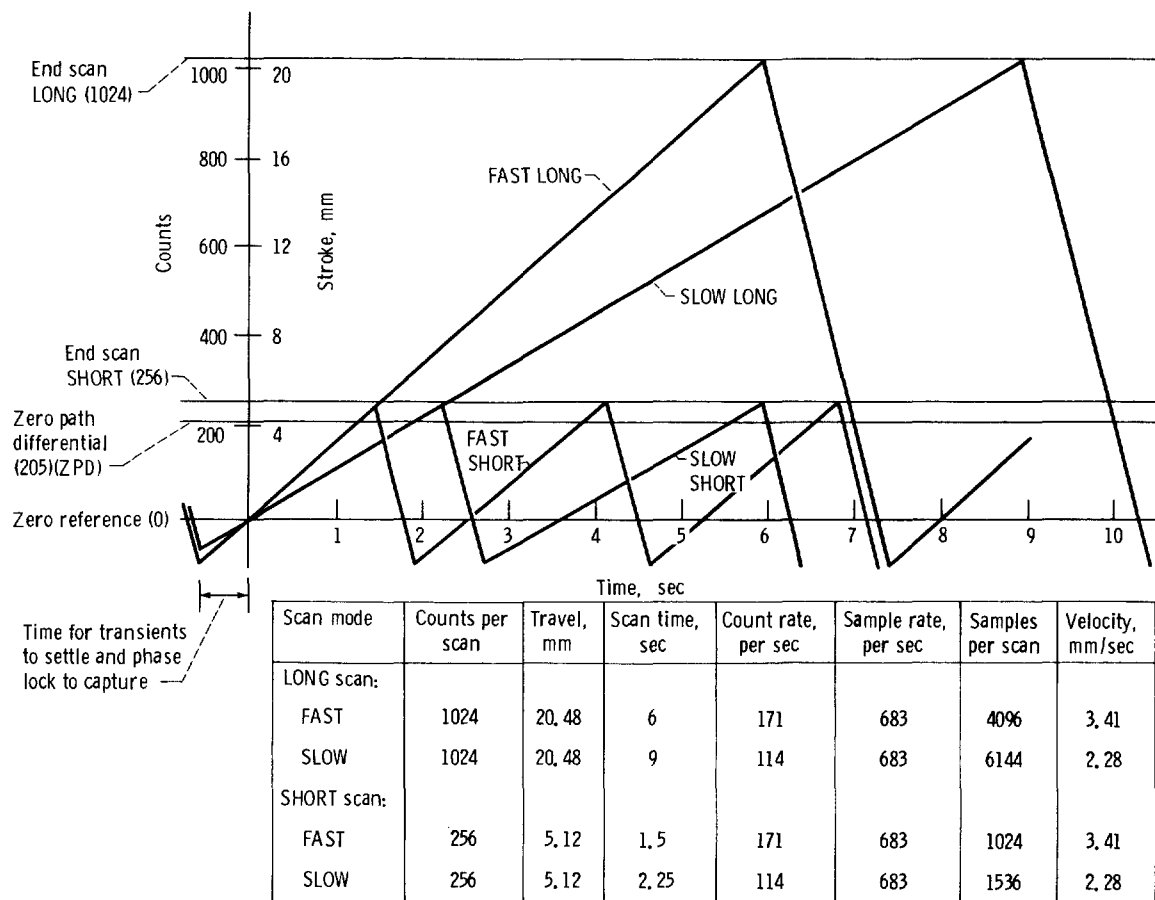
Figure 14. - FIRAS scan modes.
