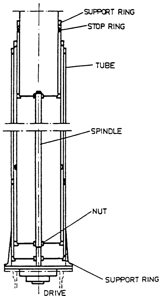
Figure 2. - ERM tube stack and working principle.
