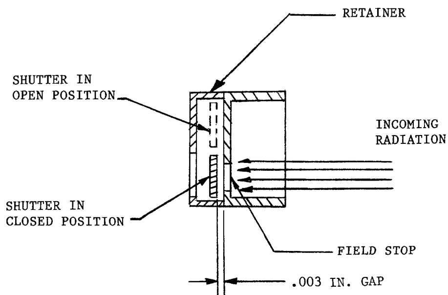
Figure 3. - Photon seal.
