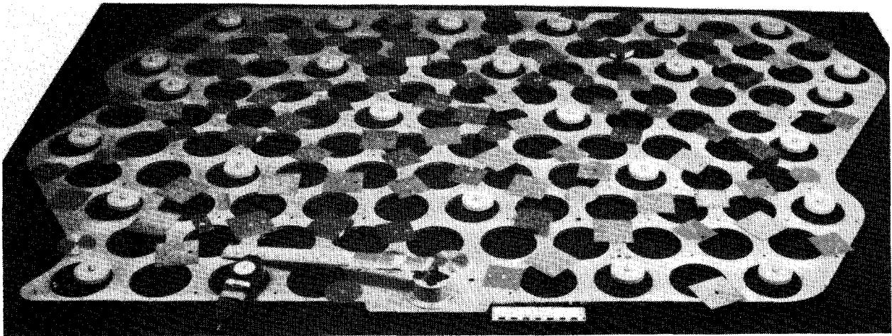
Figure 10. - Simulated thermal gradient test setup.
