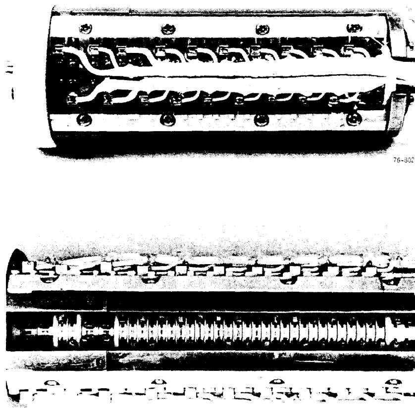
Figure 5. - GPS block 1 slip ring assembly.
