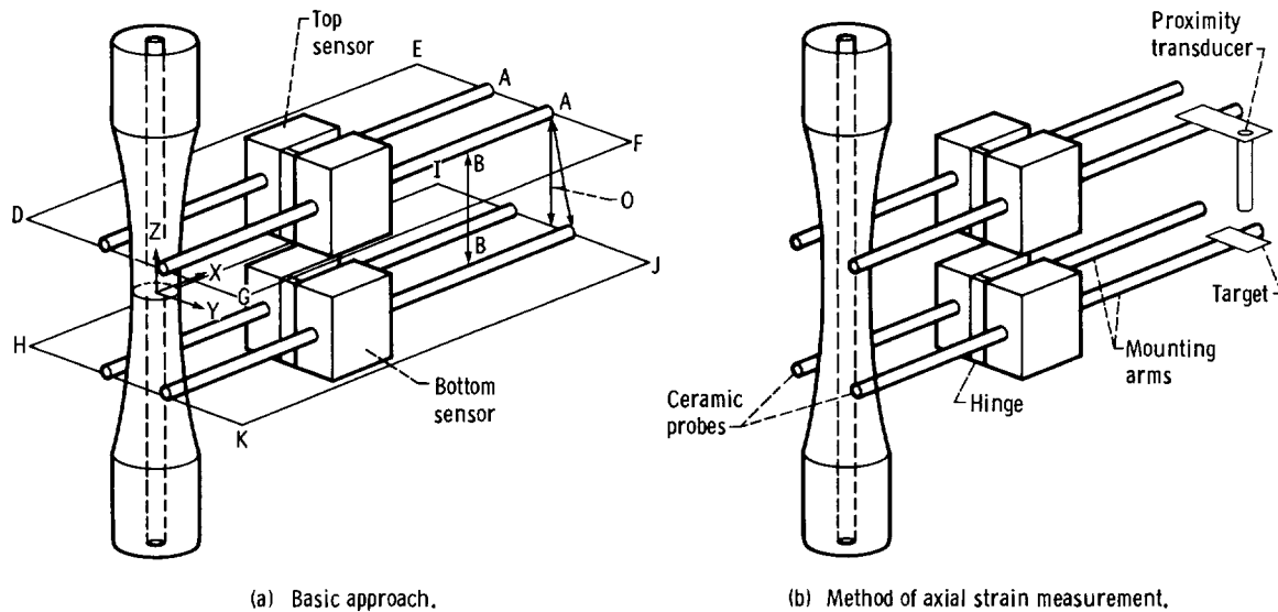
Figure 1. - Multi-axial extensometer for measuring axial, torsional, and diametral strains at elevated temperatures.
