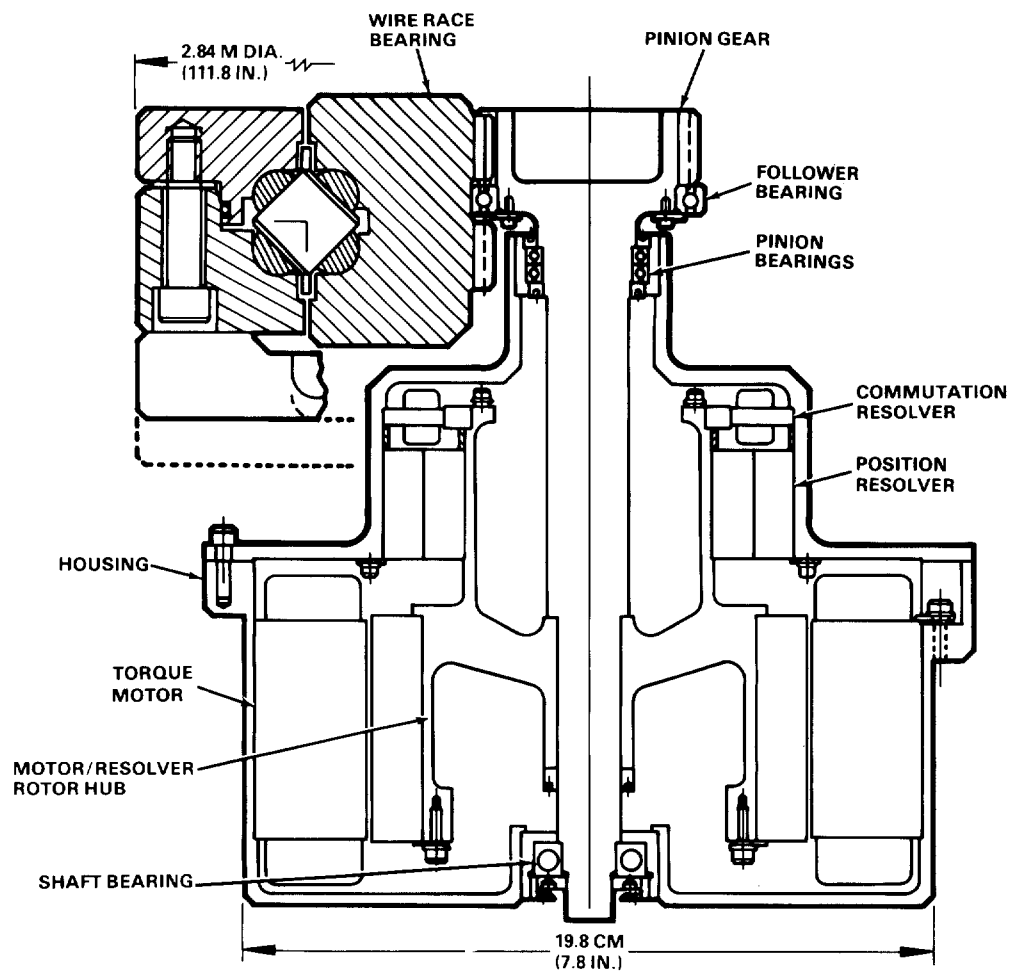
Figure 4. - Drive assembly.
