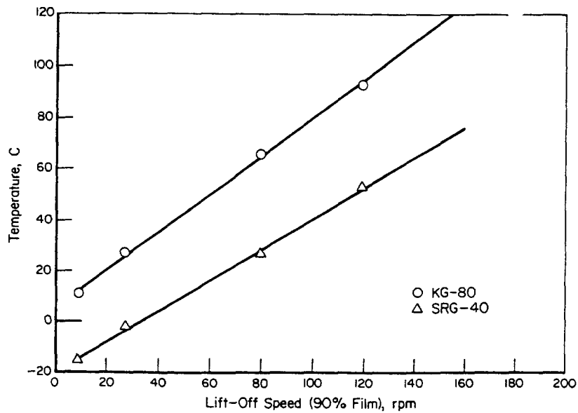
Figure 4. - Lift-off speed as a function of temperature for an R-6 bearing loaded to 980 MN/m 2 maximum Hertzian contact stress (inner race) and lubricated with two super-refined mineral oils.
