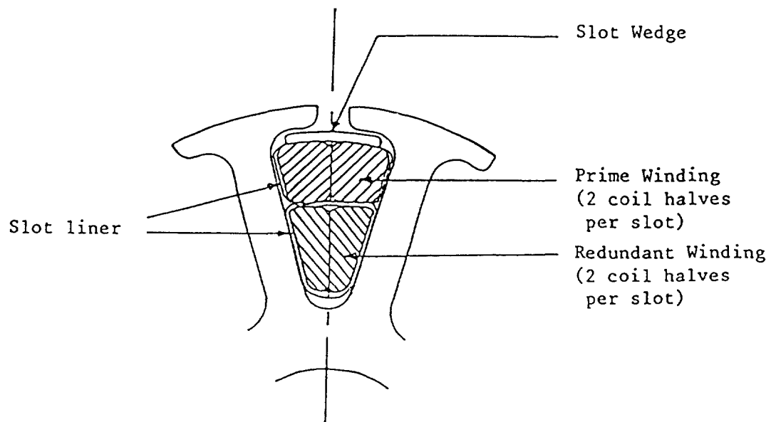
Figure 3. - Winding layout.
