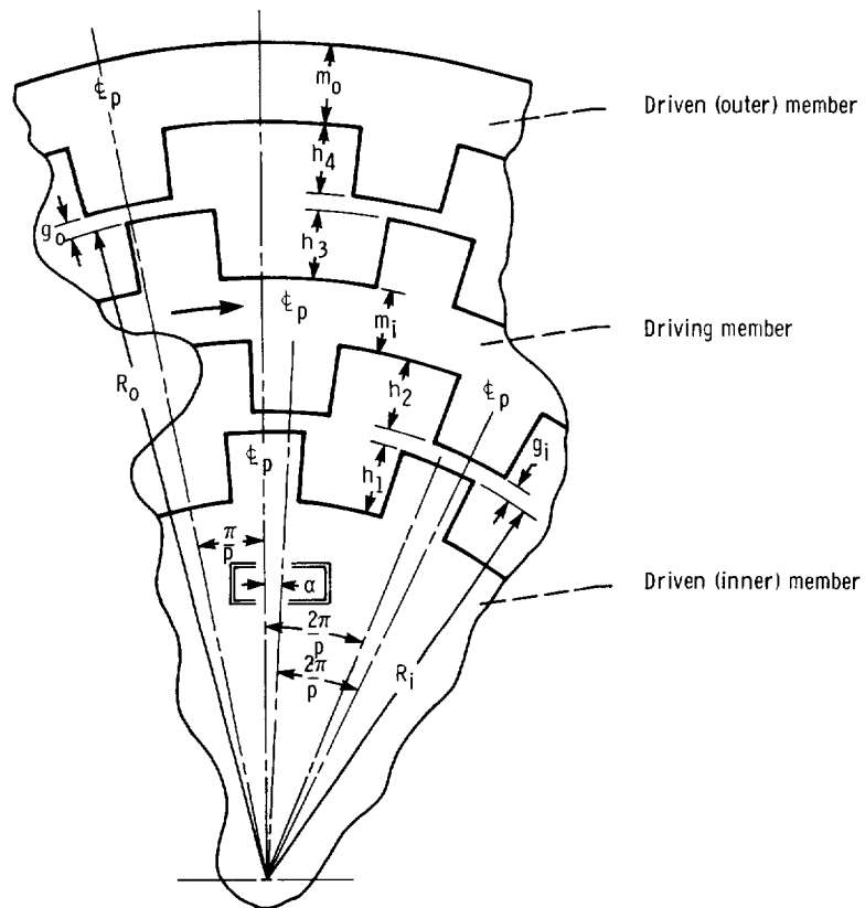
Figure 2. - Geometry of electromagnetic coupling with driven and driving members displaced by \alpha (not at scale).
