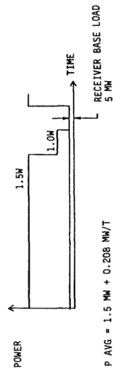
Figure 6. - Absolute, multiplexed encoder simplified block diagram and power profile.
