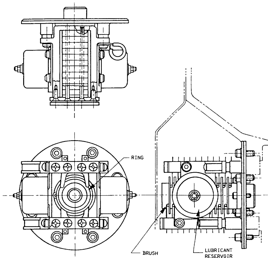
Figure 1. - OS0-6 slip ring assembly.
