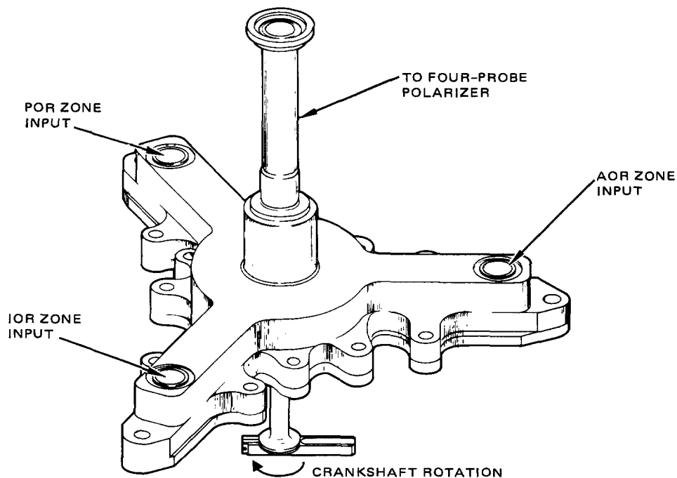
Figure 3. - Squareax switch.
