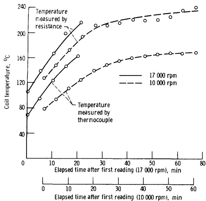
Figure 5. - Heat run; rotor 70 with hermetic seal; current, 10 A; load, 55.7 N-m (41 ft-lb).
