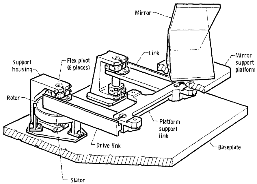
Figure 1. - Original MTM design.
