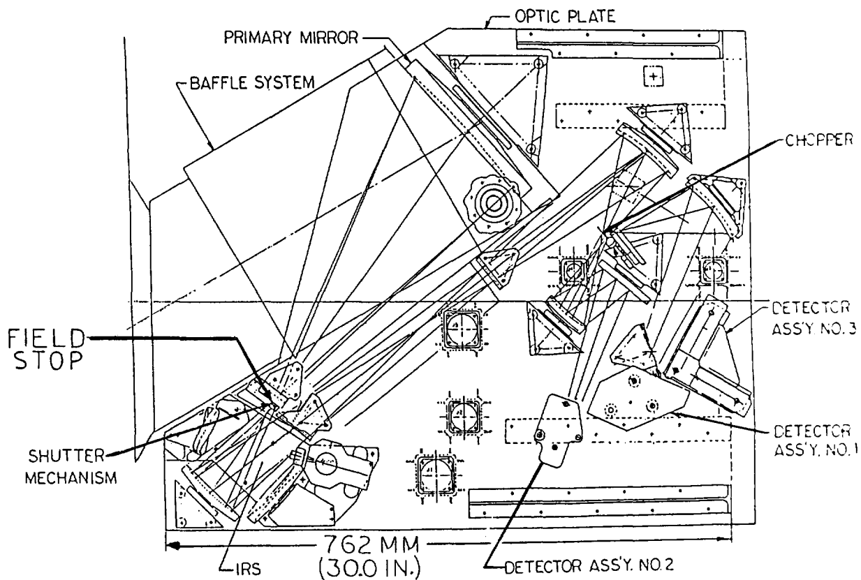
Figure 1. - DIRBE.
