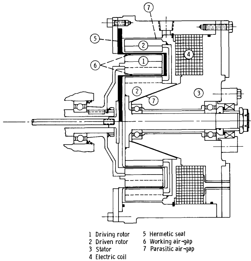
Figure 1. - Electromagnetic coupling.
