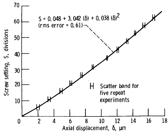
Figure 7. - Evaluation of linear adjustment mechanism.
