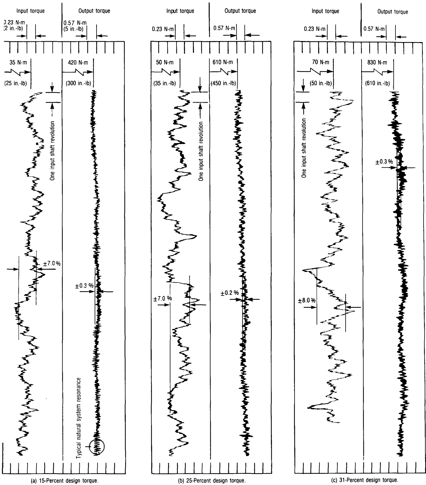
Figure 9. - Effect of torque on roller actuator torque signatures at input speed of 28 rpm. One full output shaft revolution shown for each torque; one input shaft revolution as indicated.
