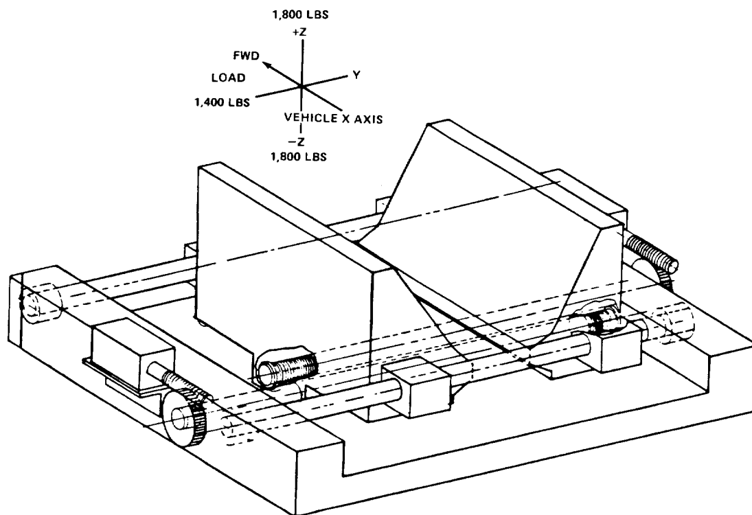
Figure 3. - S. T. keel latch concept.
