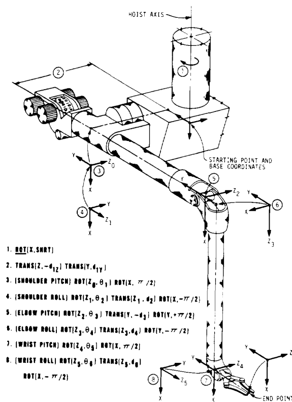
Figure 3. - Manipulator kinematics.
