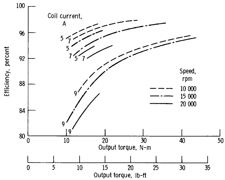
Figure 9. - Efficiency as function of output torque for rotor 85. I^2R losses are not included.
