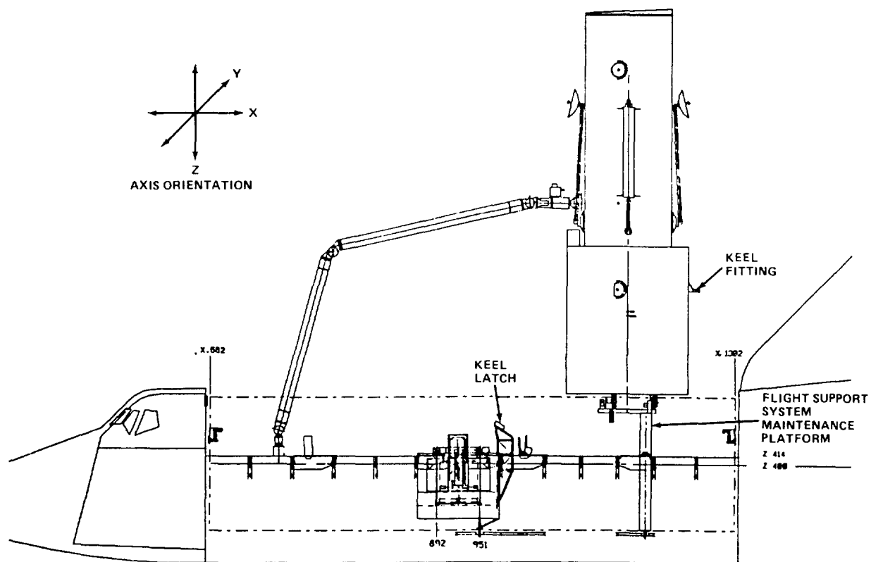
Figure 1. - Berthing configuration.
