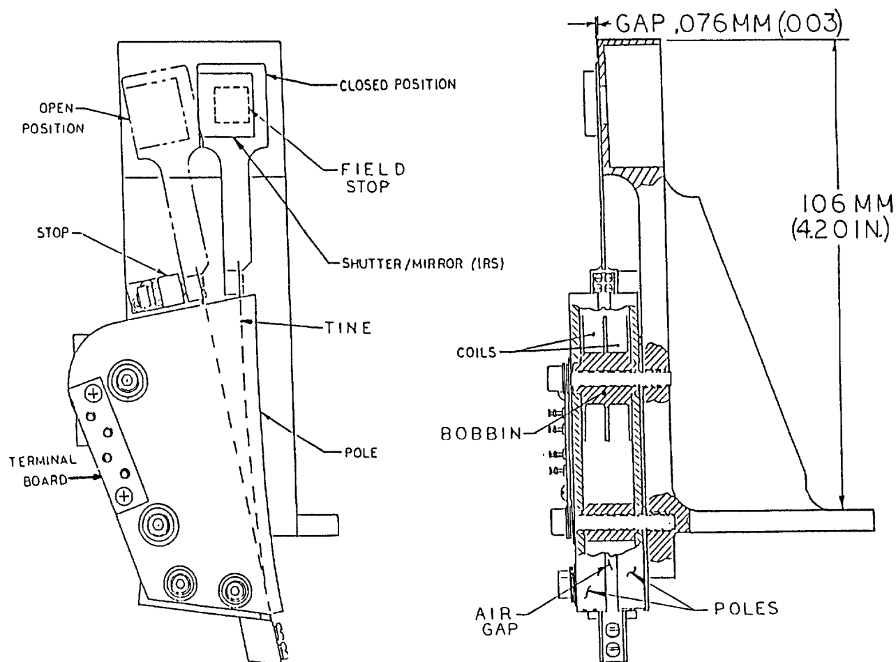
Figure 2. - Shutter mechanism.
