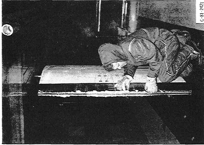
Figure 3. - NACA 63 2 -A415 wing section mounted in Icing Research Tunnel.
