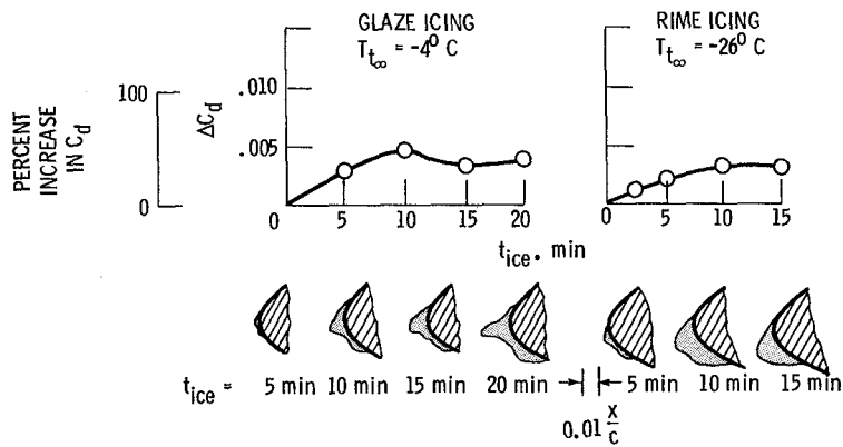
Figure 10. - Comparison of glaze and rime icing for climb conditions V_{\infty} = 40\text{ m/sec} (90 mph), \alpha = 6.6^{\circ} , \text{LWC} = 1.5\text{ gm/m}^3 .
