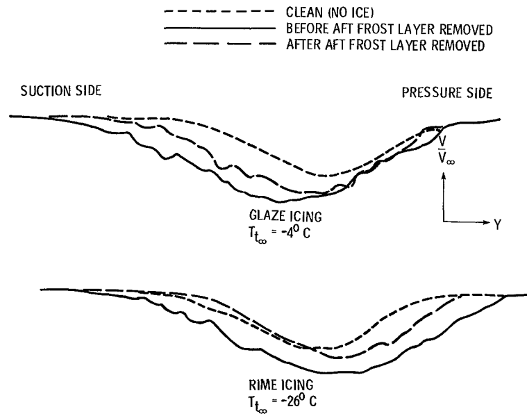
Figure 8. - Wake velocity profiles V_\infty = 51 \text{ m/sec} (115 mph), \alpha = 2.6^\circ , \text{LWC} = 1.5 \text{ gm/m}^3 , t_{\text{ice}} = 10 \text{ min} .
