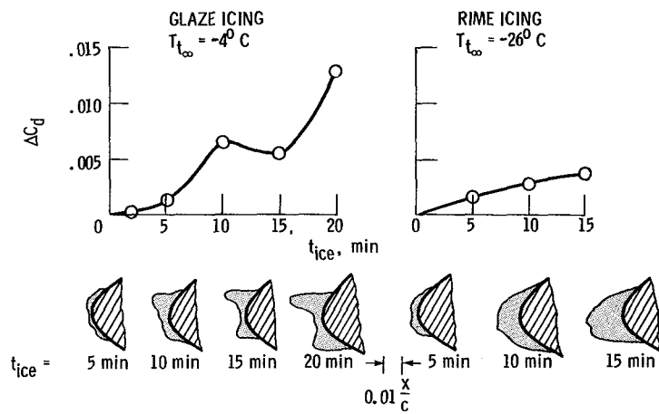
Figure 9. - Comparison of glaze and time icing for cruise conditions V_{\infty} = 5\text{ m/sec} (115 mph), \alpha = 2.6^{\circ} , \text{LWC} = 1.5\text{ gm/m}^3 .
