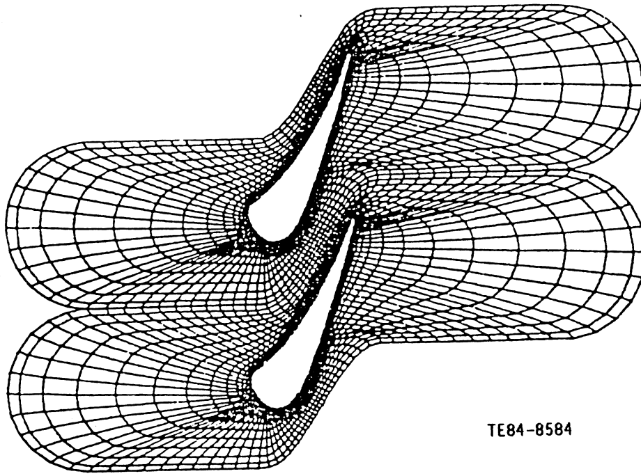
Figure 5. 0-type grid coordinate system for C3X cascade.
