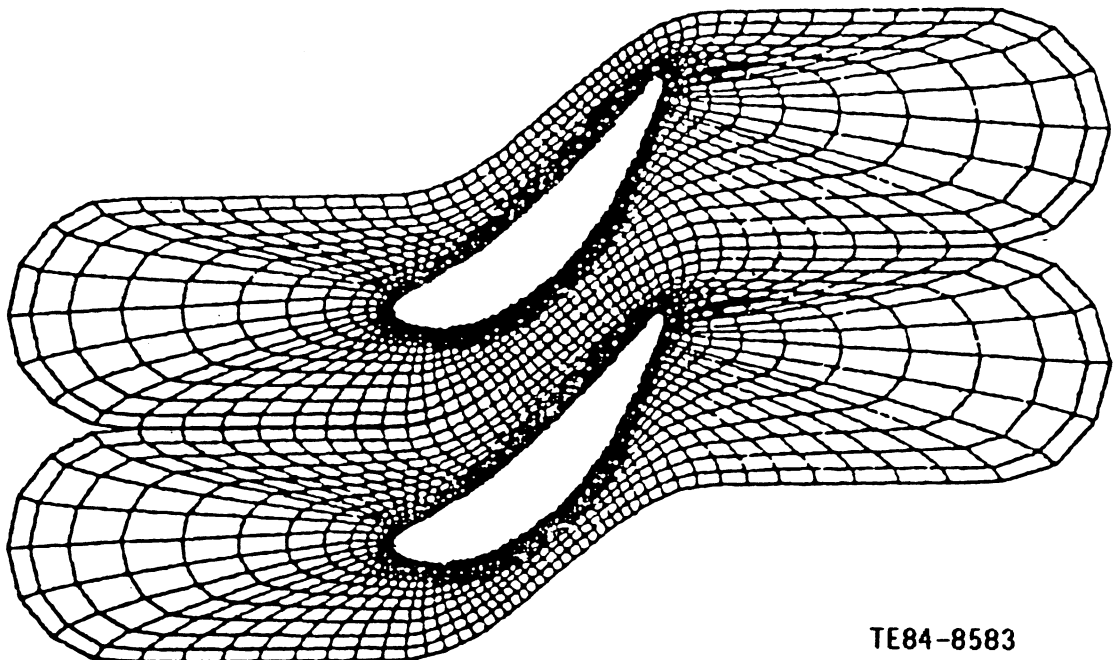
Figure 4. O-type grid coordinate system for Turner cascade.
