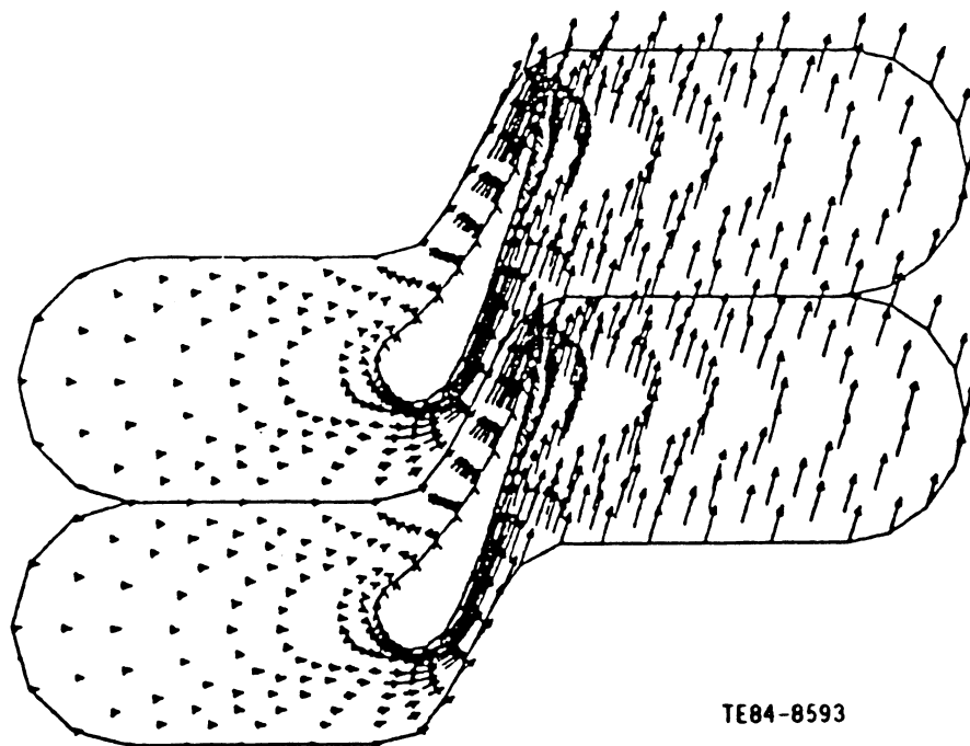
Figure 14. Vector plot for C3X cascade, case 144.
