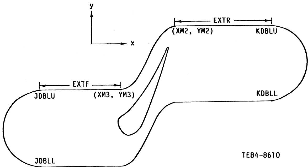
Figure 32. Cascade geometry.
