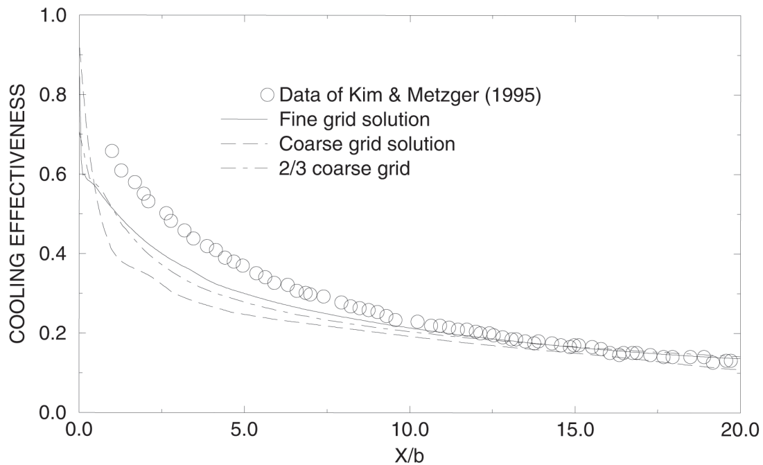
Fig. 16 Spanwise averaged cooling effectiveness (Ameri & Rigby, 1999)
