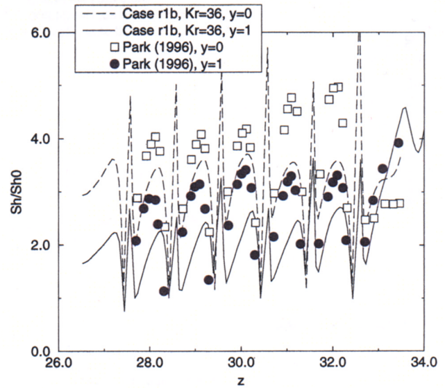
Fig. 36 Spanwise averaged Sherwood number in the second leg for the case rot36 (Rigby, 1998)
