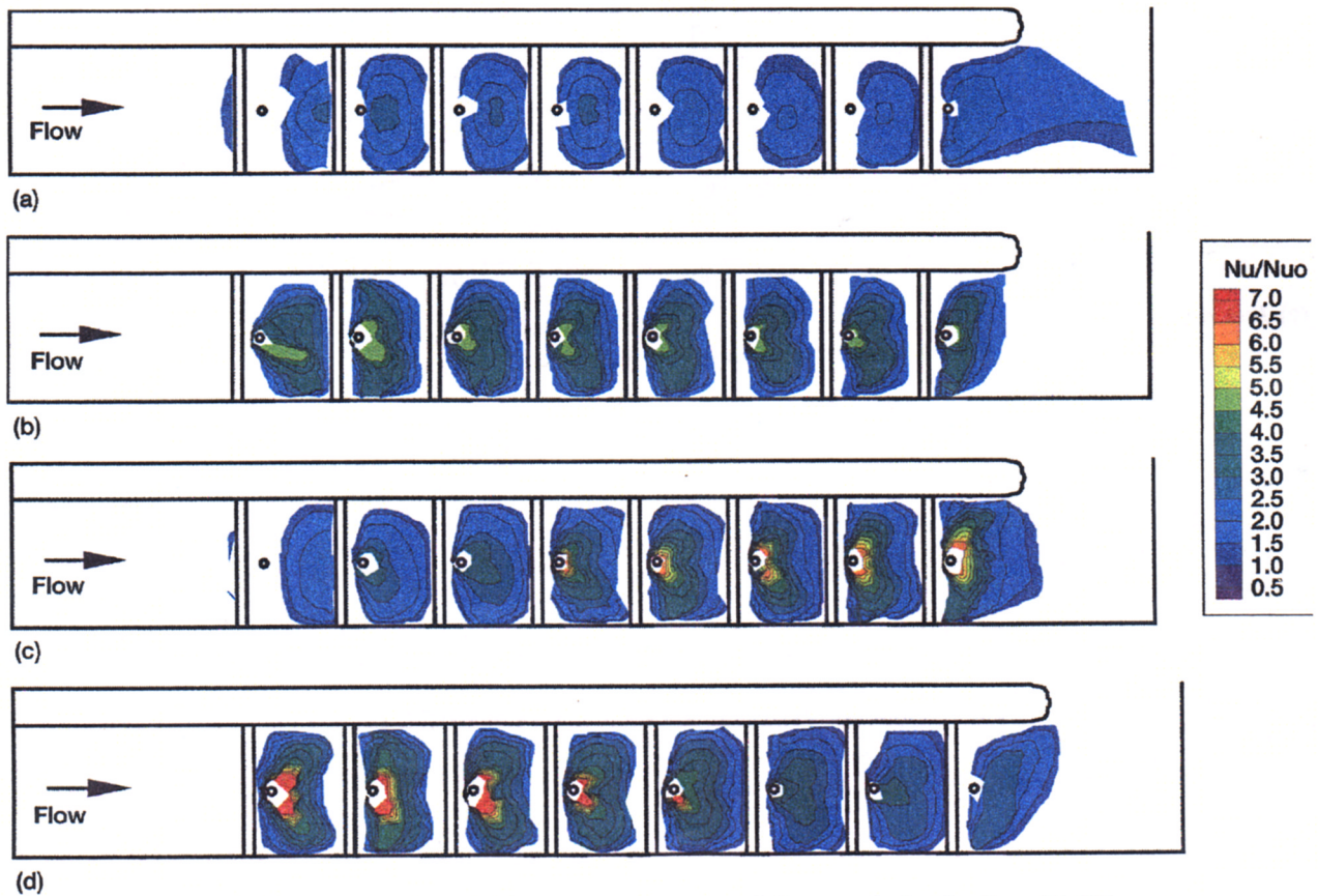
Fig. 37 Surface heat transfer, Nu/N_{uo} , for the case of ribs near holes for Re = 31,000 . (a) no bleed; (b) uniform bleed; (c) increasing bleed; (d) decreasing bleed (Thurman and Poinsatte, 2001)
