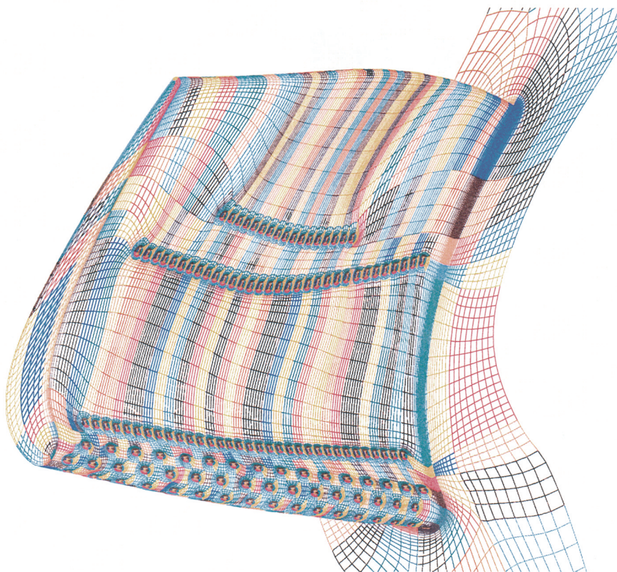
Fig. 25 Grid on the blade tip & pressure side, and a part of the hub (Garg, 2000)
