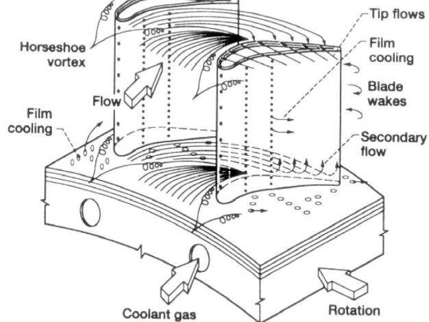
Fig. 1 Complex heat transfer phenomena in the turbine gas path
