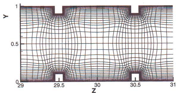
Fig. 33 Grid in the plane x = 0 (Rigby, 1998)
