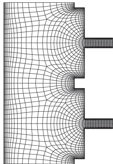
Fig. 31 Grid in the symmetry plane (Rigby et al., 1997a)
