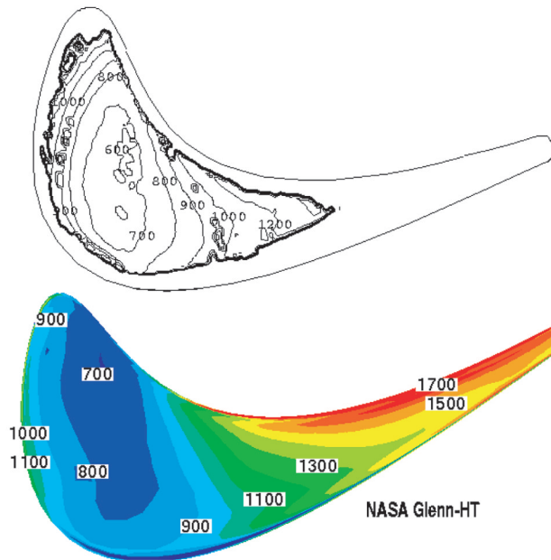
Fig. 13 Radiused edge tip heat transfer coefficient ( \text{W/m}^2 \text{K} ) for clearance of 2.03 mm and T_u = 5\% (Ameri & Bunker, 2000)
