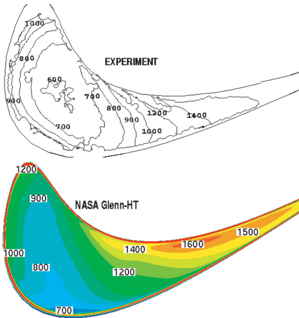
Fig. 12 Sharp edge tip heat transfer coefficient ( \text{W/m}^2 \text{K} ) for clearance of 2.03 mm and T_u = 5\% (Ameri & Bunker, 2000)
