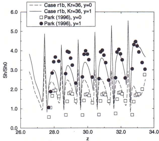
Fig. 35 Spanwise averaged Sherwood number in the first leg for the case rot36 (Rigby, 1998)
