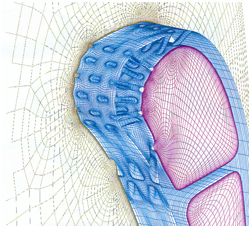
Fig. 22 Leading edge region of the computational grid (Heidmann et al., 2000)
