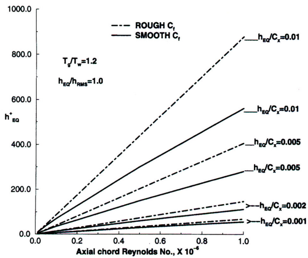
Fig. 38 Estimated maximum equivalent roughness height (Boyle et al., 2001)
