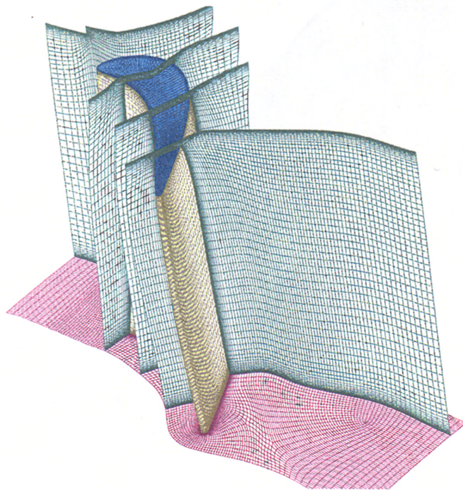
Fig. 8 Overall grid features for the GE-E 3 blade (Ameri et al., 1999)
