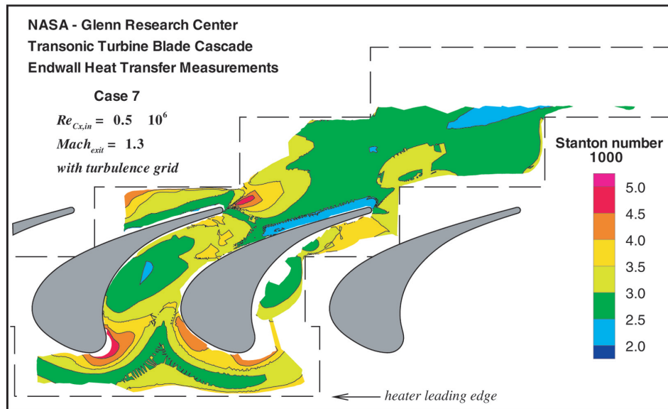
Fig. 5 Endwall Stanton number distribution (Giel et al., 1998)
