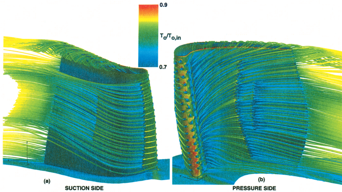
Fig. 27 Streamlines, colored by temperature, emanating from holes over the cooled blade surface with distribution of h (Case 1; grid on blade tip) (Garg, 2000)
