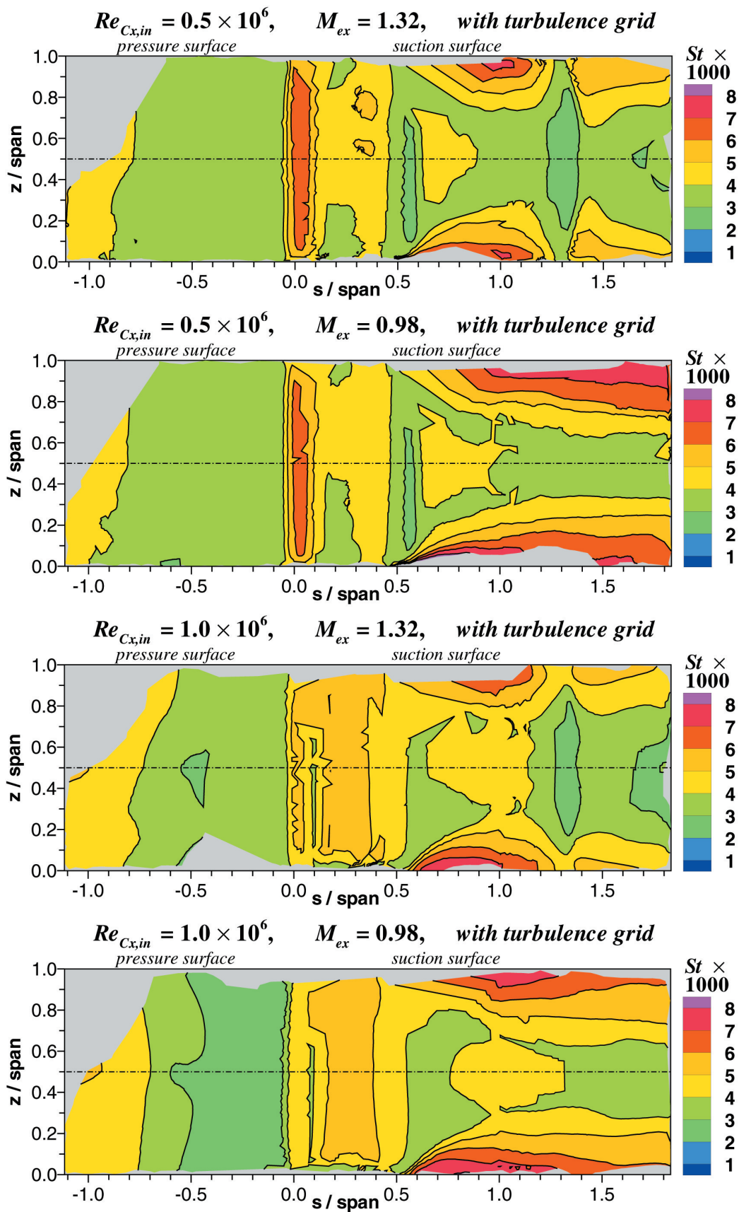
Fig. 4 Measured Stanton number \times 1000 on the blade surface (Giel et al., 1999)
