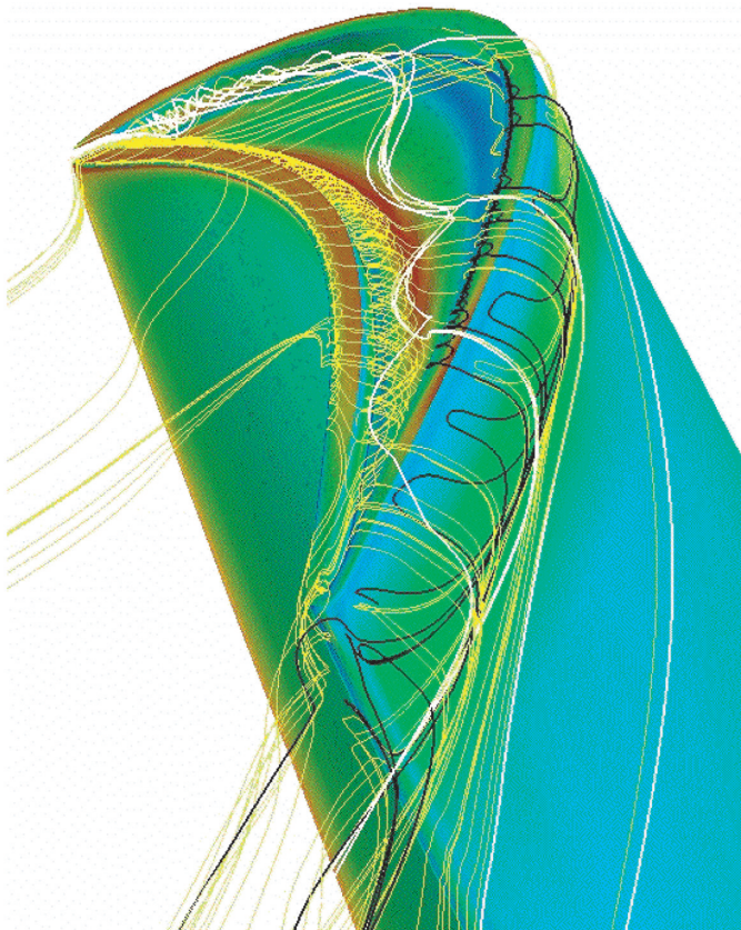
Fig. 6 Streamlines showing the blade tip flow patterns (Ameri et al., 1998)
