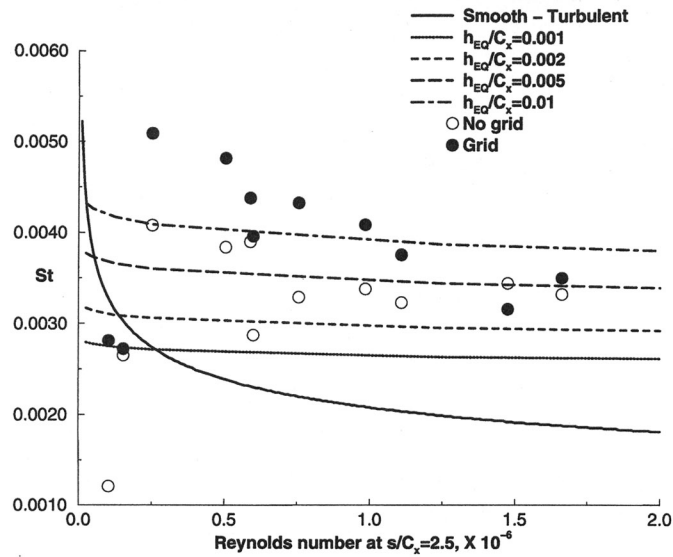
Fig. 41 Stanton number at s/C_x = 2.5 (Boyle et al., 2001)
