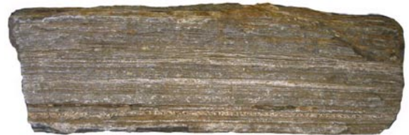
Layered gneiss from along San Lorenzo Creek in Santa Cruz County.
