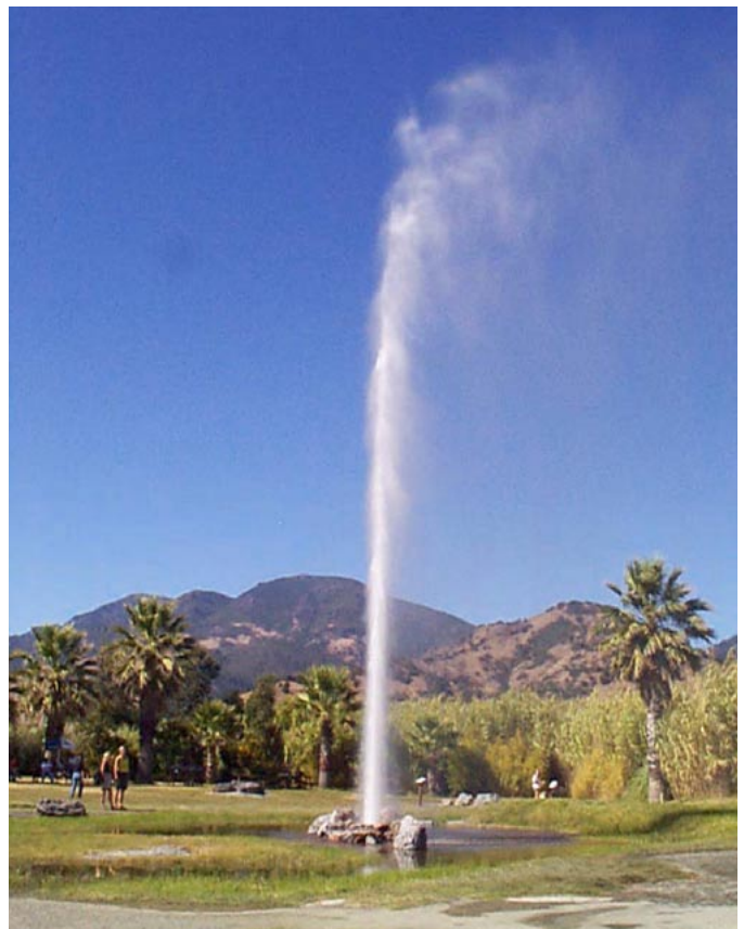
The Calistoga Geyser (Old Faithful Geyser of California) in northern Napa Valley, evidence that the Sonoma volcanic field is still relatively young and hot.
