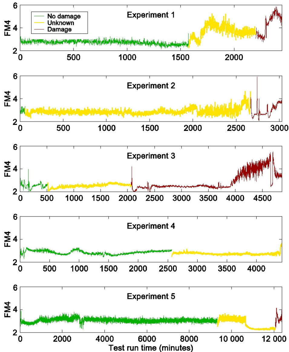
Figure 3.—FM4-spur rig experiments 1 through 5.
