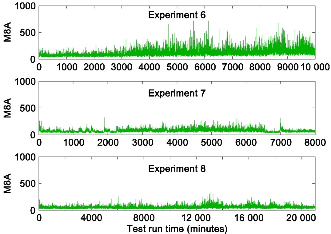
Figure 6.—M8A-spur rig experiments 6 through 8.
