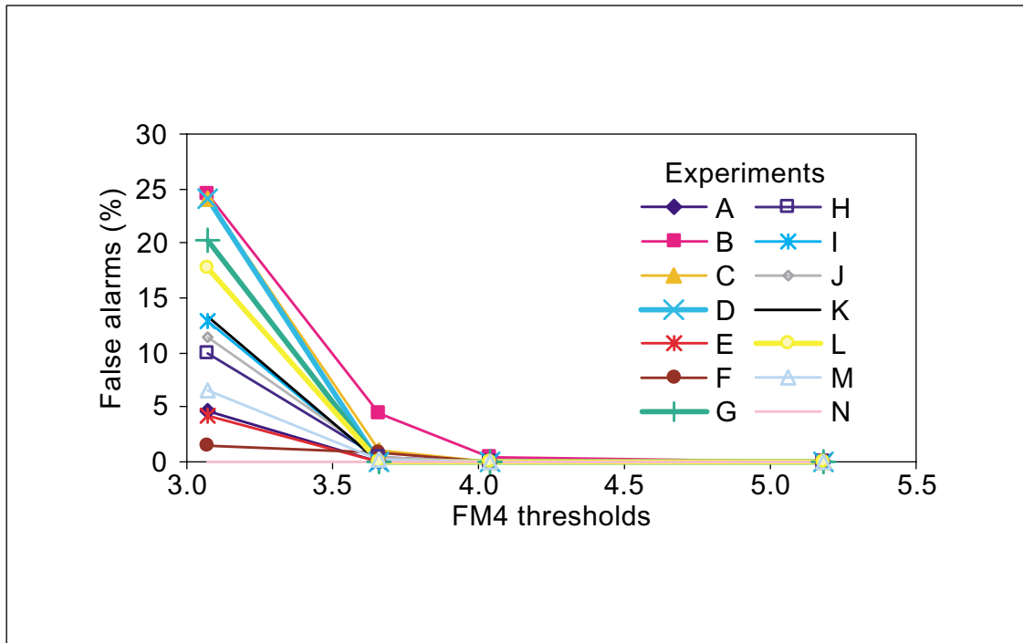
Figure 10.—FM4 false alarm rates-OH58 flight experiments maneuvers A through N.
