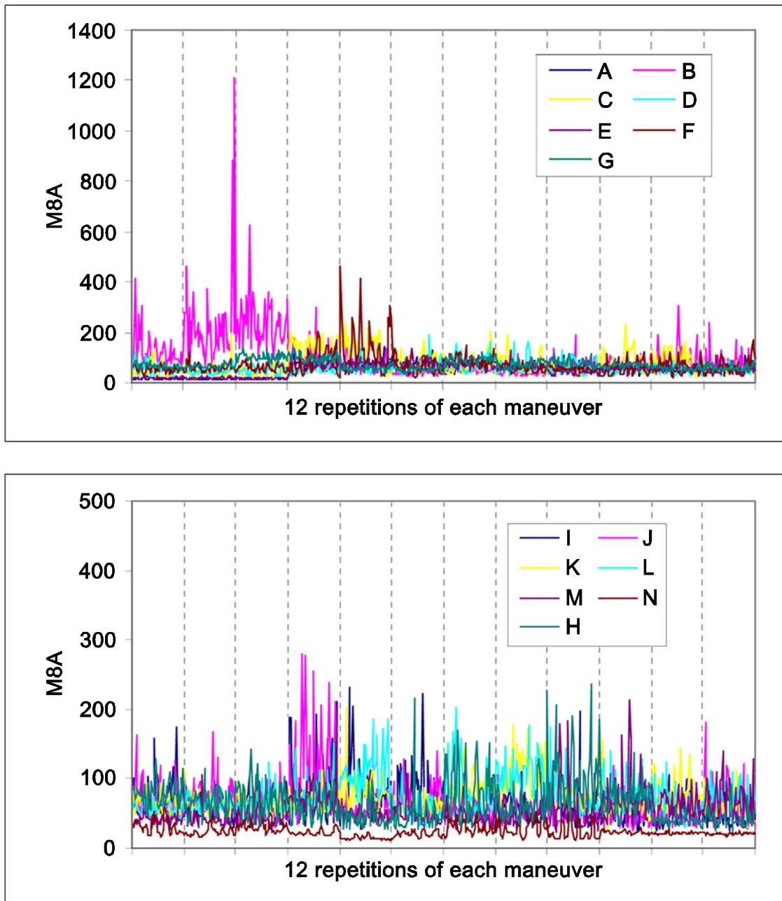
Figure 8.—M8A-OH58 flight experiments maneuvers A through N.
