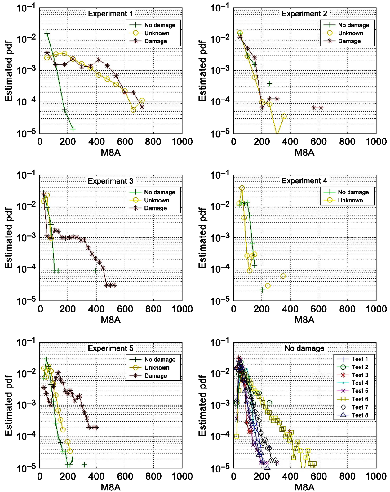
Figure 12.—Estimated probability distribution functions of M8A from GRC test rig experiments.
