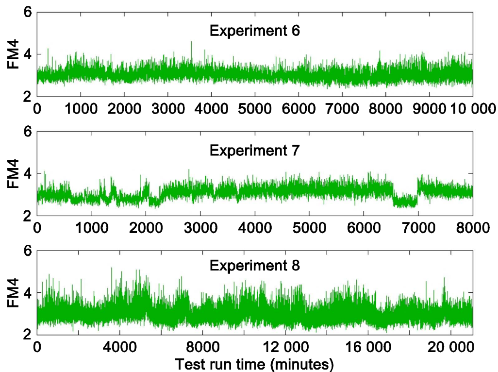
Figure 5.—FM4-spur rig experiments 6 through 8.
