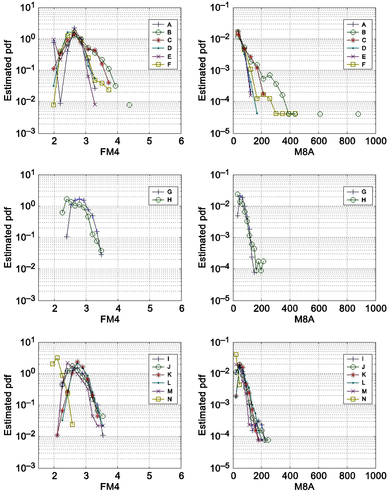
Figure 13.—Estimated probability distribution functions of FM4 and M8A from ARC flight test.
