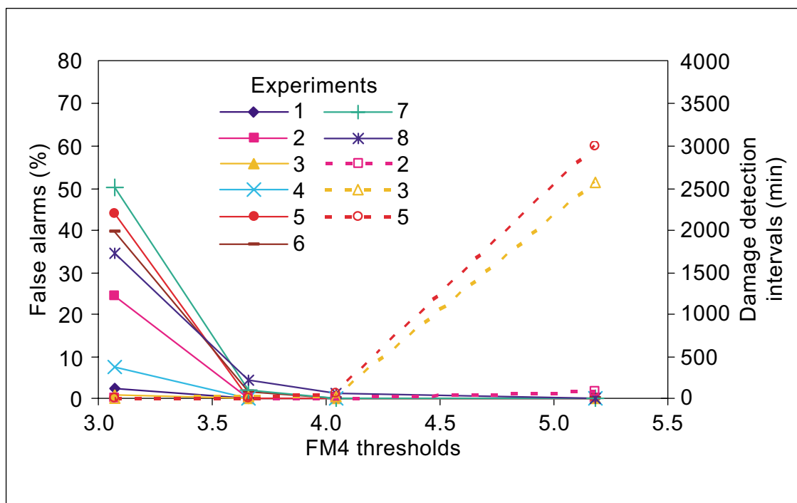
Figure 9.—FM4 false alarm rates and damage detection intervals for spur rig experiments 1 through 8.
