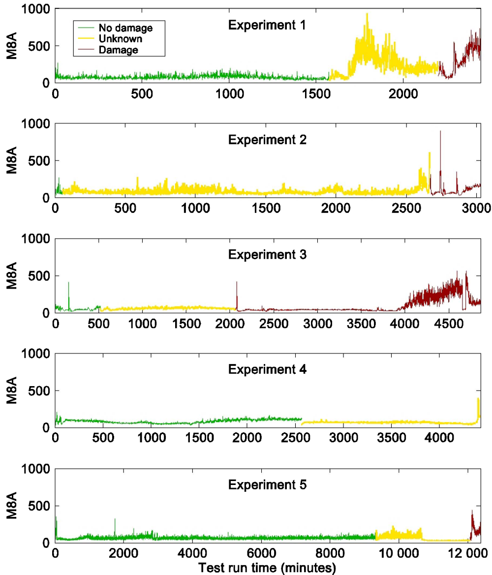
Figure 4.—M8A-spur rig experiments 1 through 5.
