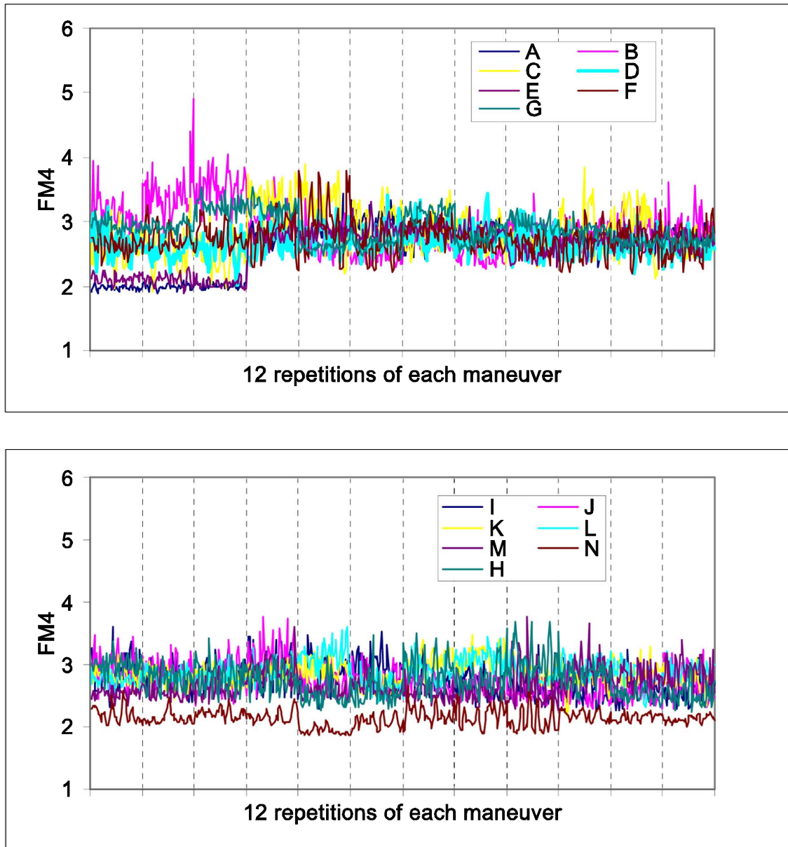
Figure 7.—FM4-OH58 flight experiments maneuvers A through N.
