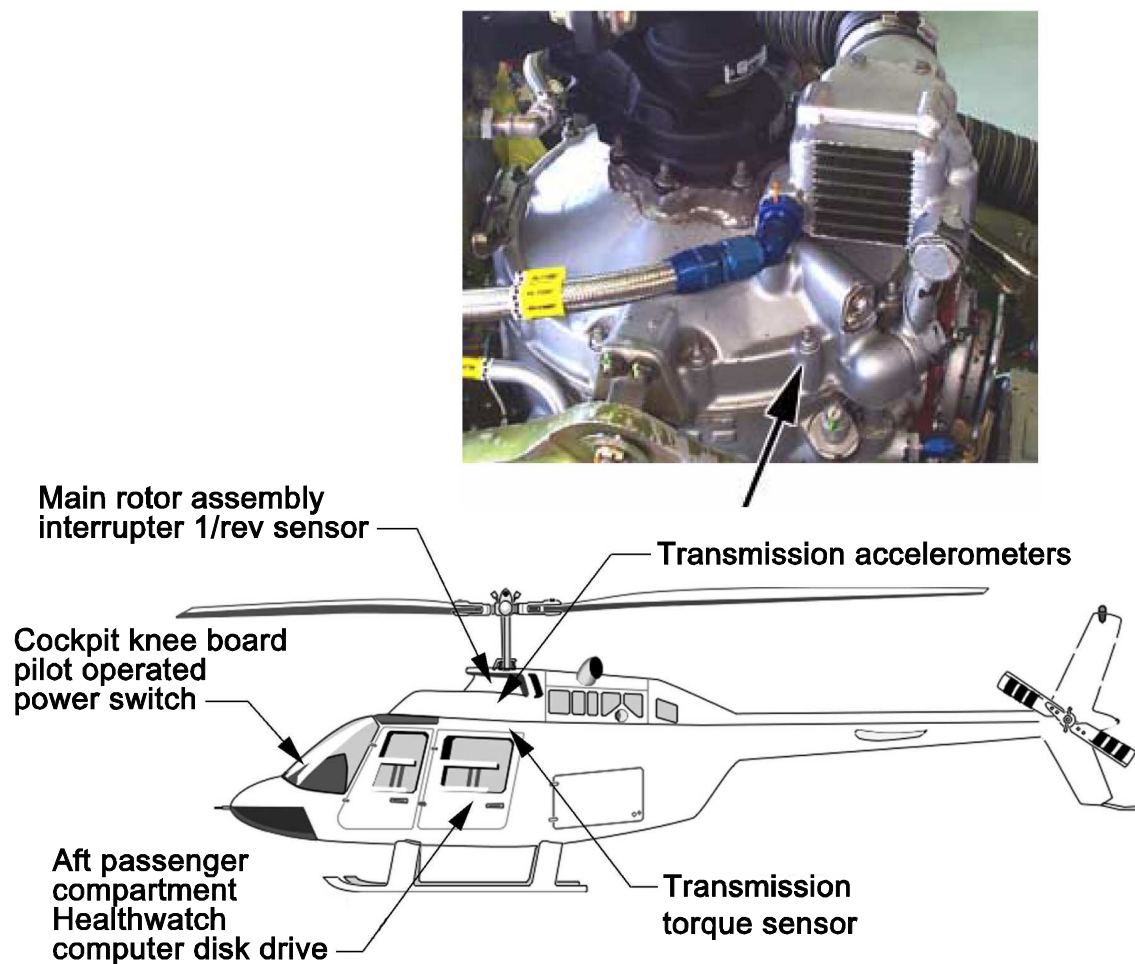
Figure 2.—Accelerometer a6 location on OH58 helicopter.
