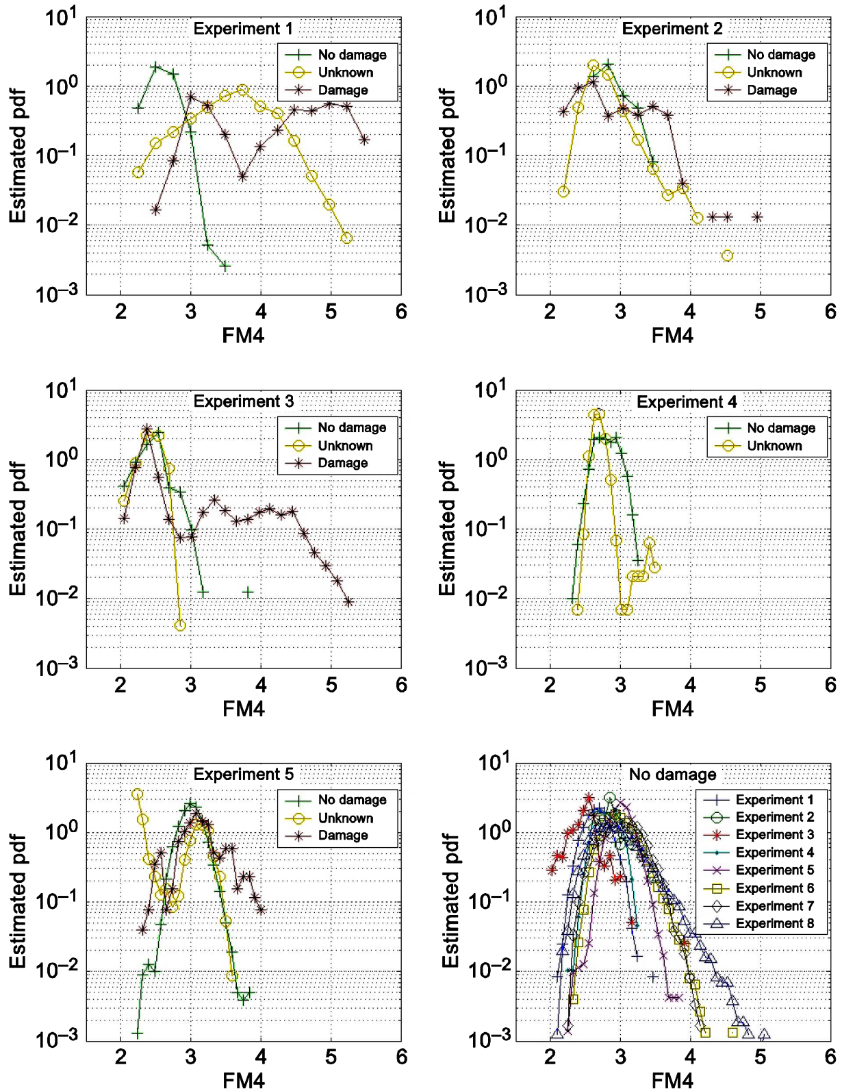
Figure 11.—Estimated probability distribution functions of FM4 from GRC test rig experiments.
