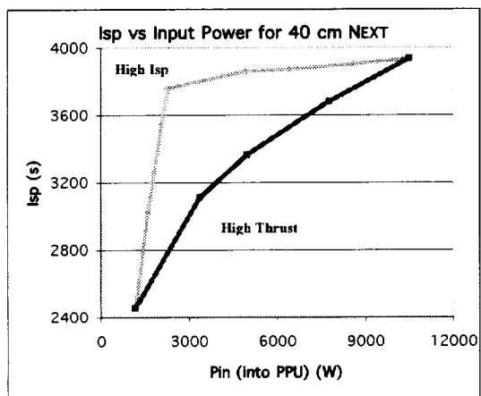
Figure 2. High I_{sp} and High Thrust Throttle Fits
