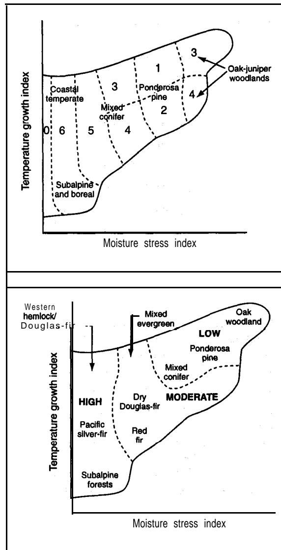
Figure 2-Fire regimes in Pacific Northwest vegetation types can be defined by physical characteristics of the disturbance (0=little fire influence, 1-infrequent light surface fire [ >25 yr], 2=frequent light surface fire [1-25 yr], 3=infrequent severe surface fire [ > 25 yr], 4= short return interval crown fire and severe surface fire [25-100 yr], 5=long return interval crown fire and severe surface fire [100-300 yr], 6=very long return interval crown fire and severe surface fire [ >300 yr]). From Agee (1993; granted with permission from "Fire Ecology of Pacific Northwest Forests," Agee, © Island Press, Aug.13, 1998. Published by Island Press, Washington, DC, and Covelo, CA).
