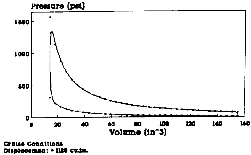
Figure 6.11 Pressure vs. Volume Diagram 960 Hp Engine
