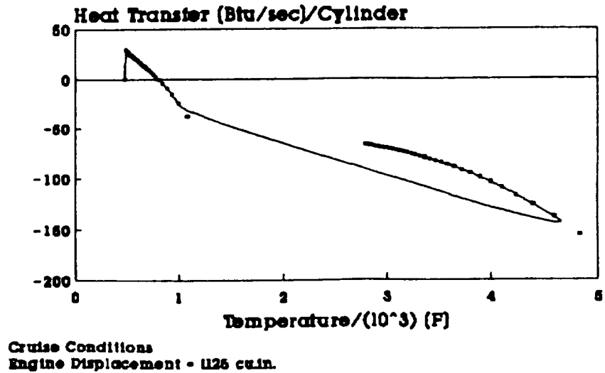
Figure 6.12 Heat Transfer vs. Temperature 960 Hp Engine
