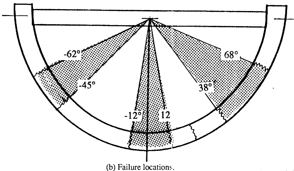
Figure 18. - Comparison of nondimensional analytical moment distribution predicted by finite element frame model and observed failure locations on metal and composite fuselage components and structures.
