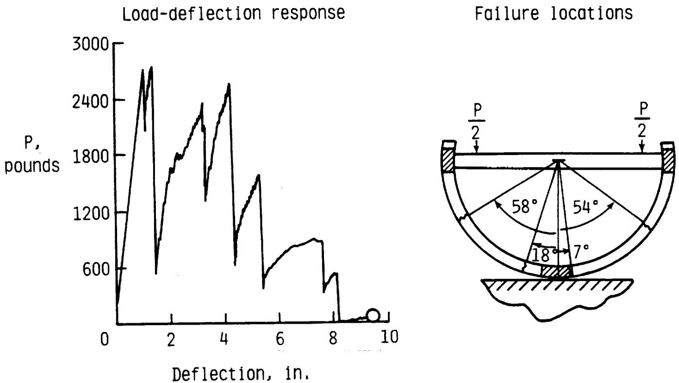
(b) Load-displacement and failure locations.
