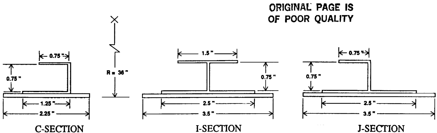
(a) Cross-sectional dimensions.
