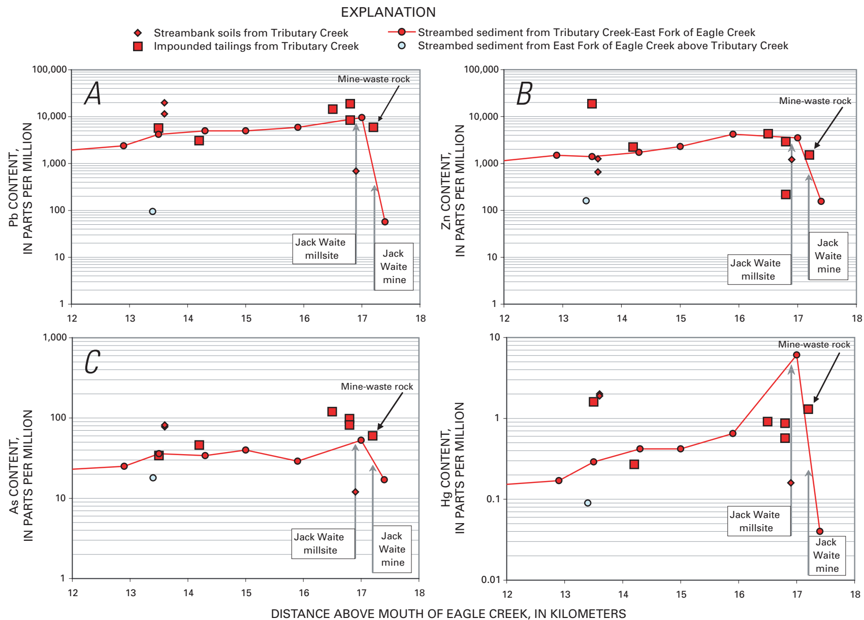
Figure 13. Pb (A), Zn (B), As (C), and Hg (D) contents in fine (<0.063-mm grain size) fraction of samples of streambed sediment, streambank soil, and artificial-fill material (impounded tailings except where noted) collected from Tributary Creek and immediately downstream segment of the East Fork of Eagle Creek in the northern Coeur d’Alene Mining District, northern Idaho (fig. 4), versus distance upstream from mouth of Eagle Creek, with locations of the Jack Waite (Pb-Zn) Mine and its ore-concentration mill along stream labeled.
