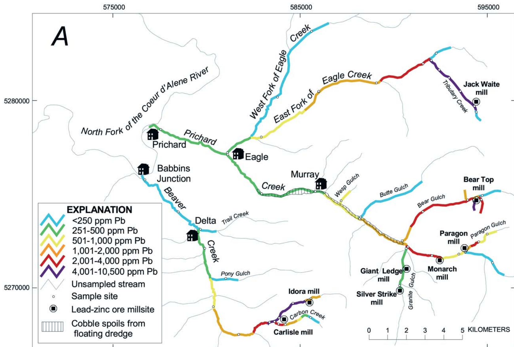
Figure 9. Prichard Creek, Eagle Creek, and Beaver Creek drainages in the northern Coeur d'Alene Mining District, northern Idaho (figs. 1, 2), showing ranges of Pb (A), Zn (B), As (C), and Hg (D) contents in fine (<0.063-mm grain size) fraction of streambed sediment along segments of streams, extrapolated from measured values at discrete sampling sites. Locations of stream-segment boundaries were interpolated from measured values at discrete sampling points or extrapolated to tributary junctions by inferred relations to either metal-poor or metal-enriched inflowing tributaries. Locations of major lead-zinc ore millsites, the source of a significant proportion of metal-enriched sediment, are also shown. Background values, based on samples from the unimpacted West Fork of Eagle Creek: Pb, 82 \pm 16 ppm; Zn, 113 \pm 15 ppm; As, 11 \pm 1 ppm; Hg, 0.06 \pm 0.01 ppm.
