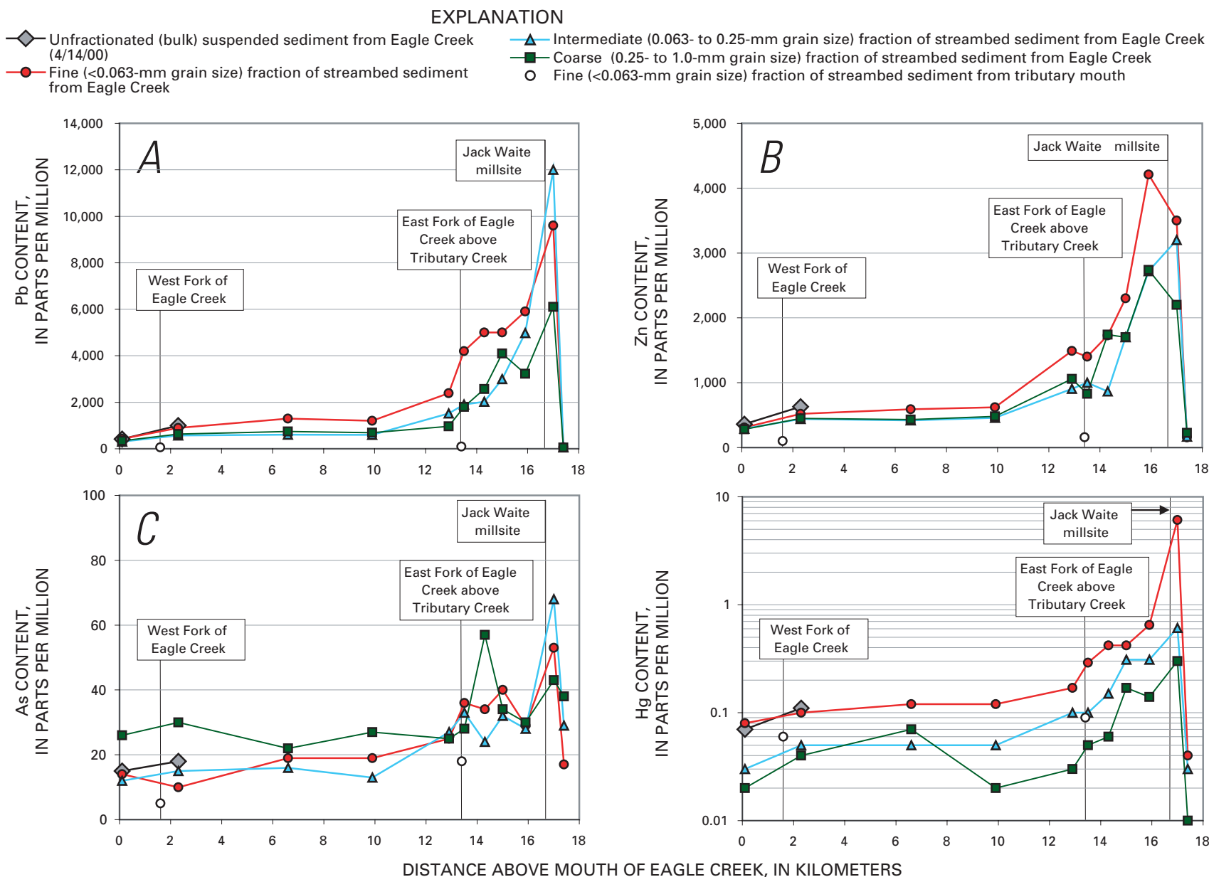
Figure 12. Pb (A), Zn (B), As (C), and Hg (D) contents in three grain-size fractions of samples of streambed sediment and in samples of unfractionated (bulk) suspended sediment collected from the Eagle Creek drainage basin in the northern Coeur d'Alene Mining District, northern Idaho (figs. 1, 2), versus distance upstream from mouth of Eagle Creek, beginning (at right) at head of Tributary Creek and continuing down the East Fork of Eagle Creek to mouth of main stem of Eagle Creek. Data points for fine (<0.063-mm grain size) fraction of streambed sediment from tributaries to Eagle Creek are plotted at confluence of tributary and Eagle Creek.
