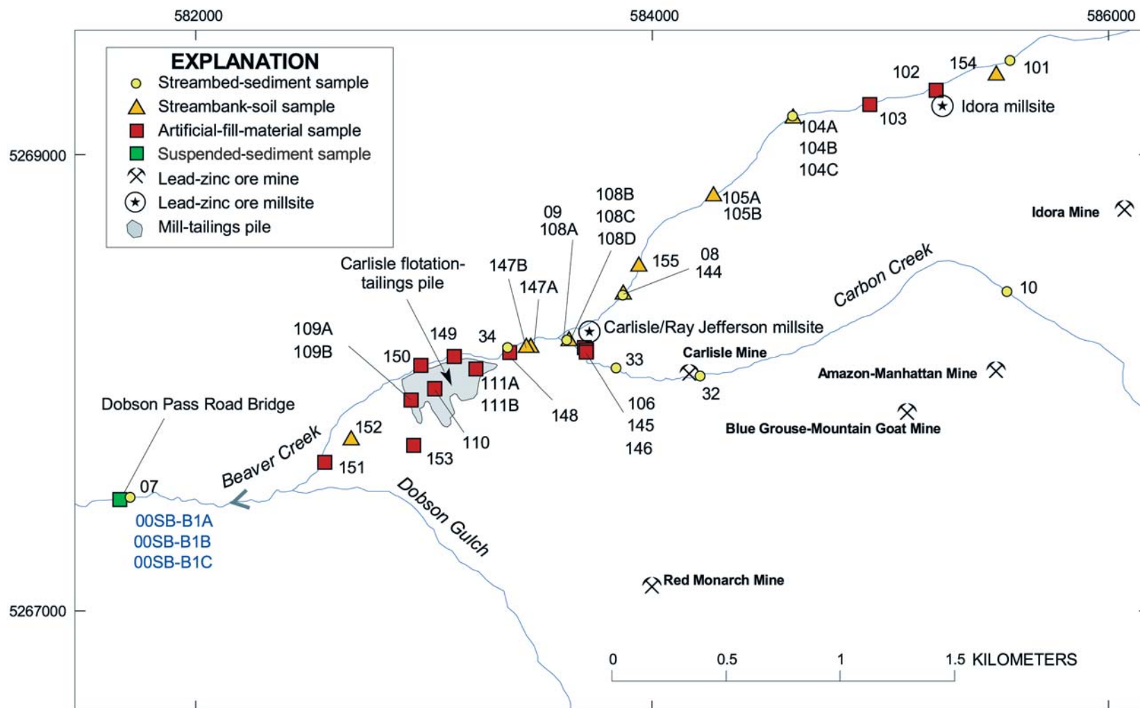
Figure 5. Upper Beaver Creek drainage in the northern Coeur d'Alene Mining District, northern Idaho (figs. 1, 2), showing locations of mines, millsites, and tailings piles and of sampling sites for streambed sediment, suspended sediment, streambank soil, and artificial-fill material.
