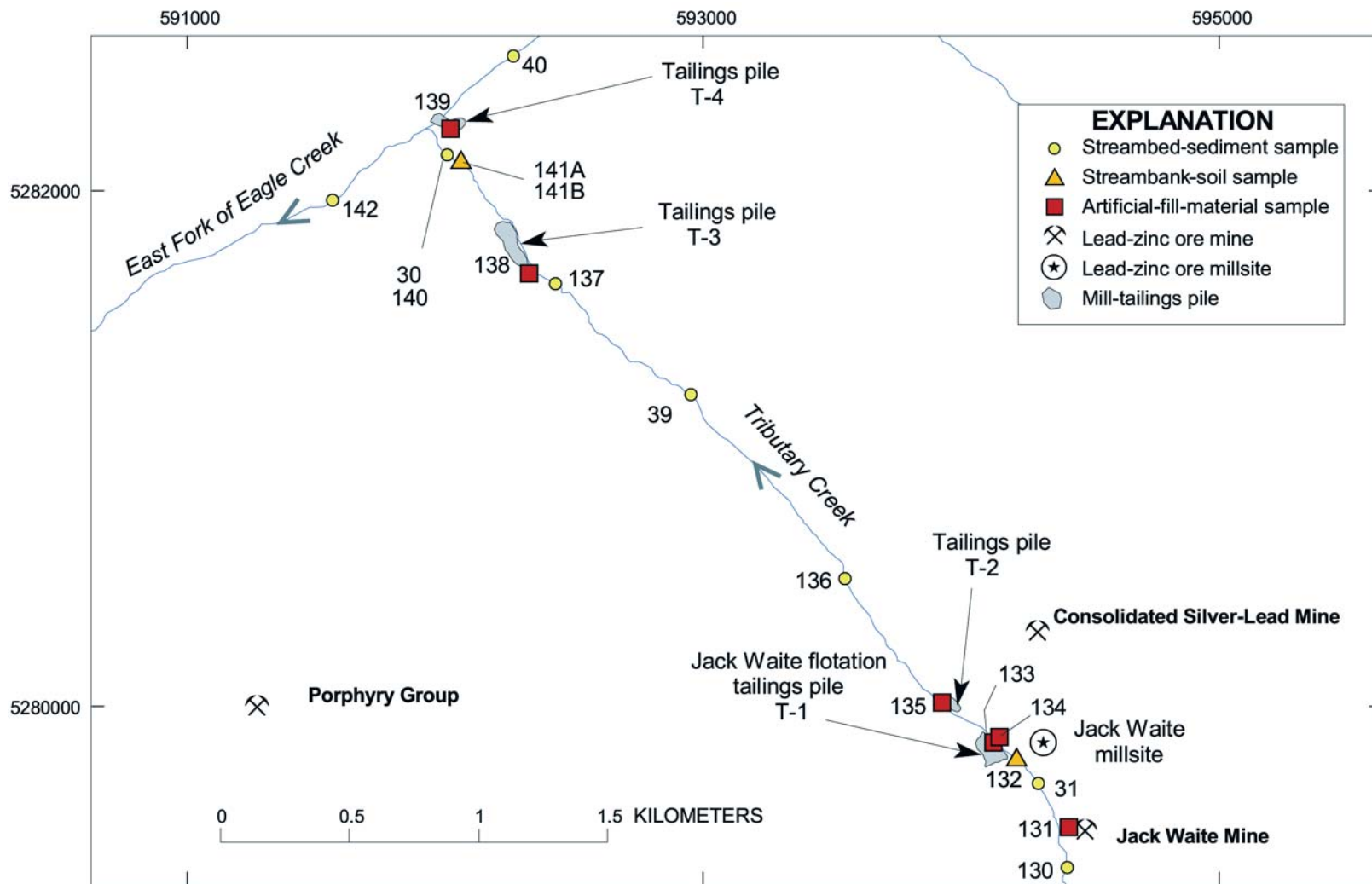
Figure 4. Tributary Creek and upper East Fork of Eagle Creek drainages in the northern Coeur d'Alene Mining District, northern Idaho (figs. 1, 2), showing locations of mines, millsites, and tailings piles and of sampling sites for streambed sediment, suspended sediment, streambank soil, and artificial-fill material.
