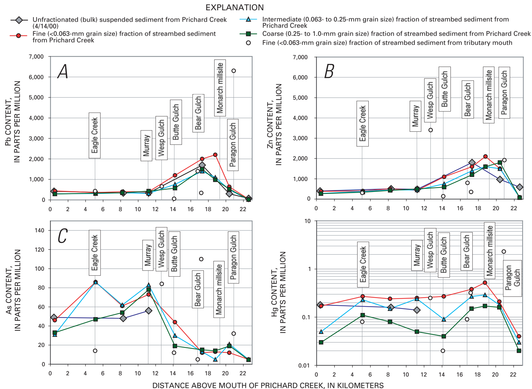
Figure 10. Pb (A), Zn (B), As (C), and Hg (D) contents in three grain-size fractions of samples of streambed sediment and in samples of unfractionated (bulk) suspended sediment collected from the Prichard Creek drainage basin in the northern Coeur d'Alene Mining District, northern Idaho (figs. 1, 2), versus distance upstream from mouth of Prichard Creek, beginning (at right) at head of Prichard Creek and continuing down to mouth. Data points for samples of fine (<0.063-mm grain size) fraction of streambed sediment from tributaries to Prichard Creek are plotted at location of confluence of tributary and Prichard Creek.
