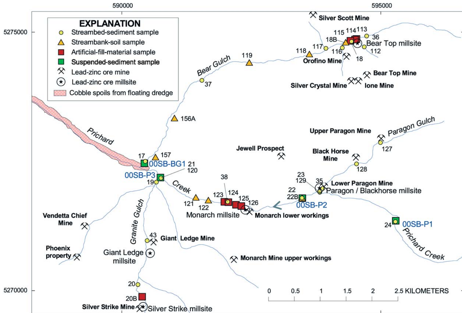
Figure 3. Upper Prichard Creek drainage in the northern Coeur d'Alene Mining District, northern Idaho (figs. 1, 2), showing locations of mines and mill-sites and of sampling sites for streambed sediment, suspended sediment, streambank soil, and artificial-fill material.
