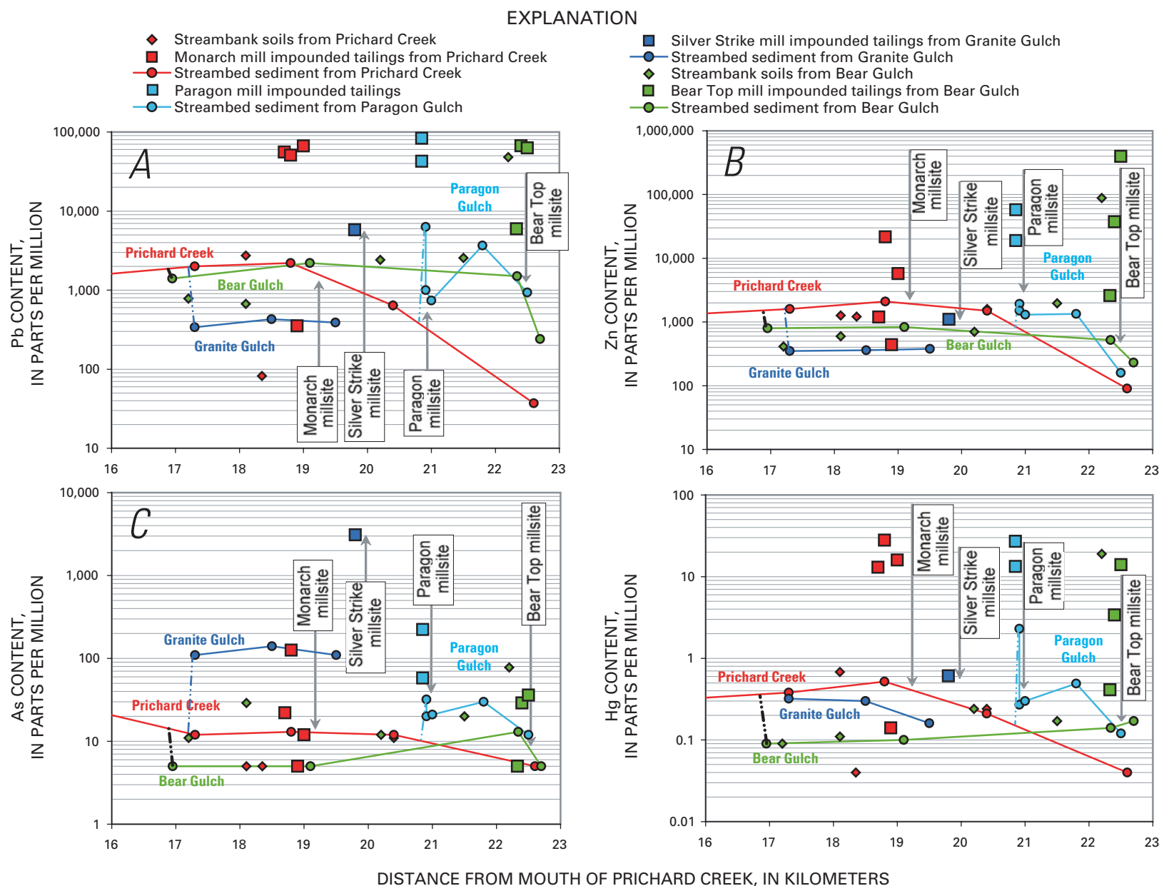
Figure 11. Pb (A), Zn (B), As (C), and Hg (D) contents in fine (<0.063-mm grain size) fraction of samples of streambed sediment, streambank soil, and impounded tailings collected from Prichard Creek and Paragon, Granite, and Bear Gulches in the northern Coeur d'Alene Mining District, northern Idaho (fig. 3), versus distance upstream from mouth of Prichard Creek, with locations of four historical lead-zinc ore-concentration mills along stream labeled. Data for Paragon mill gravity tailings from Johnson (1999).
