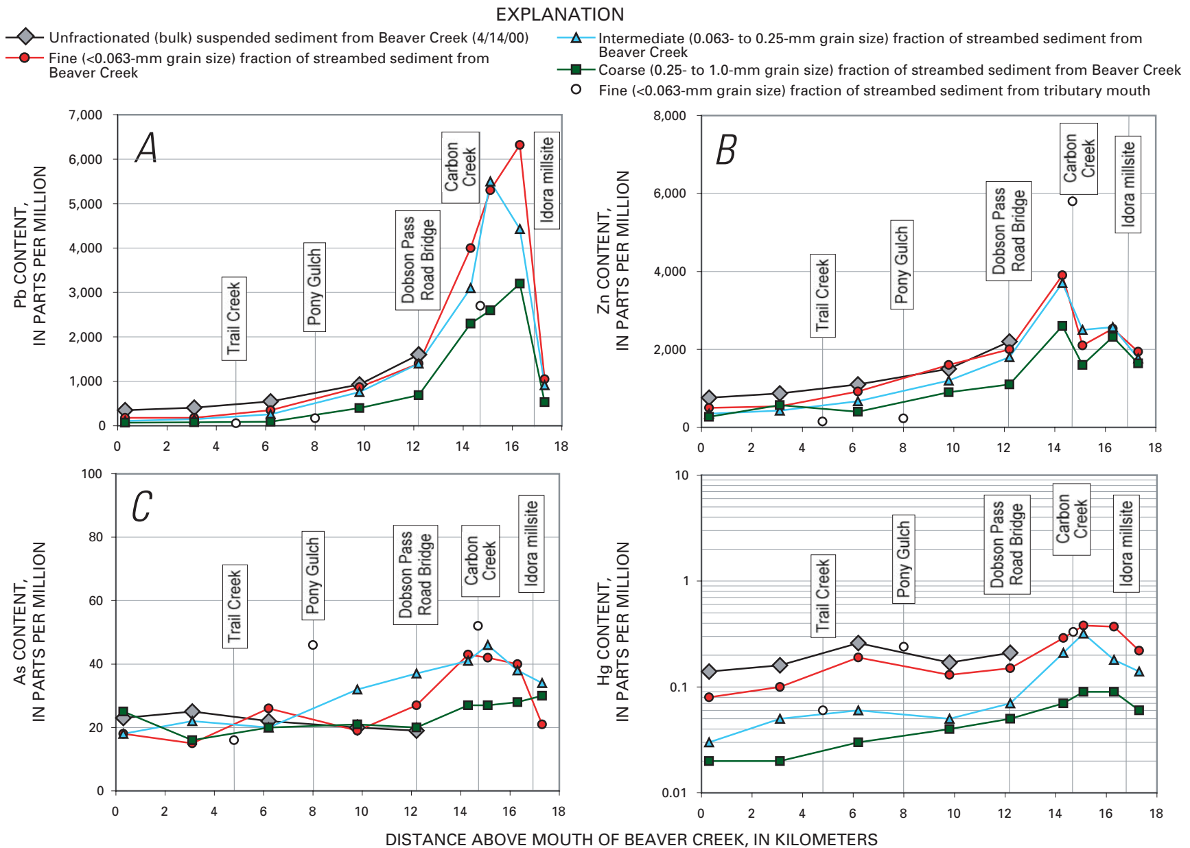
Figure 14. Pb (A), Zn (B), As (C), and Hg (D) contents in three grain-size fractions of samples of streambed sediment and in samples of unfractionated (bulk) suspended sediment in the Beaver Creek drainage basin in the northern Coeur d'Alene Mining District, northern Idaho (figs. 1, 2), versus distance upstream from mouth of Beaver Creek, beginning (at right) at head of creek and continuing down to mouth. Data points for samples of fine (<0.063-mm grain size) fraction of streambed sediment from tributaries to Beaver Creek are plotted at confluence of tributary and Beaver Creek.
