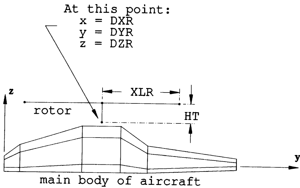
Figure 3.8: Side view of rotor geometry.
