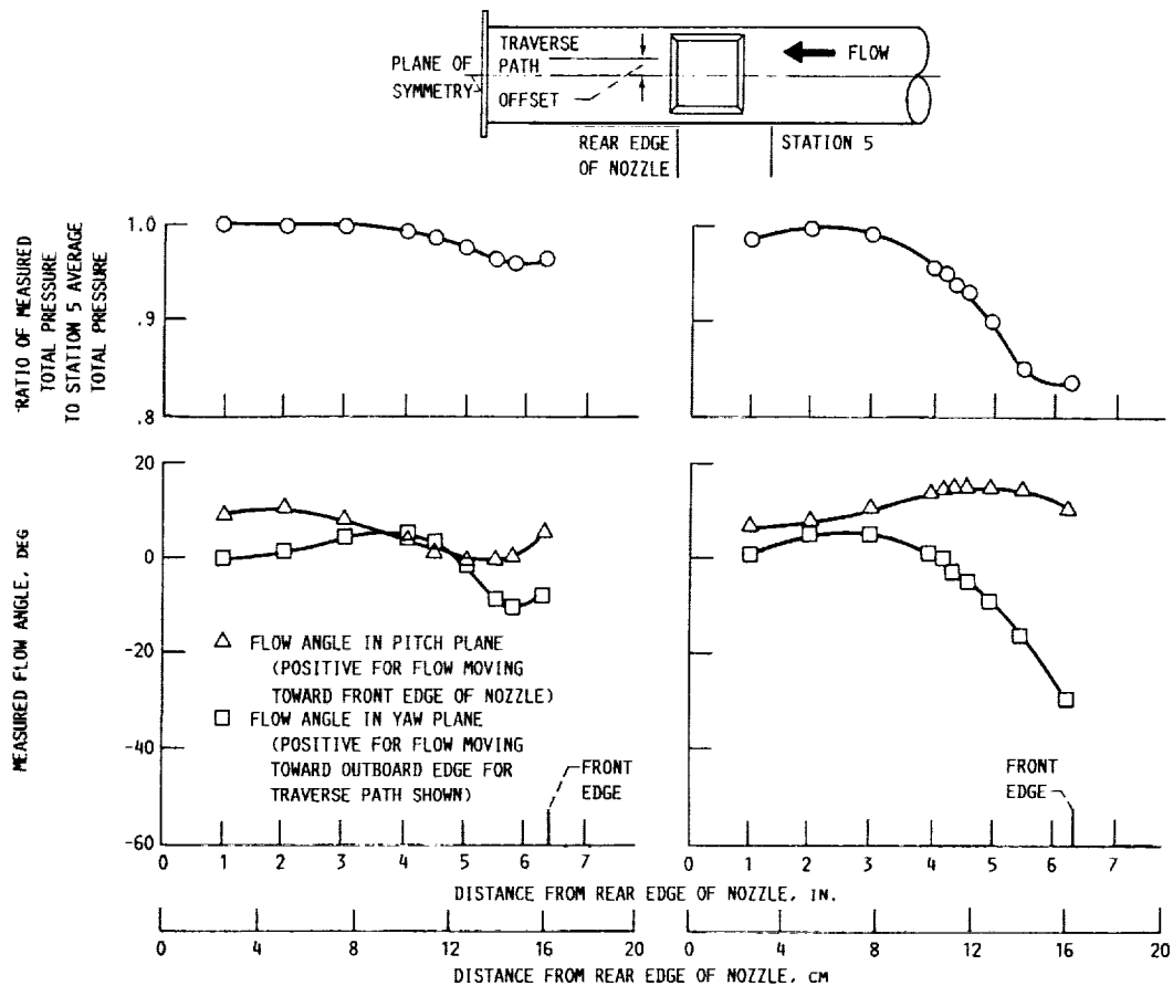
(a) TRAVERSE PATH OFFSET 4.5 IN. (11.4 CM) FROM PLANE OF SYMMETRY. (b) TRAVERSE PATH OFFSET 1.5 IN. (3.8 CM) FROM PLANE OF SYMMETRY.
