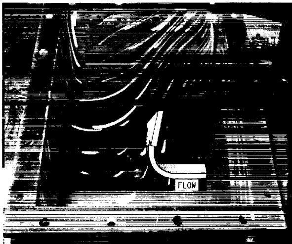
FIG 12. - FLOW VISUALIZATION ON VENTRAL DUCT SIDE WALL.
