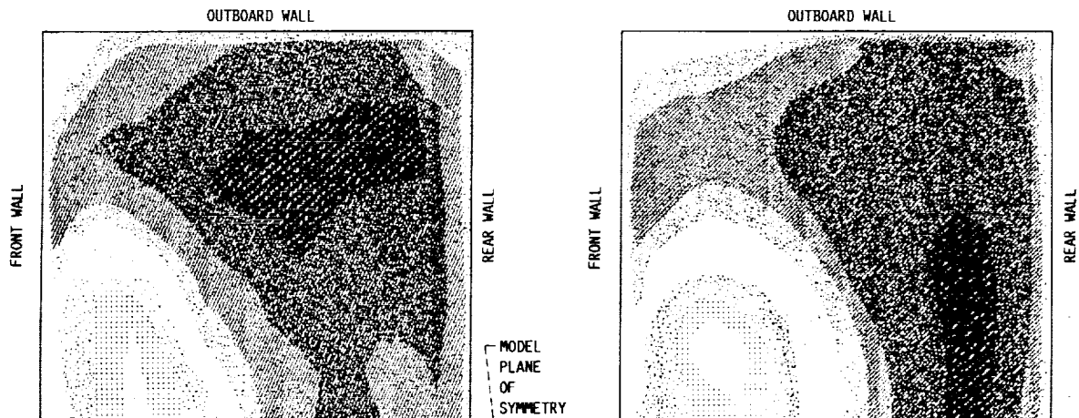
(a) EXPERIMENTAL PITOT PRESSURE.
