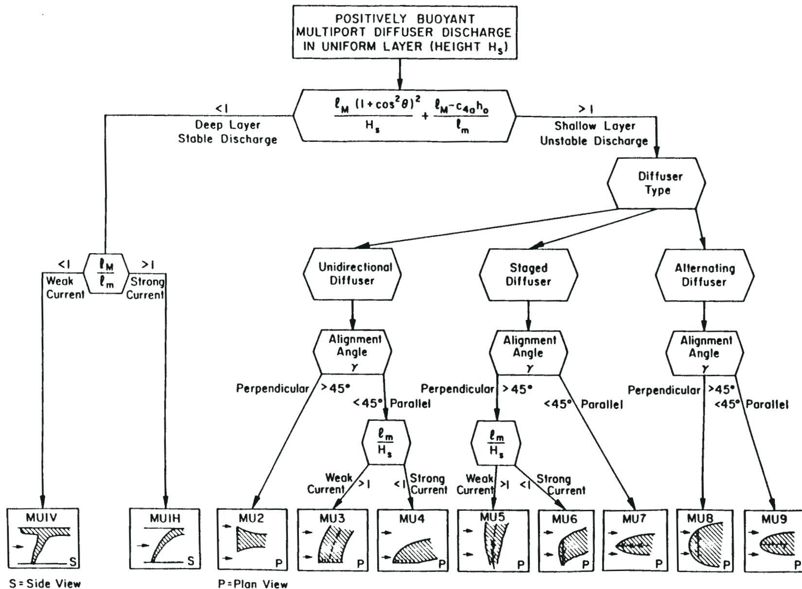
Figure 8-17. CORMIX2 sub-classification: flow classes for positively buoyant multiport discharges in uniform ambient layer.
