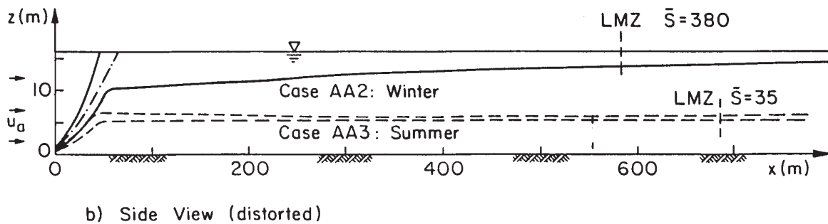
Figure 9-5. Cases AA2 and AA3: predicted (CORMIX1) far-field behavior for single port discharge (modified design) in winter and summer conditions.
