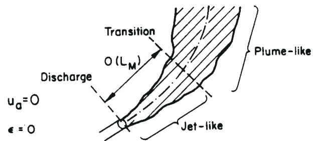
a) Buoyant Jet in Stagnant Uniform Environment
