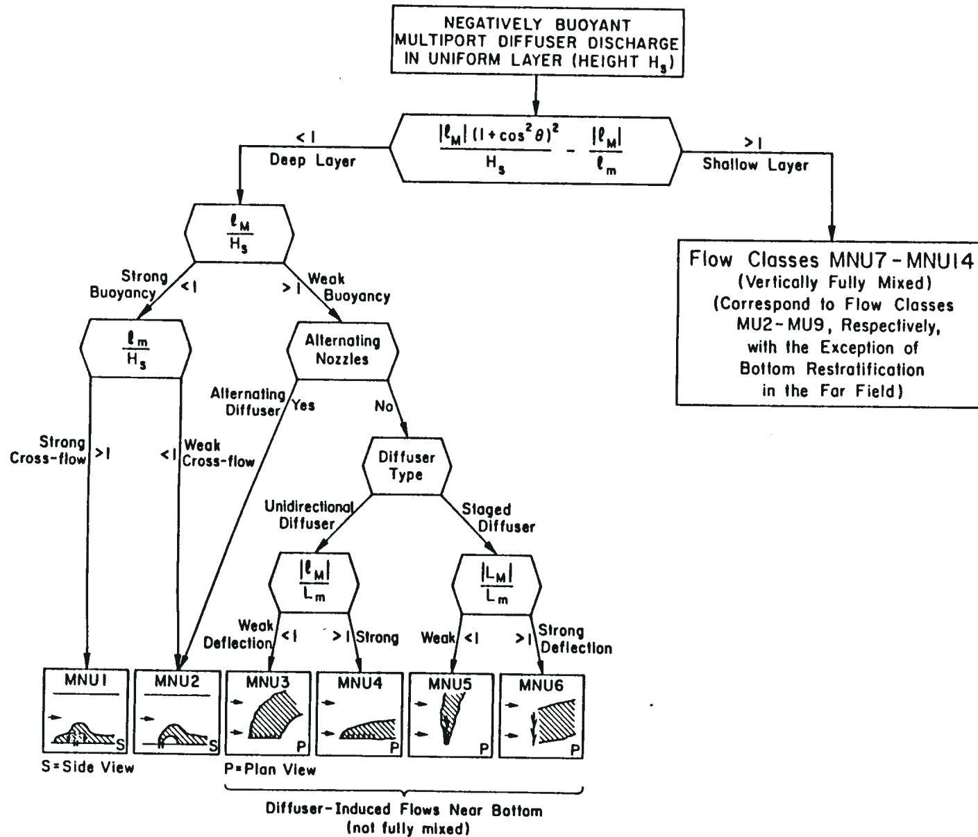
Figure 8-18. CORMIX2 sub-classification: flow classes for negatively buoyant multiport discharges in uniform ambient layer.
