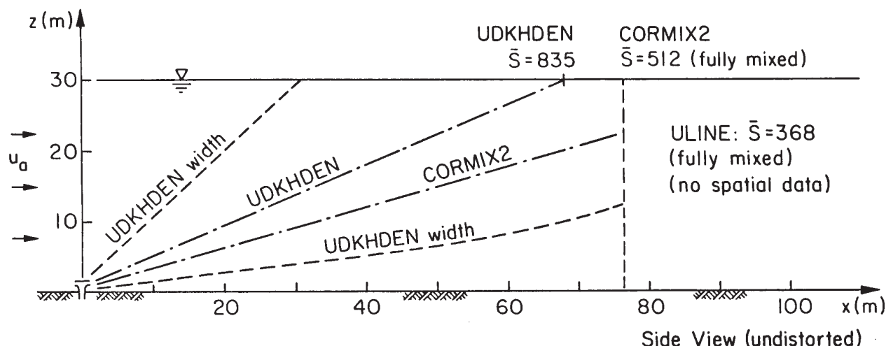
Figure 9-10. Case BB2: multiport diffuser discharge in uniform ambient; comparison of jet integral models and CORMIX2.
