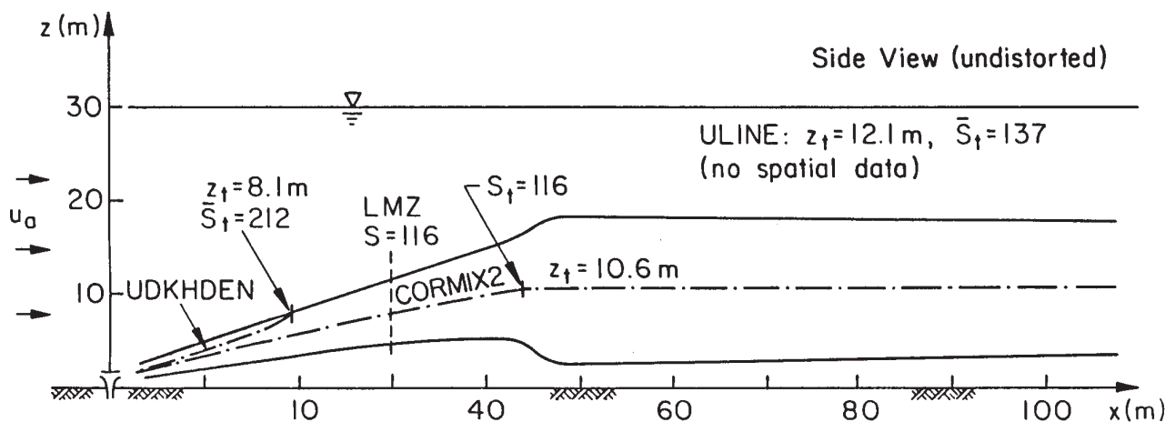
Figure 9-8. Case BB1: multiport diffuser discharge under stratified conditions; comparison of jet integral models and CORMIX2.
