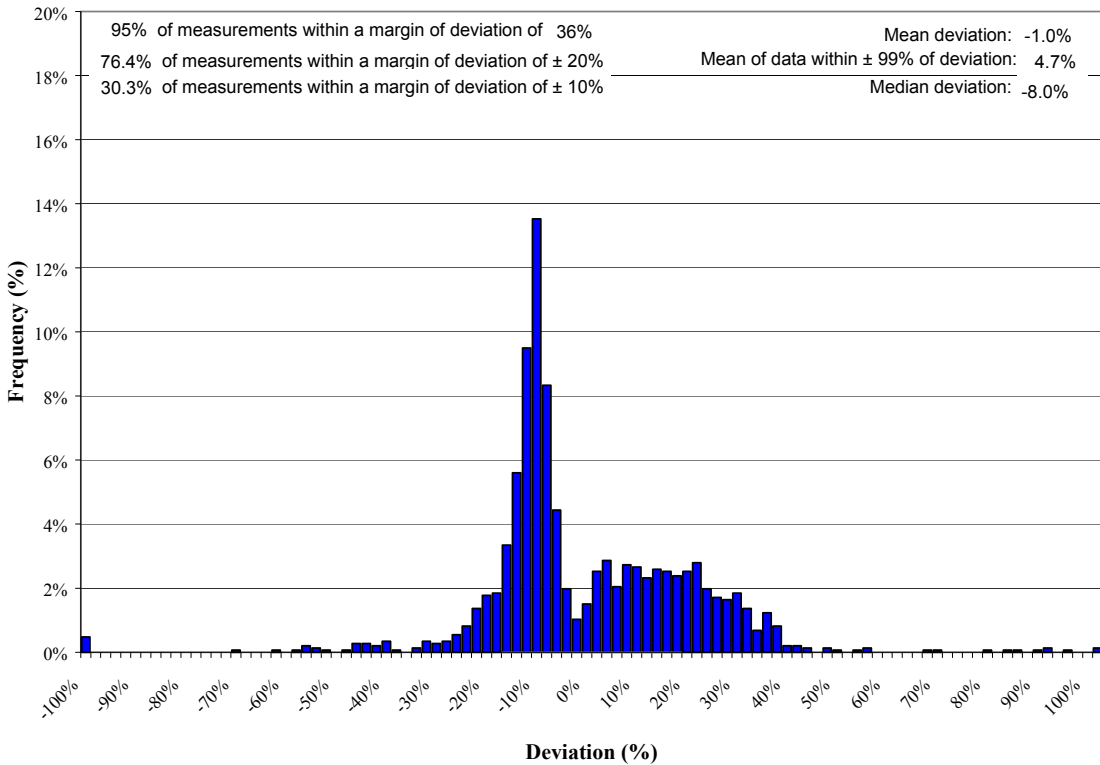
Figure 4-22. Flow deviation distribution—Test D.
