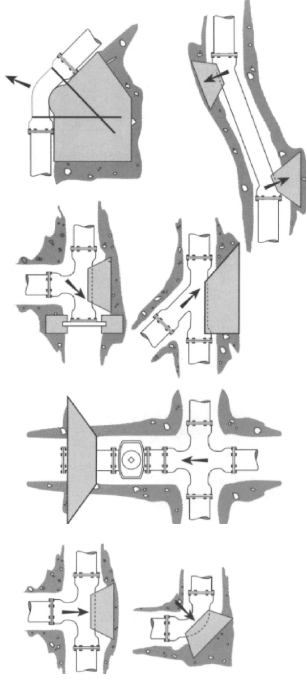
Thrust Blocks
