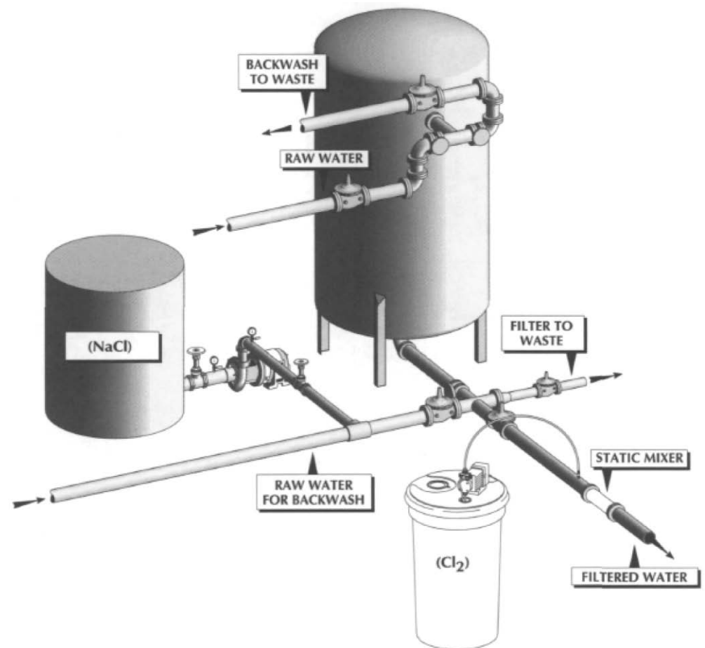
Ion Exchange Water Softener
