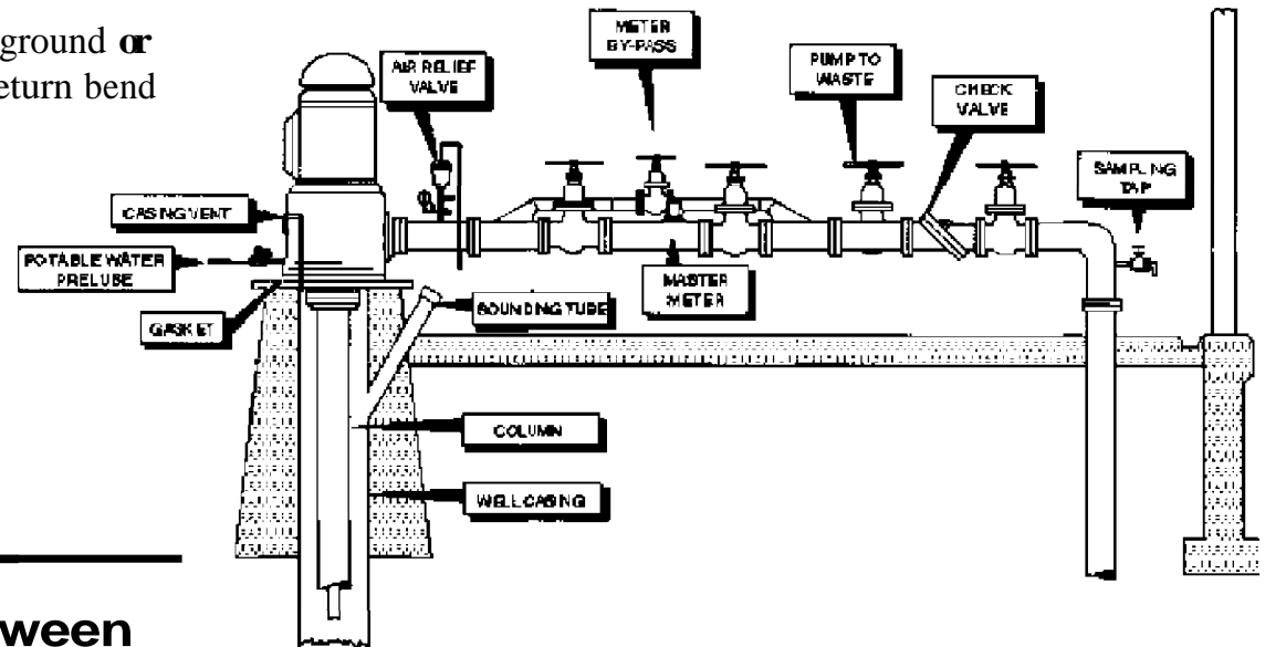
Typical Lineshaft Turbine Installation
