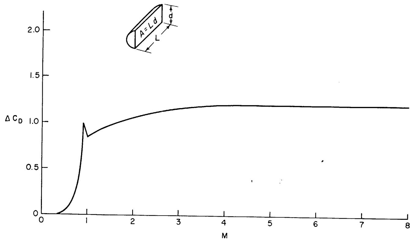
Figure 4-5—Leading Edge Drag
