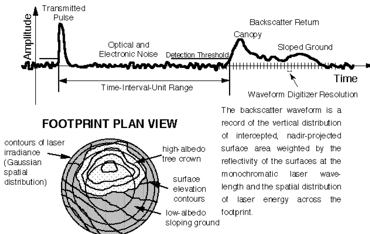
Figure 2: Laser Altimetry Echo Recovery
