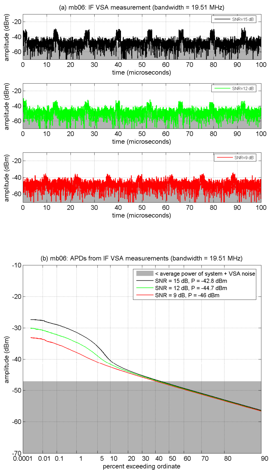
Figure B-56. IF amplitude analyses of MB-06 at INR_{TOV} .
