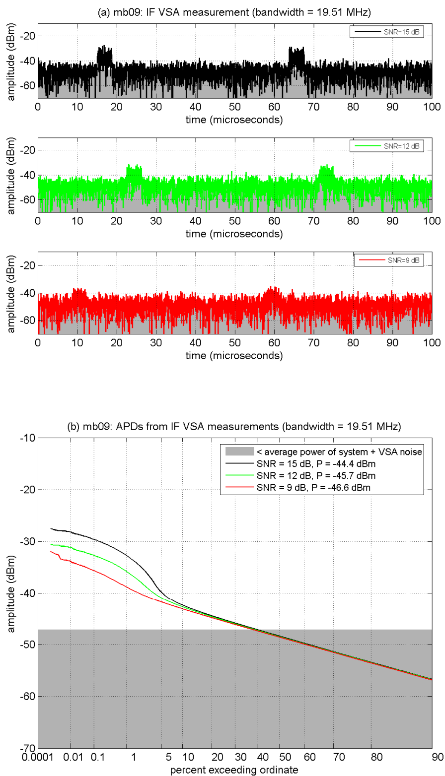
Figure B-62. IF amplitude analyses of MB-09 at INR_{TOV} .
