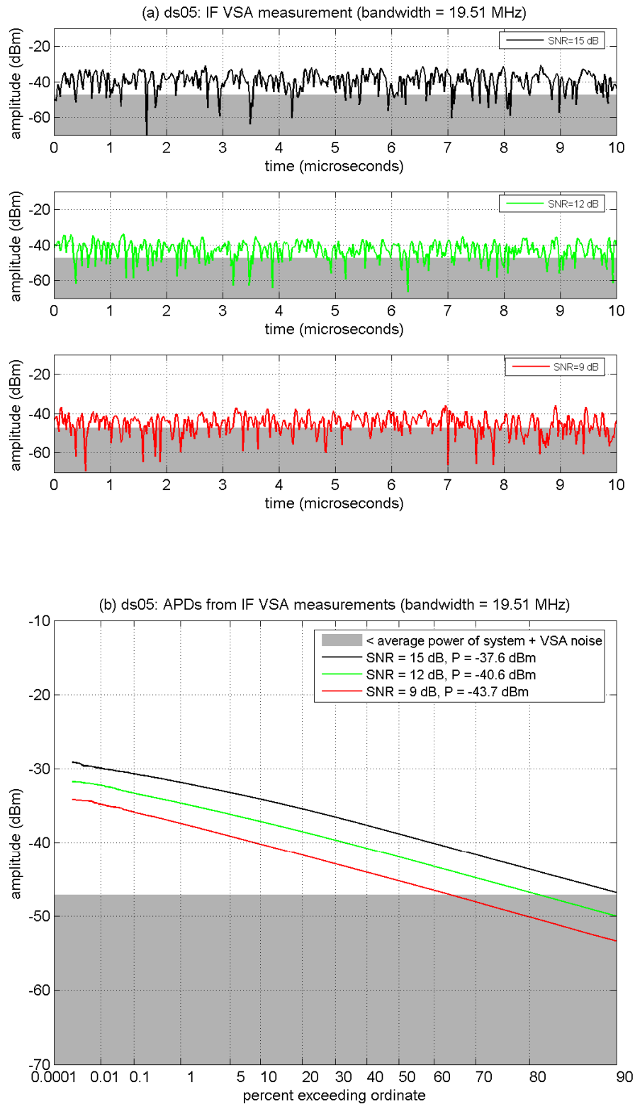
Figure B-42. IF amplitude analyses of DS-05 at INR_{TOV} .
