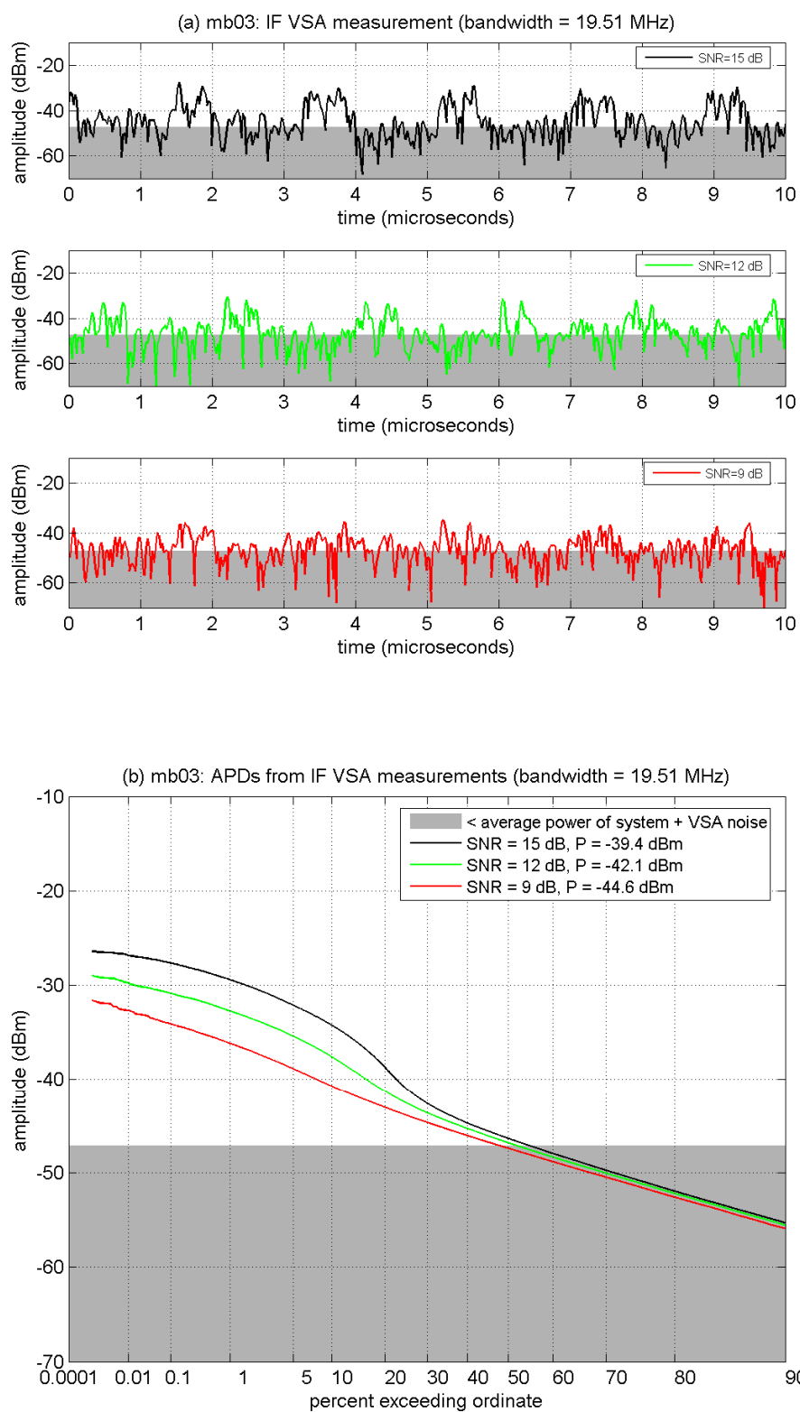
Figure B-50. IF amplitude analyses of MB-03 at INR_{TOV} .
