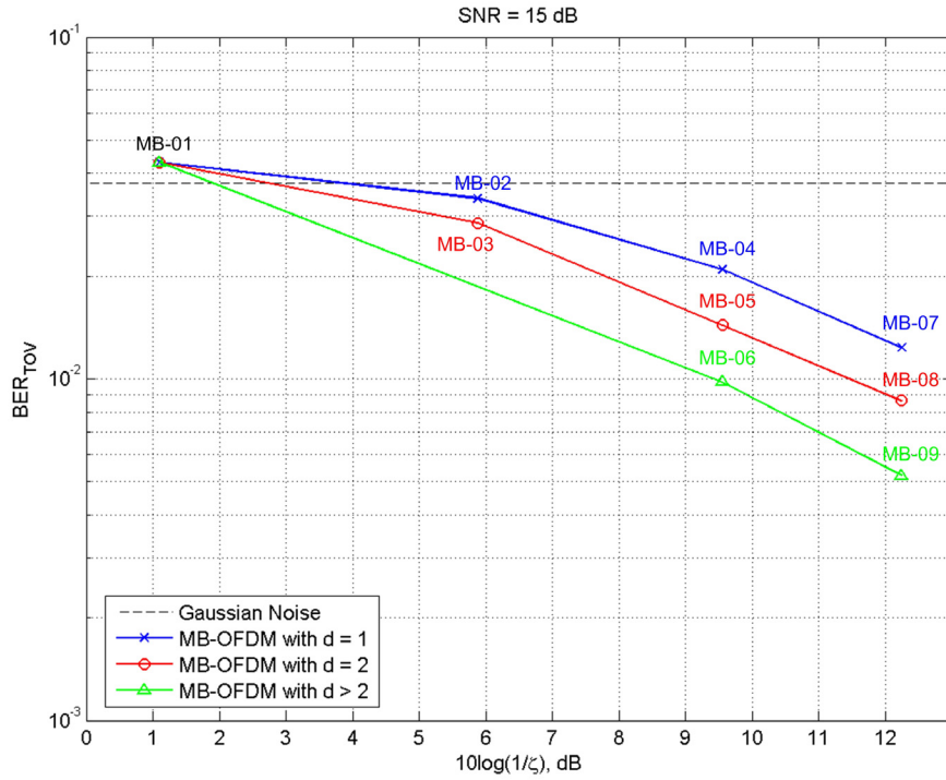
Figure 33. BER_{TOV} versus 10\log(1/\zeta) for a DTV channel operating at SNR = 15 dB and exposed to MB interference.
