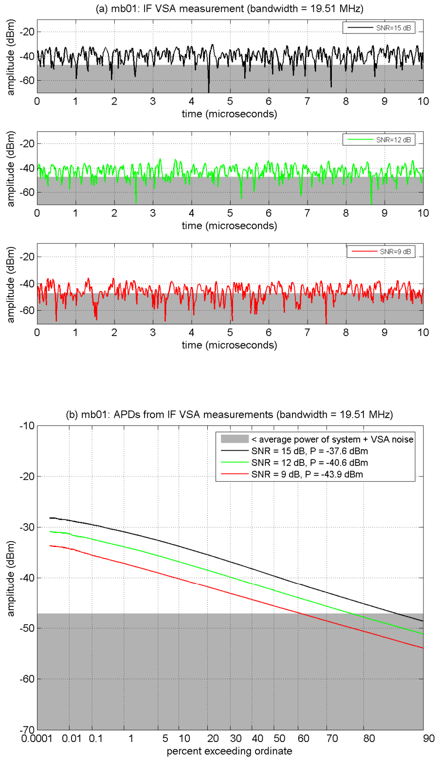
Figure B-46. IF amplitude analyses of MB-01 at INR_{TOV} .
