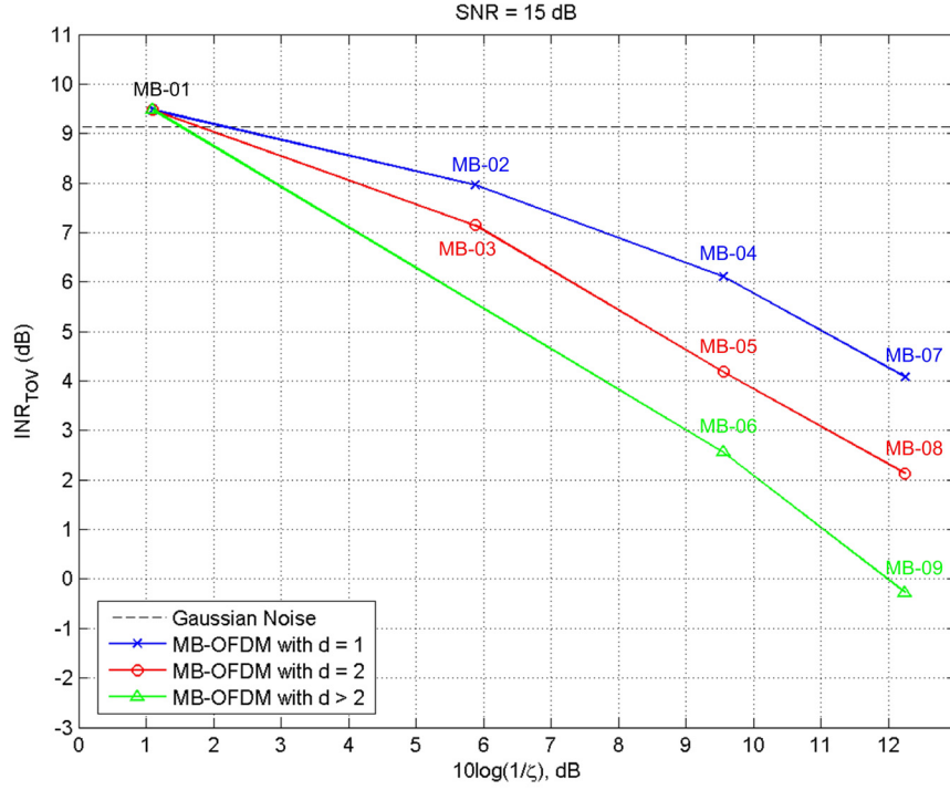
Figure 32. INR_{TOV} versus 10\log(1/\zeta) for a DTV channel operating at SNR = 15 dB and exposed to MB interference.
