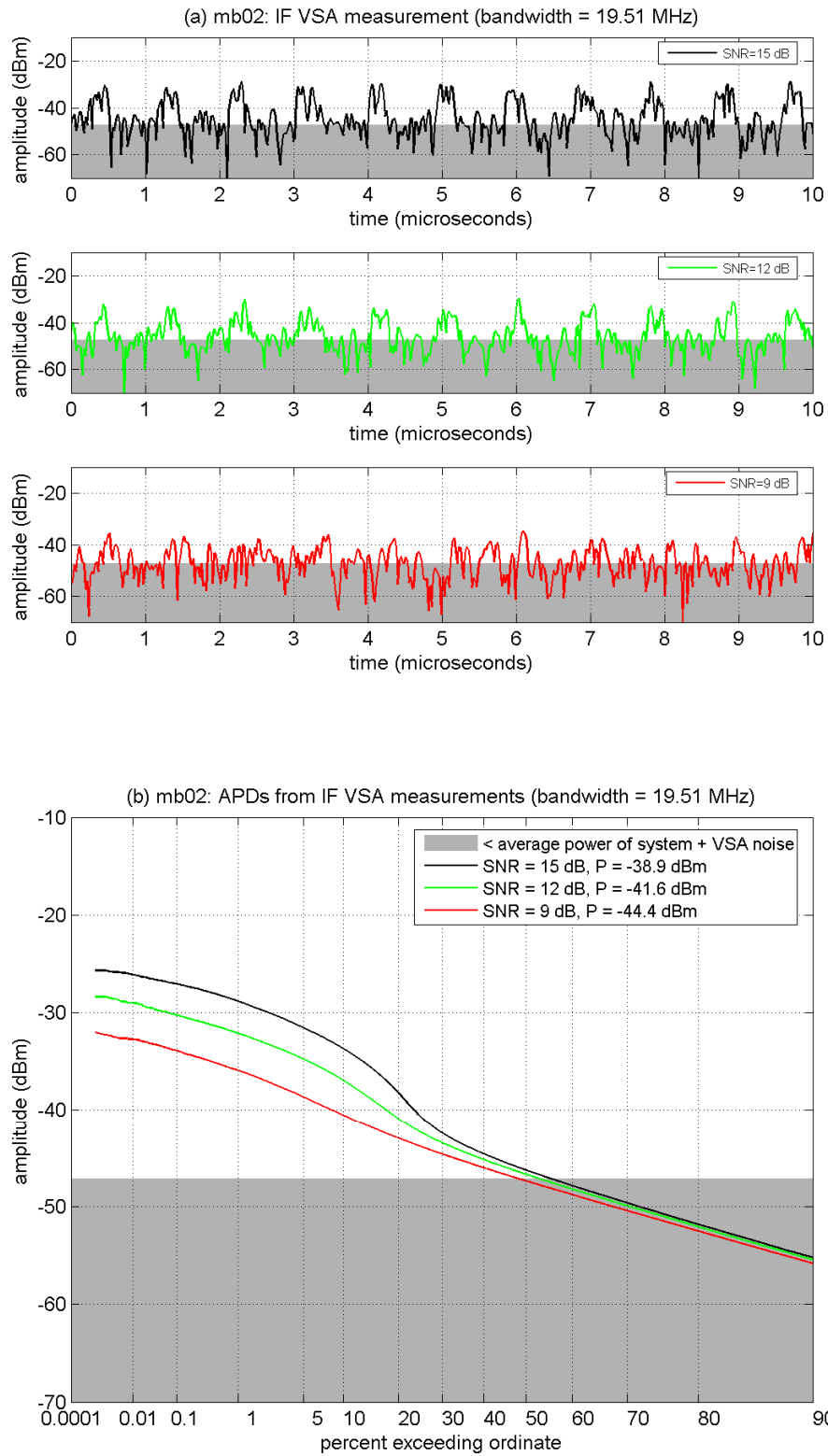
Figure B-48. IF amplitude analyses of MB-02 at INR_{TOV} .
