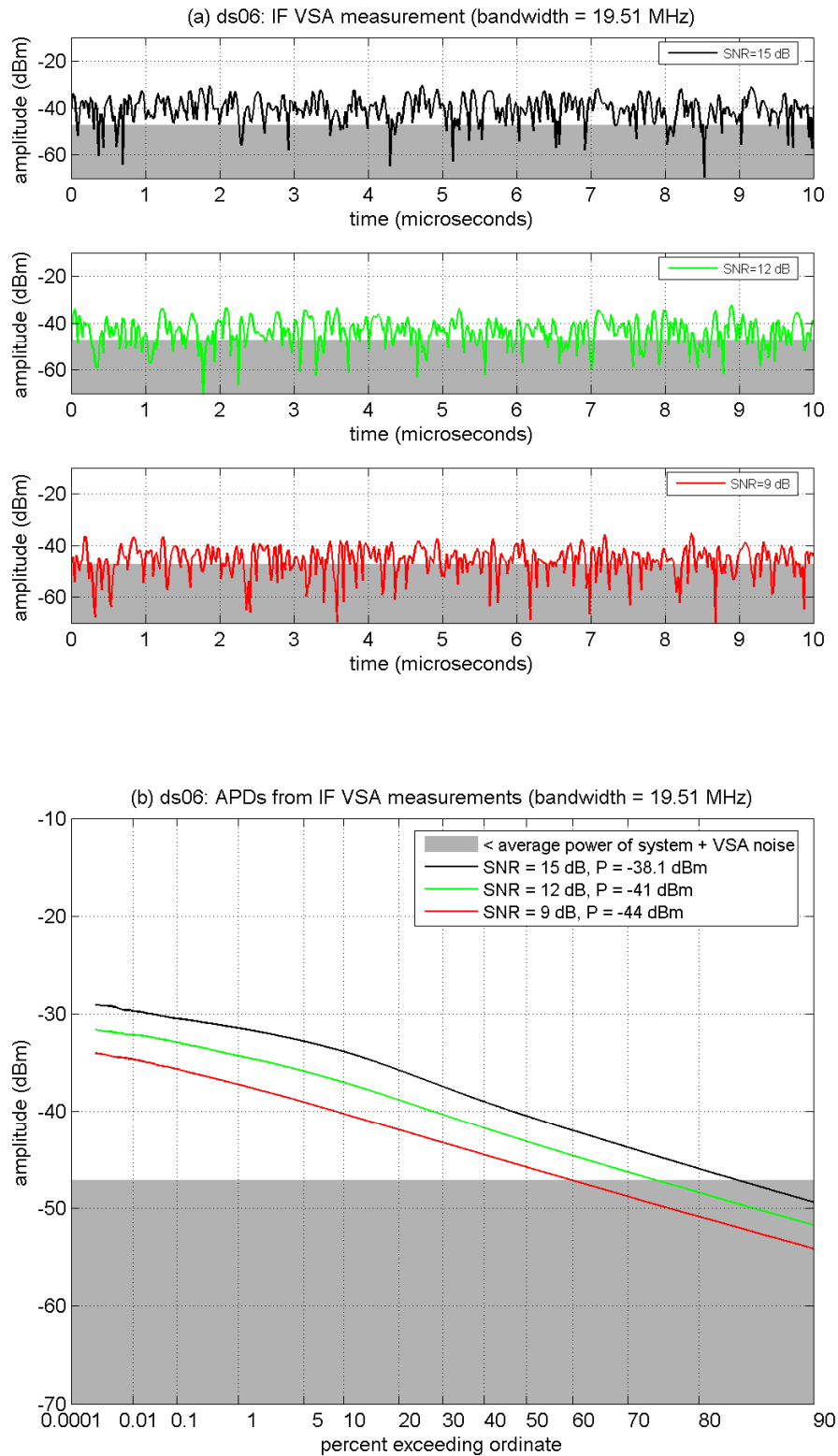
Figure B-44. IF amplitude analyses of DS-06 at INR_{TOV} .
