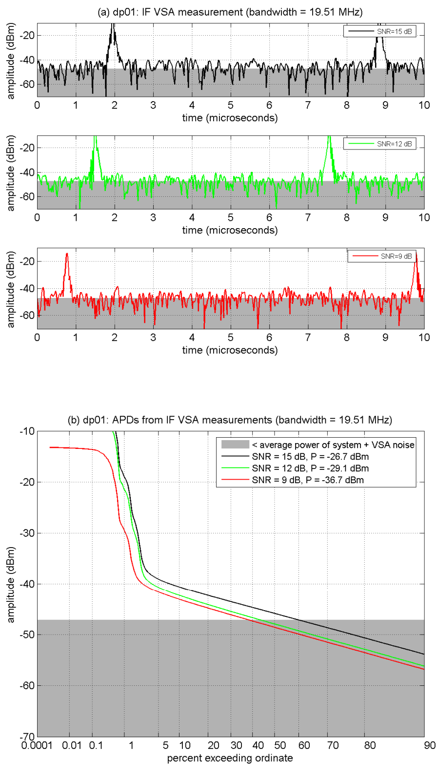
Figure B-26. IF amplitude analyses of DP-01 at INR_{TOV} .
