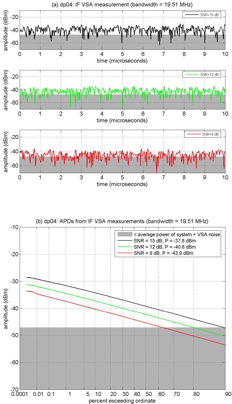
Figure B-32. IF amplitude analyses of DP-04 at INR_{TOV} .
