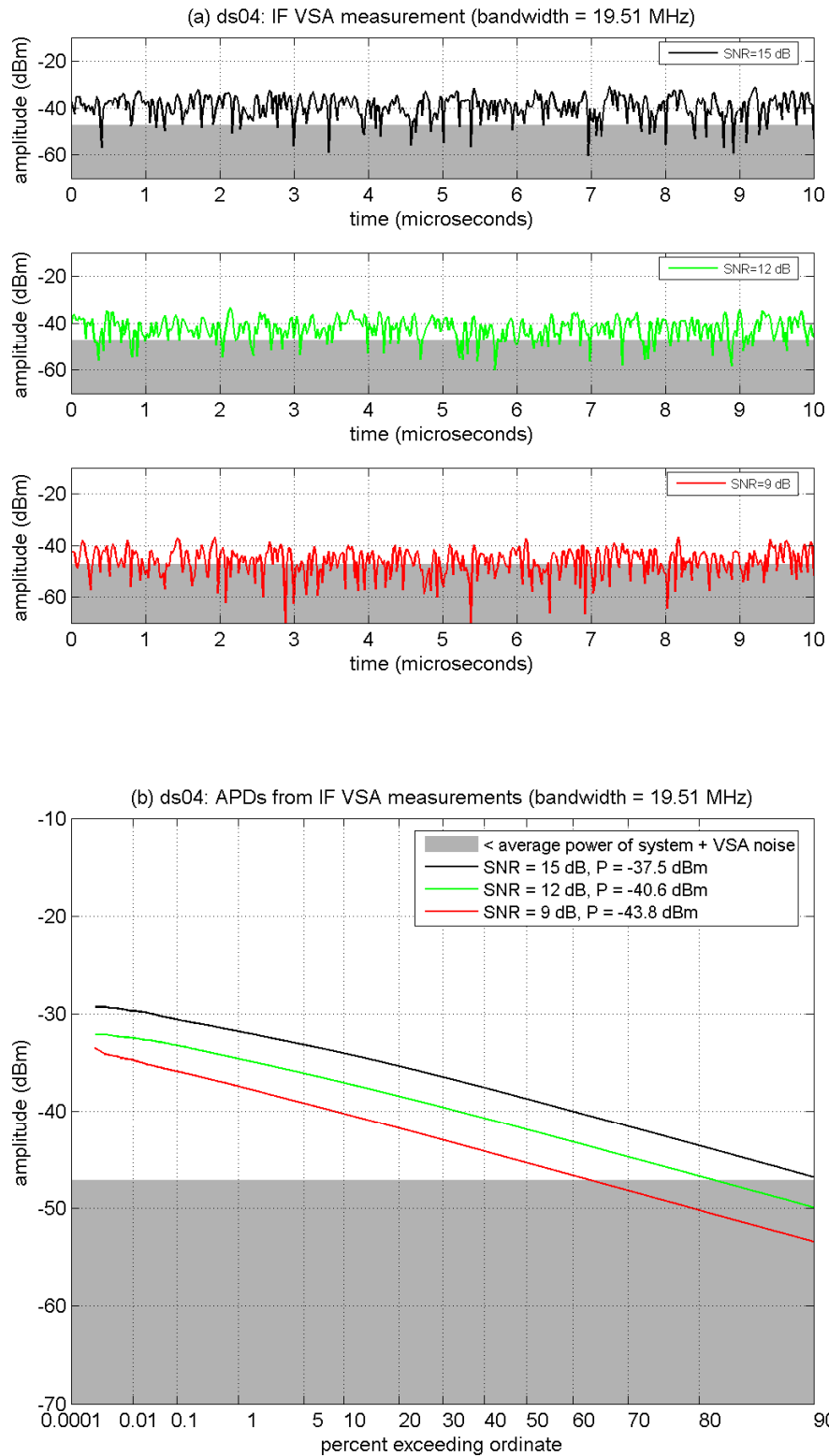
Figure B-40. IF amplitude analyses of DS-04 at INR_{TOV} .
