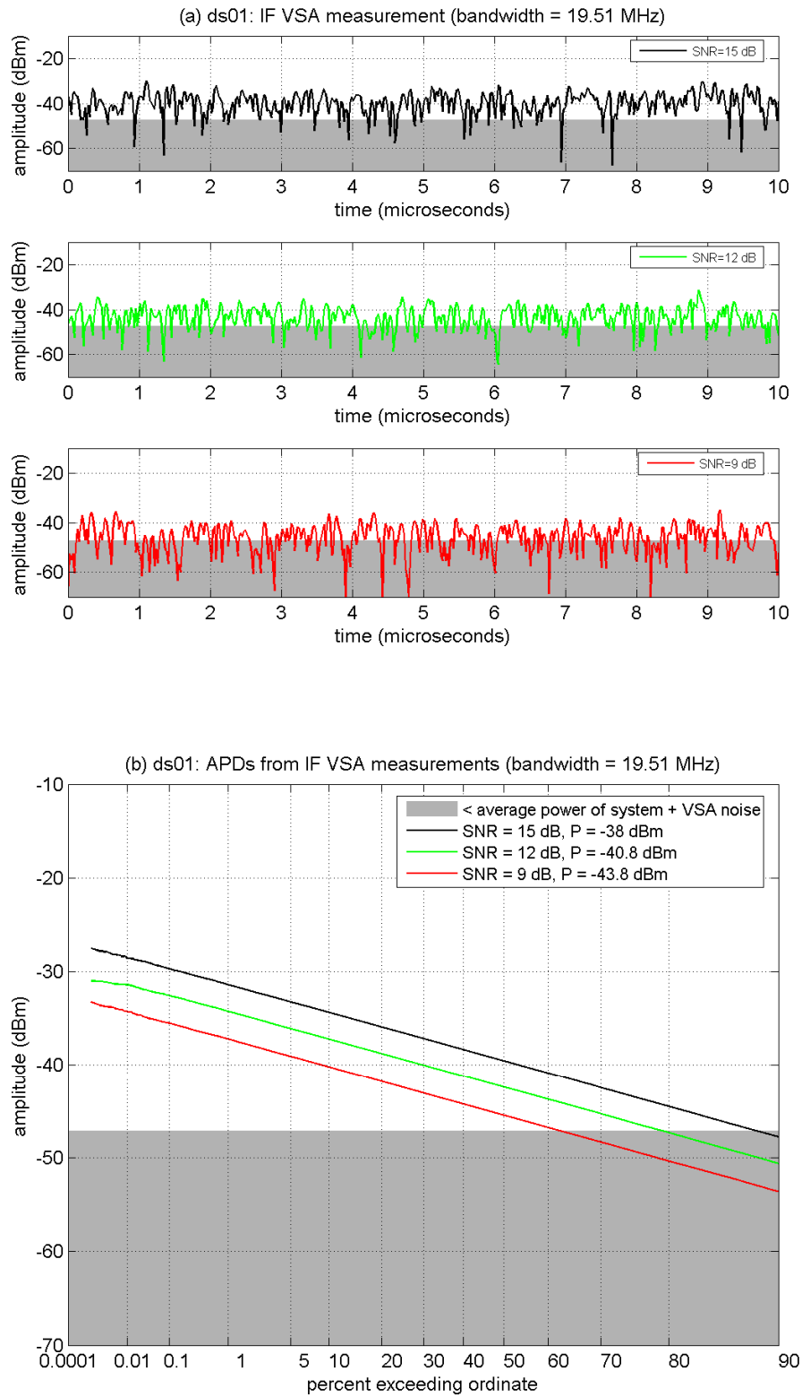
Figure B-34. IF amplitude analyses of DS-01 at INR_{TOV} .
