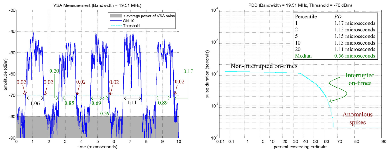
Figure B-3. Pulse duration statistics of gated noise with 50% duty cycle and 1- \mu s on-time.
