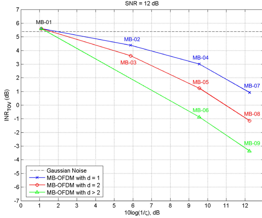
Figure 30. INR_{TOV} versus 10\log(1/\zeta) for a DTV channel operating at SNR = 12 dB and exposed to MB interference.
