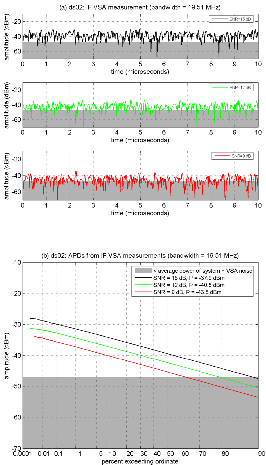
Figure B-36. IF amplitude analyses of DS-02 at INR_{TOV} .
