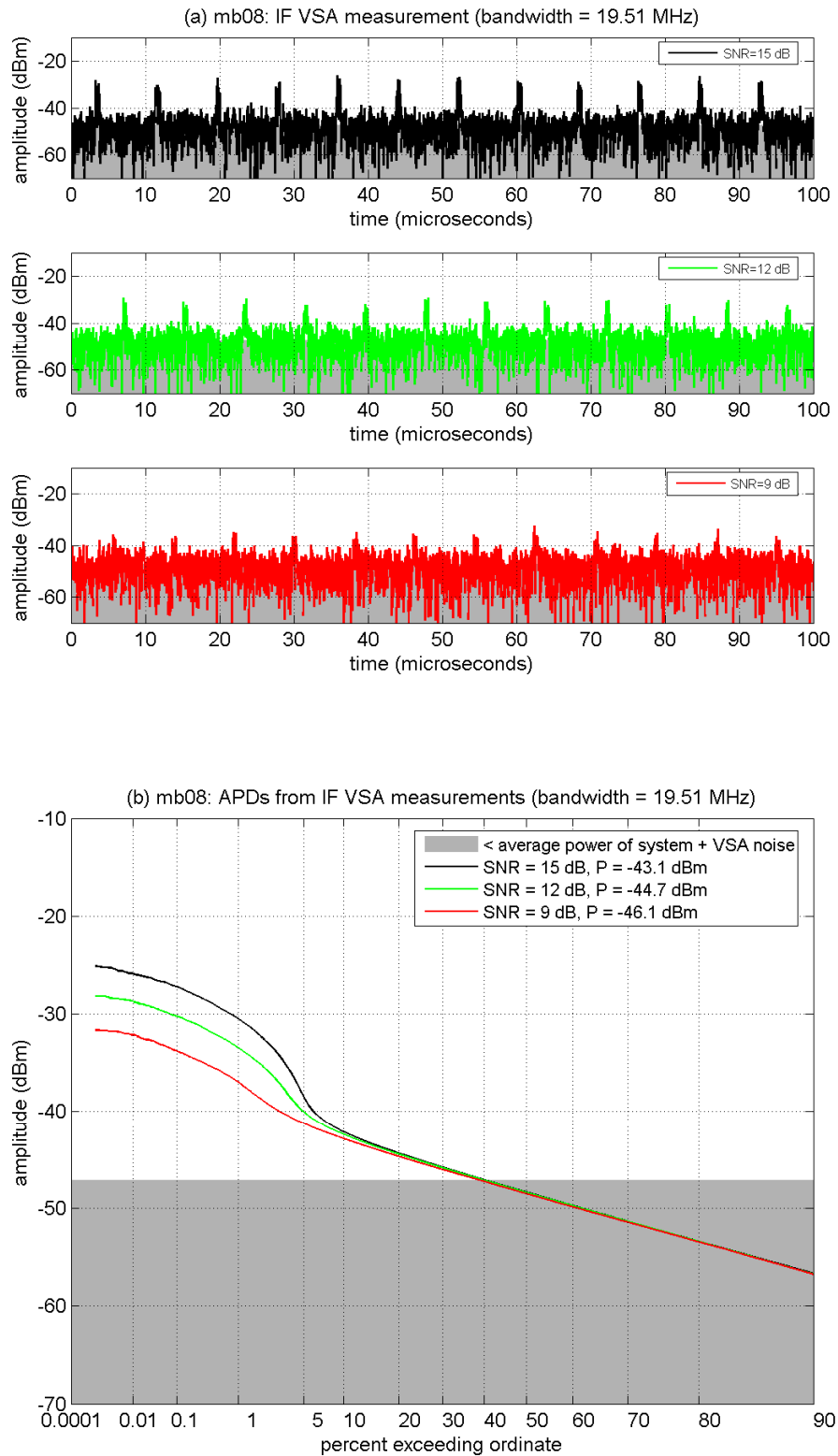
Figure B-60. IF amplitude analyses of MB-08 at INR_{TOV} .
