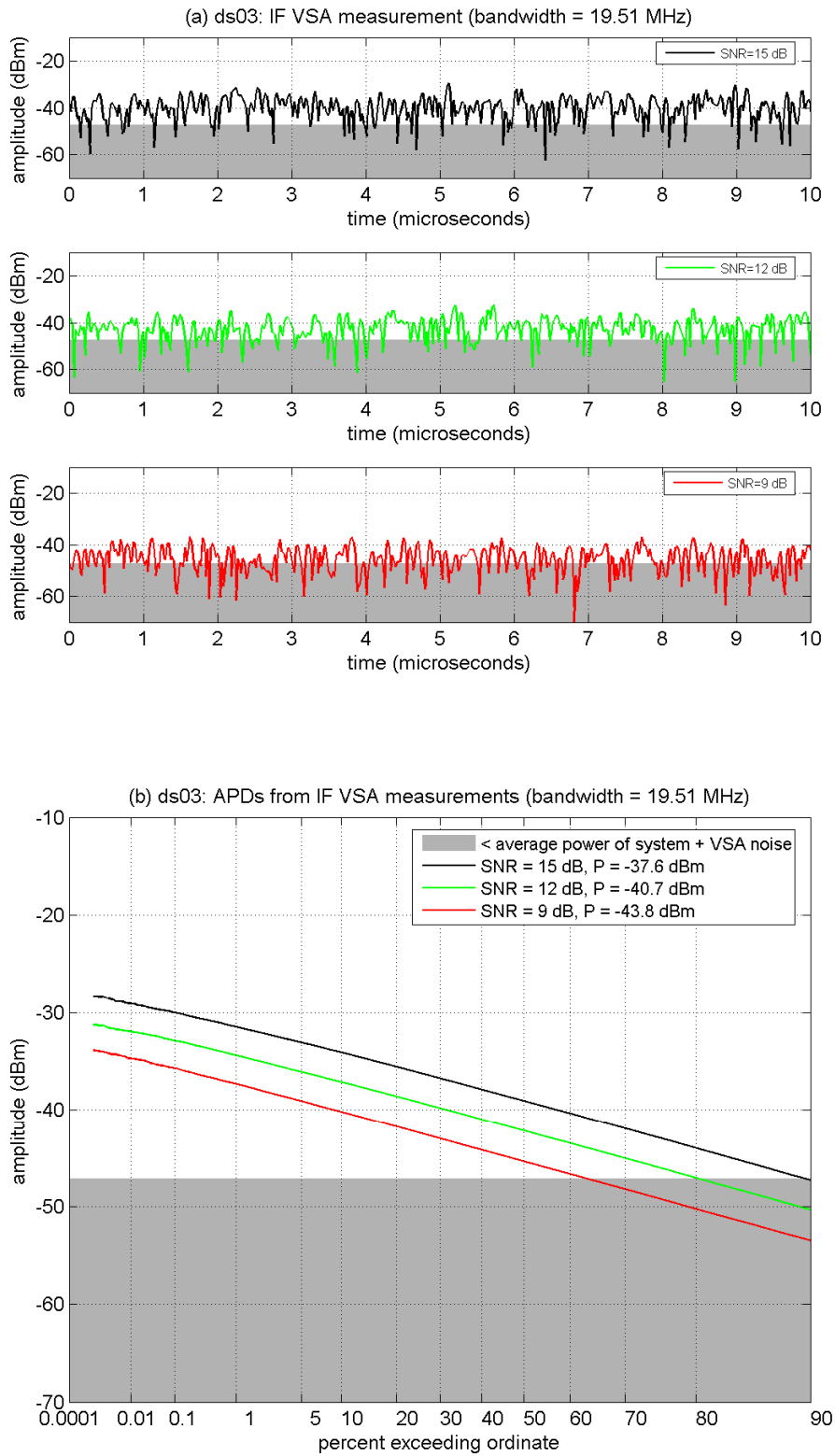
Figure B-38. IF amplitude analyses of DS-03 at INR_{TOV} .
