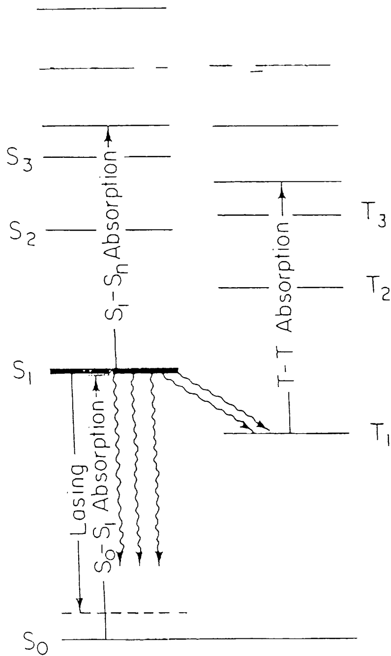
Figure 1. Energy level diagram of a dye molecule.
