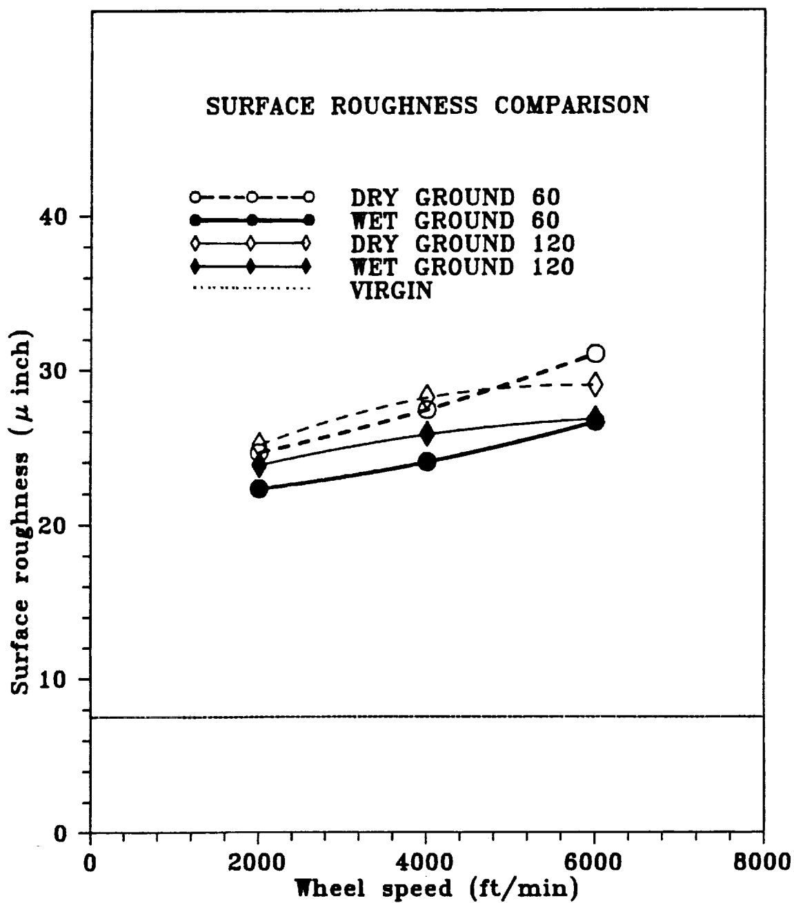
Figure 4. Surface roughness vs wheel speed: virgin material and ground specimens.
