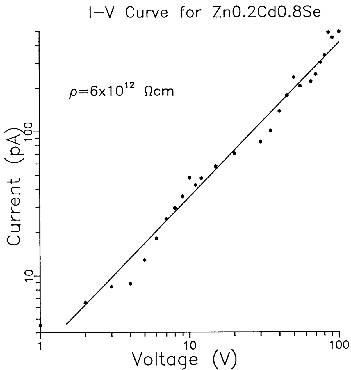
Figure 2. The I-V curve of an as-grown Zn 0.2 Cd 0.8 Se sample, 0.15 cm thick, 0.06 cm 2 contact area.
