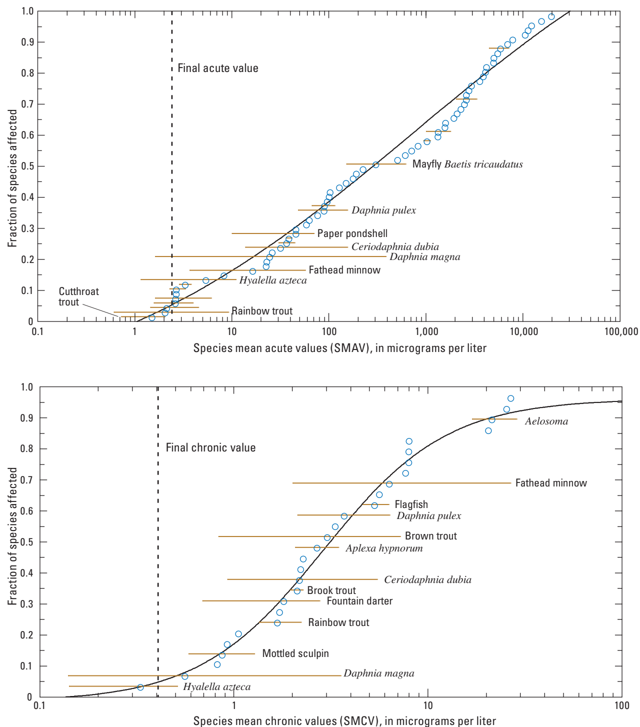
Figure 5. Species sensitivity distributions of cadmium values showing species mean values (open circles), ranges of species values (horizontal lines), 5 th percentile final acute and chronic values (vertical dashed lines), and their fitted logistic distribution curves. All values adjusted to a hardness of 50 milligrams per liter \text{CaCO}_3 .
