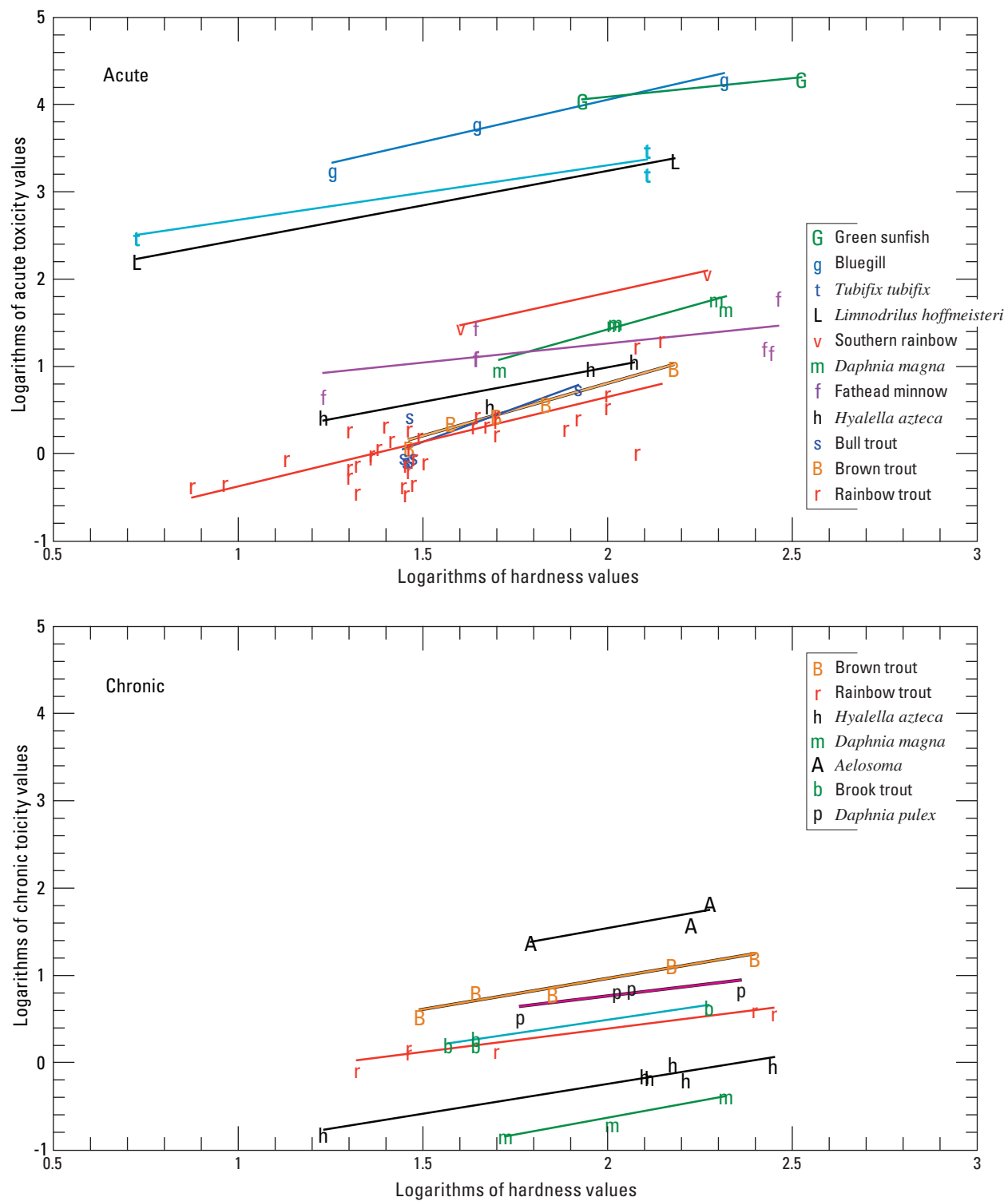
Figure 2. Hardness-toxicity relations for acute and chronic data. Data are from studies in tables 15 and 16 with an “h” in the code/notes column.
