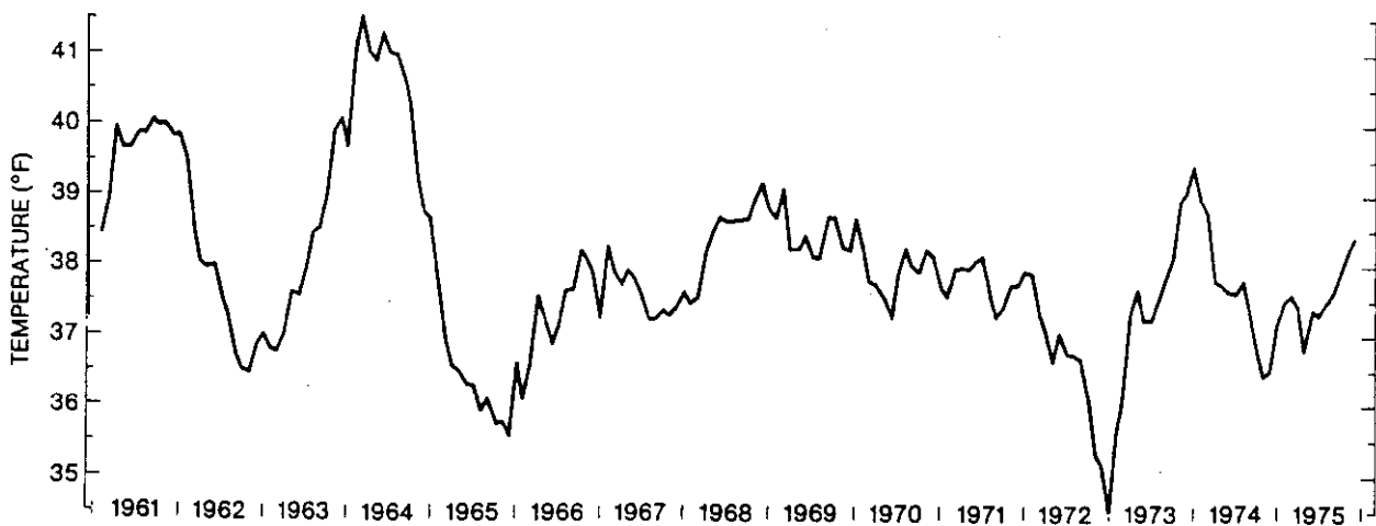
Figure 1. Twelve-month running monthly mean temperatures at Duluth, Minnesota.
