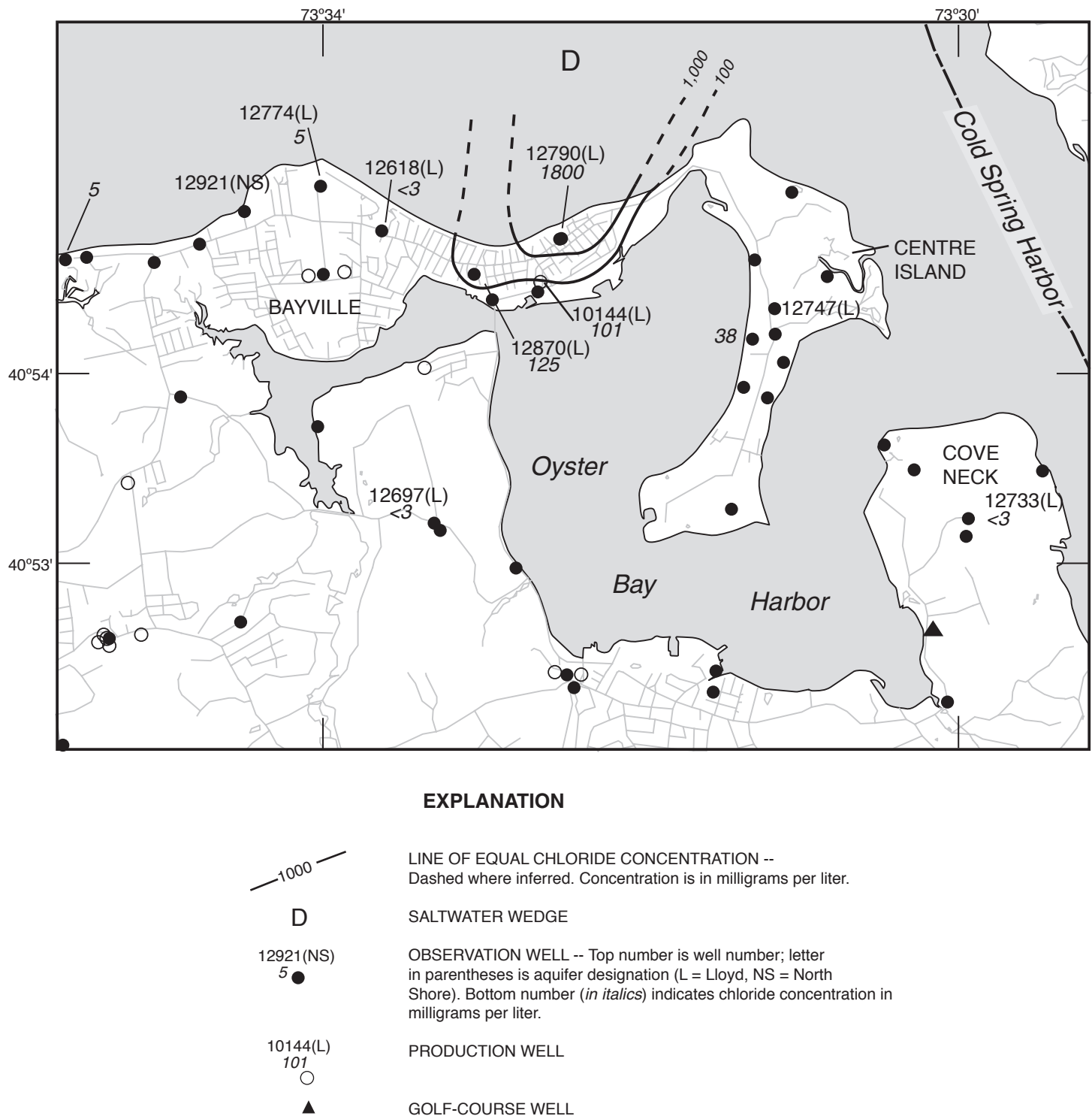
FIGURE 17B. Chloride concentrations in the Lloyd and North Shore aquifers, Oyster Bay study area, Nassau County, N.Y., 1997. (Location is shown in fig. 17A.)
