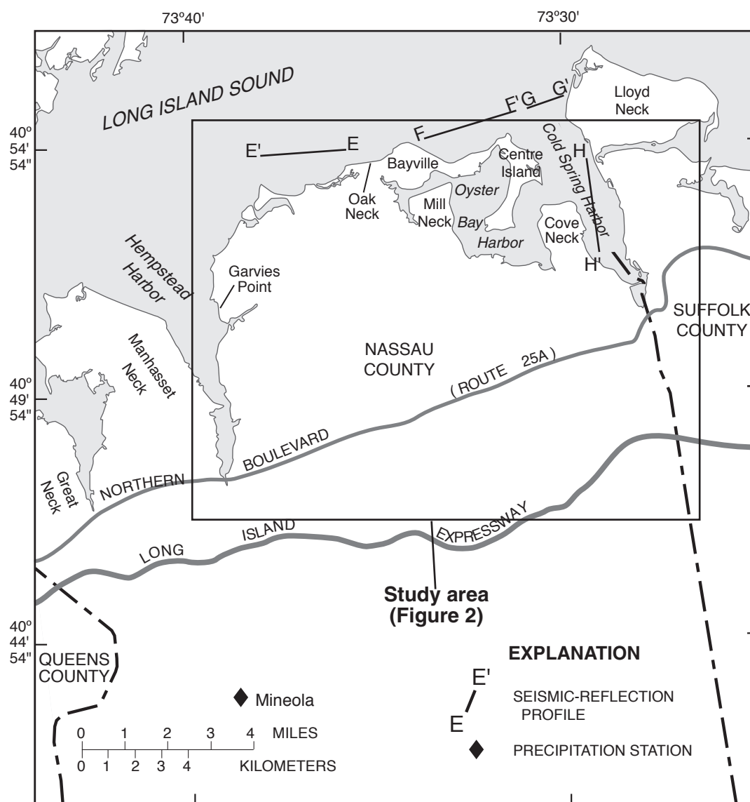
FIGURE 1. Location of Oyster Bay study area and marine-seismic-reflection profiles, Nassau County, N.Y.
